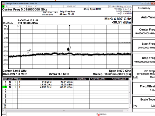
Band26-Part90s_3MHz_QPSK_RB1_0_CH26775
