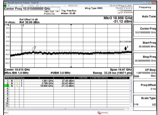
Band25_5MHz_QPSK_RB1_0_CH26665
