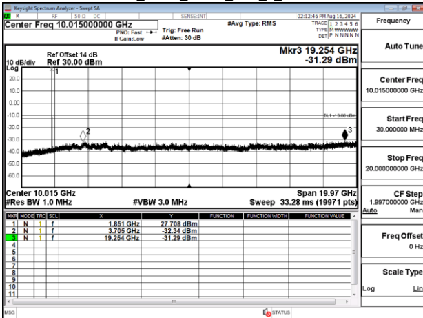
Band25_5MHz_QPSK_RB1_0_CH26065
