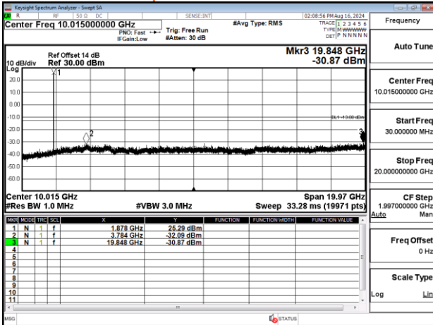
Band25_10MHz_QPSK_RB1_0_CH26640
