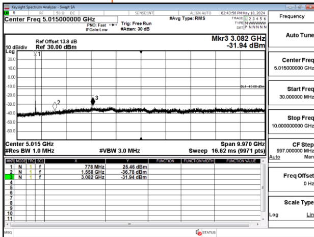
Band13_5MHz_QPSK_RB1_0_CH23230
