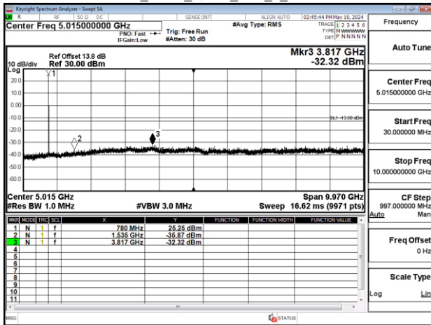
Band13_5MHz_QPSK_RB1_0_CH23255
