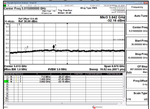
Band12_3MHz_QPSK_RB1_0_CH23165
