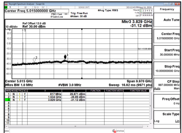
Band26-Part90s_5MHz_QPSK_RB1_0_CH26765
