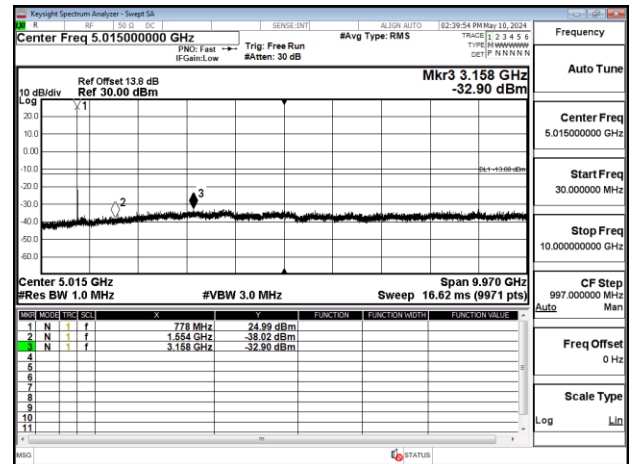
Band14_5MHz_QPSK_RB1_0_CH23305
