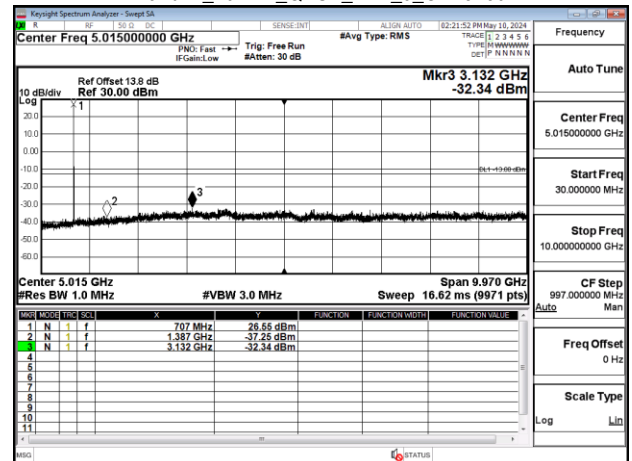
Band12_10MHz_QPSK_RB1_0_CH23130
