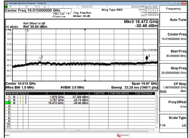
Band25_15MHz_QPSK_RB1_0_CH26615
