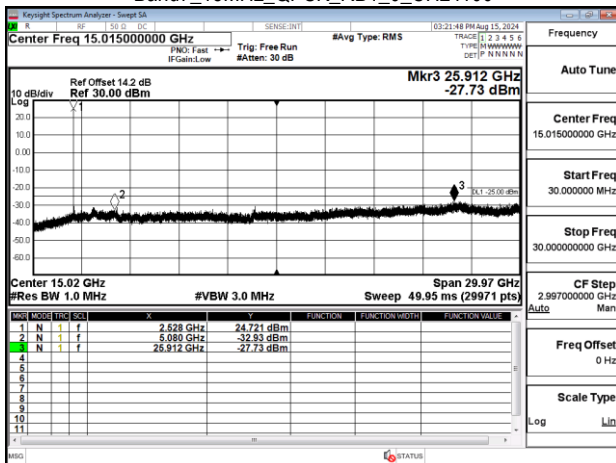
Band7_15MHz_QPSK_RB1_0_CH21375
