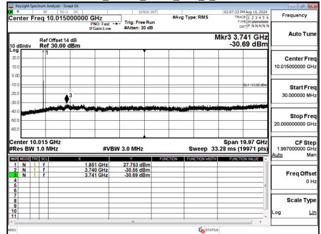
Band25_10MHz_QPSK_RB1_0_CH26090
