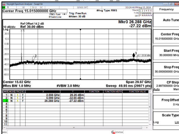
Band7_15MHz_QPSK_RB1_0_CH21375
