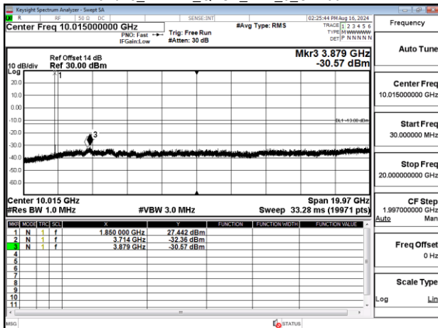
Band25_1.4MHz_QPSK_RB1_0_CH26047
