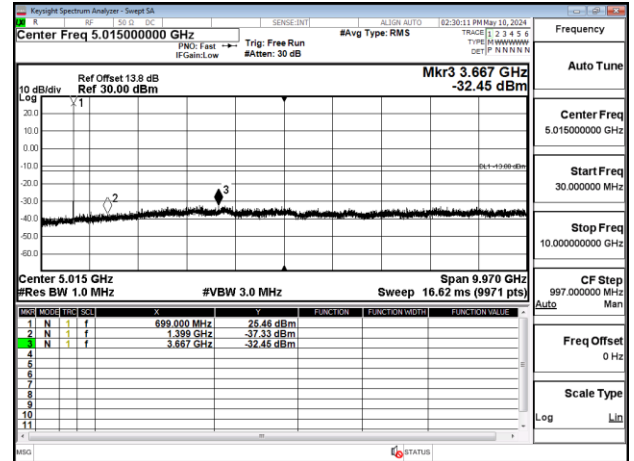
Band12_3MHz_QPSK_RB1_0_CH23095
