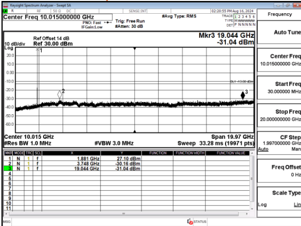
Band25_3MHz_QPSK_RB1_0_CH26675
