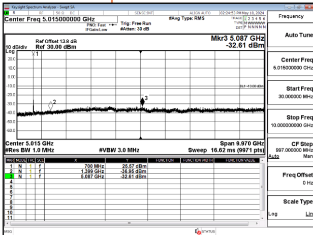
Band12_5MHz_QPSK_RB1_0_CH23095
