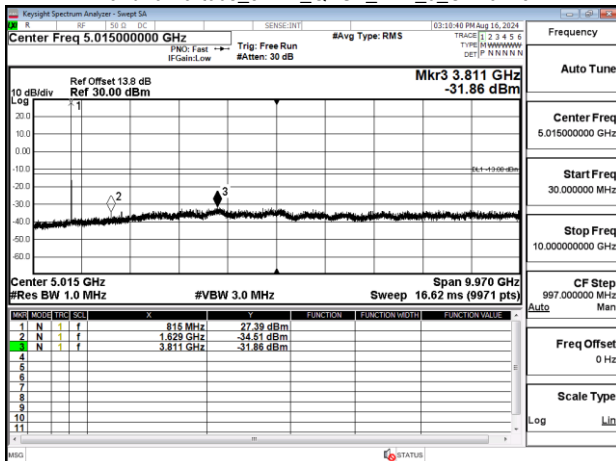
Band26-Part90s_5MHz_QPSK_RB1_0_CH26715
