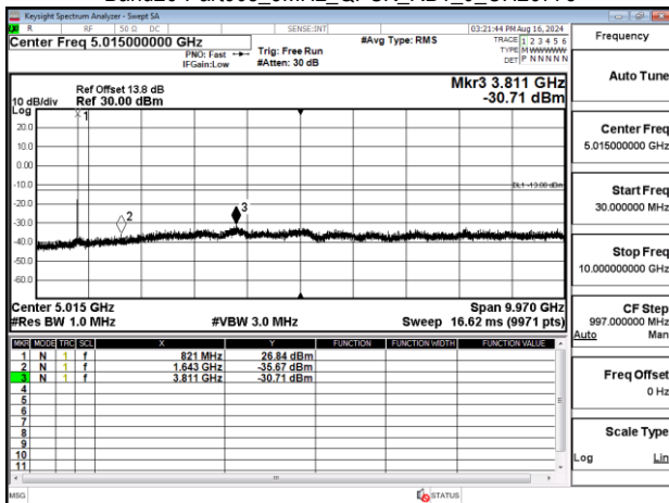
Band26-Part90s_5MHz_QPSK_RB1_0_CH26715
