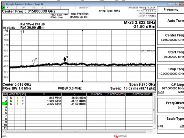
Band26_1.4MHz_QPSK_RB1_0_CH27033
