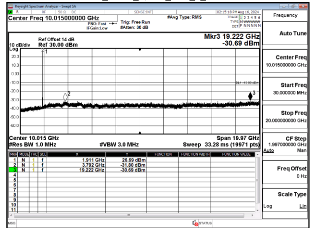
Band25_10MHz_QPSK_RB1_0_CH26090
