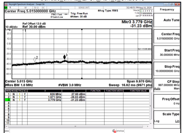
Band26_3MHz_QPSK_RB1_0_CH27025
