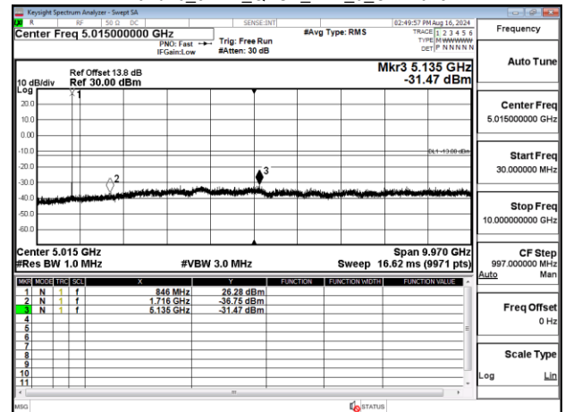
Band26_3MHz_QPSK_RB1_0_CH27025
