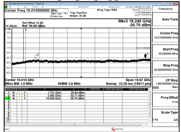
Band4_3MHz_QPSK_RB1_0_CH20385
