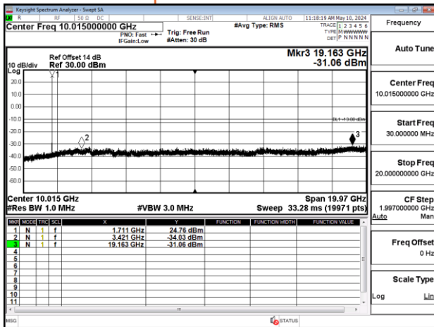
Band4_5MHz_QPSK_RB1_0_CH20175
