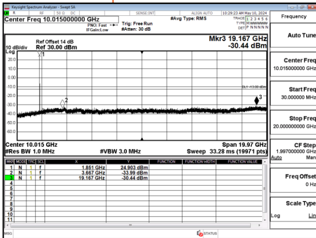
Band2_5MHz_QPSK_RB1_0_CH18900
