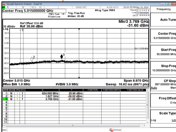
Band5_1.4MHz_QPSK_RB1_0_CH20525
