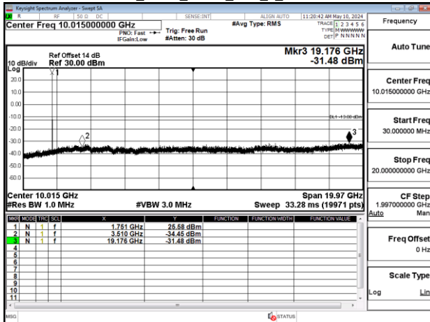
Band4_5MHz_QPSK_RB1_0_CH20375
