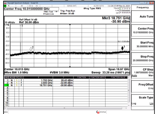
Band4_3MHz_QPSK_RB1_0_CH20385
