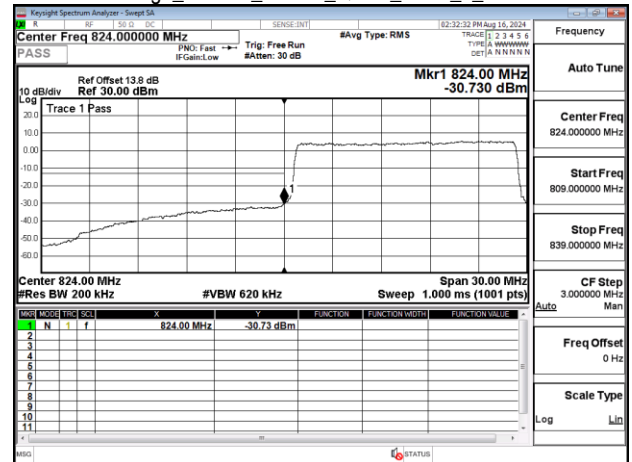
Band Edge_Band26_15MHz_QPSK_RB75_0_CH26865
