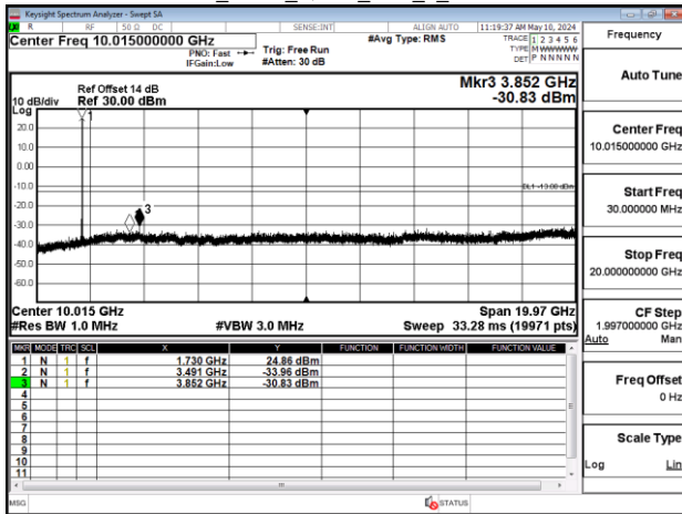
Band4_5MHz_QPSK_RB1_0_CH20375
