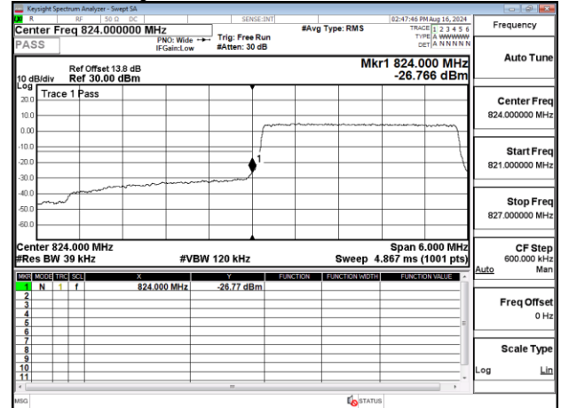
Band Edge_Band26_3MHz_QPSK_RB15_0_CH26805
