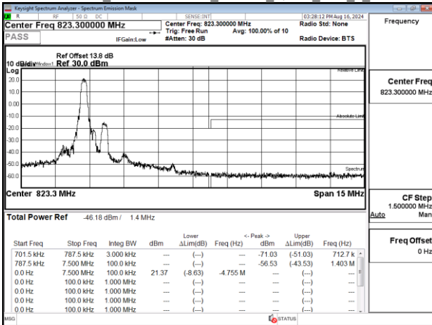
Emission Mask_Band26-Part90s_1.4MHz_QPSK_RB1_0_CH26783
