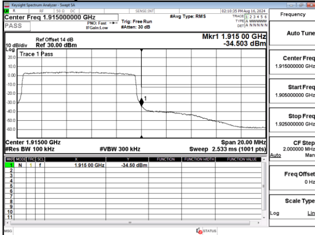
Band Edge_Band25_10MHz_QPSK_RB50_0_CH26640
