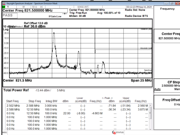
Emission Mask_Band26-Part90s_5MHz_QPSK_RB1_0_CH26765
