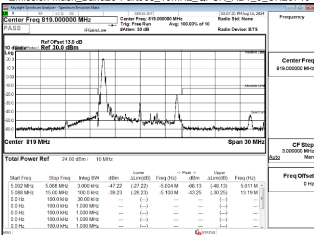
Emission Mask_Band26-Part90s_10MHz_QPSK_RB1_0_CH26740
