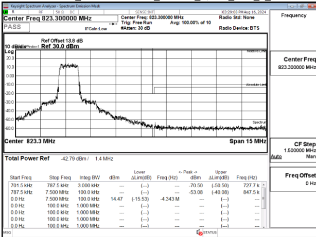
Emission Mask_Band26-Part90s_1.4MHz_QPSK_RB6_0_CH26783
