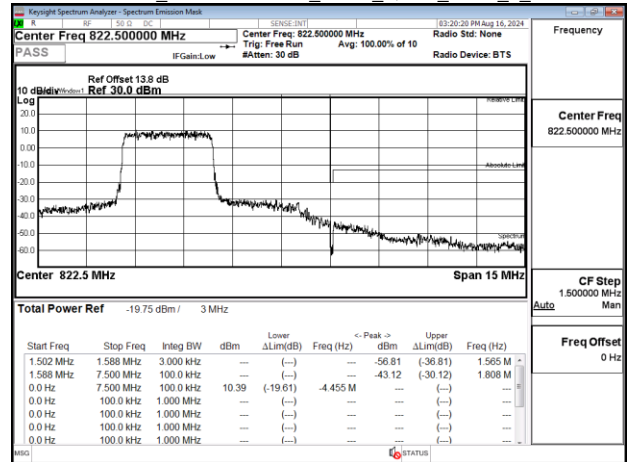
Emission Mask_Band26-Part90s_3MHz_QPSK_RB15_0_CH26775
