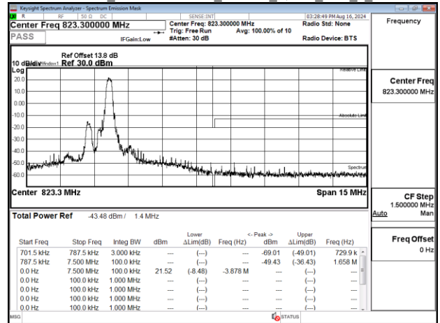
Emission Mask_Band26-Part90s_1.4MHz_QPSK_RB1_5_CH26783
