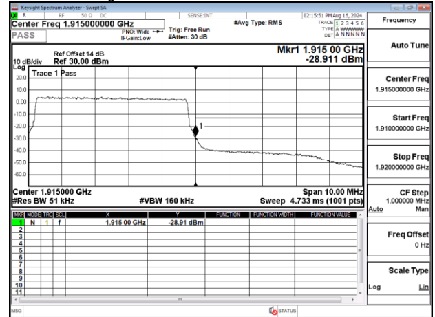
Band Edge_Band25_10MHz_QPSK_RB1_0_CH26090
