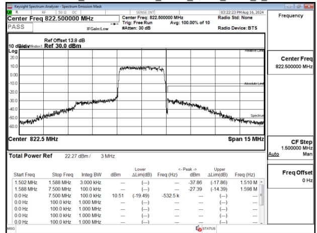
Emission Mask_Band26-Part90s_5MHz_QPSK_RB1_0_CH26715
