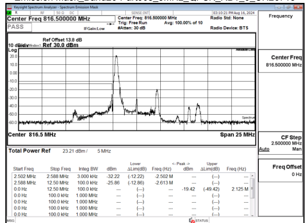
Emission Mask_Band26-Part90s_5MHz_QPSK_RB1_0_CH26715
