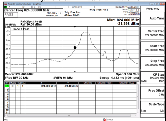
Band Edge_Band26_1.4MHz_QPSK_RB1_0_CH26797
