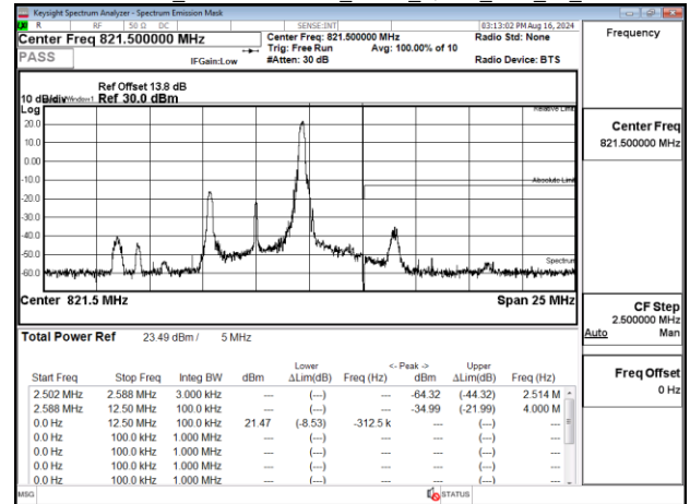
Emission Mask_Band26-Part90s_5MHz_QPSK_RB1_24_CH26765
