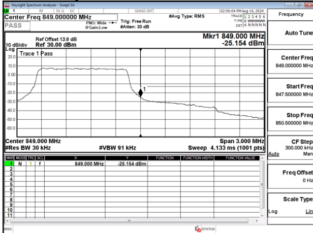
Band Edge_Band26_1.4MHz_QPSK_RB6_0_CH27033
