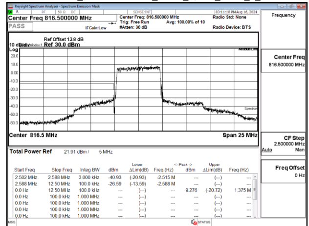
Emission Mask_Band26-Part90s_5MHz_QPSK_RB25_0_CH26715
