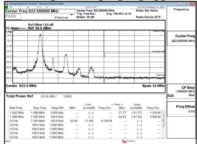
Emission Mask_Band26-Part90s_3MHz_QPSK_RB1_0_CH26775
