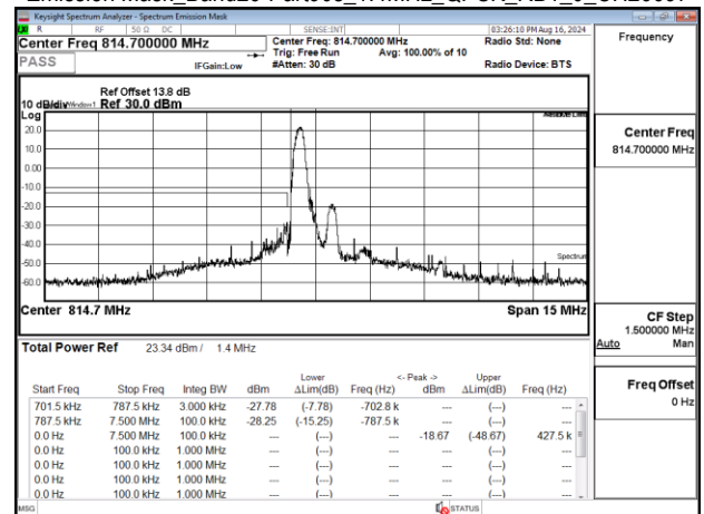
Emission Mask_Band26-Part90s_1.4MHz_QPSK_RB1_0_CH26697
