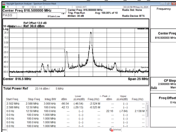
Emission Mask_Band26-Part90s_5MHz_QPSK_RB1_24_CH26715
