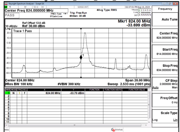
Band Edge_Band26_10MHz_QPSK_RB1_0_CH26840
