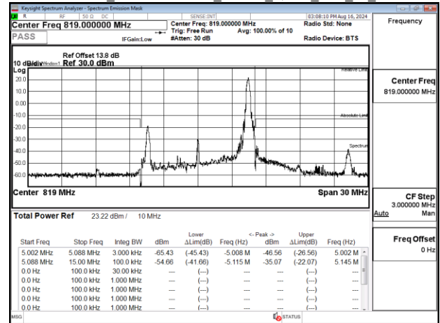
Emission Mask_Band26-Part90s_10MHz_QPSK_RB50_0_CH26740
