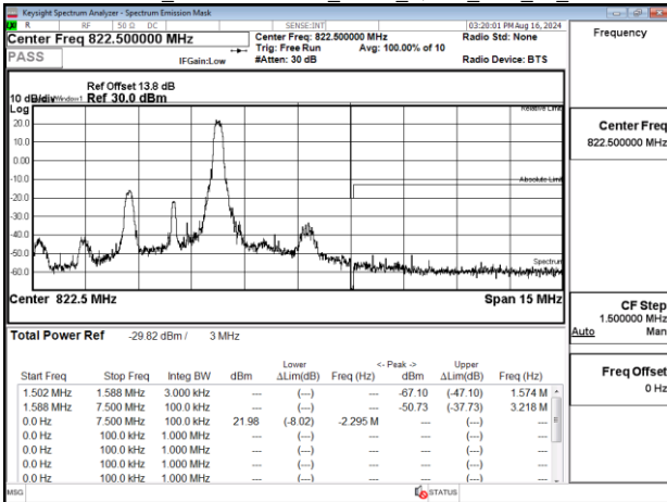
Emission Mask_Band26-Part90s_3MHz_QPSK_RB1_14_CH26775
