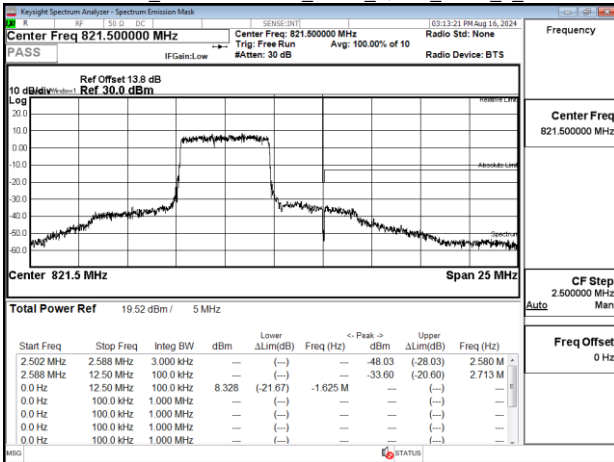
Emission Mask_Band26-Part90s_5MHz_QPSK_RB25_0_CH26765
