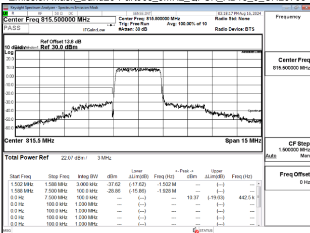
Emission Mask_Band26-Part90s_3MHz_QPSK_RB15_0_CH26705
