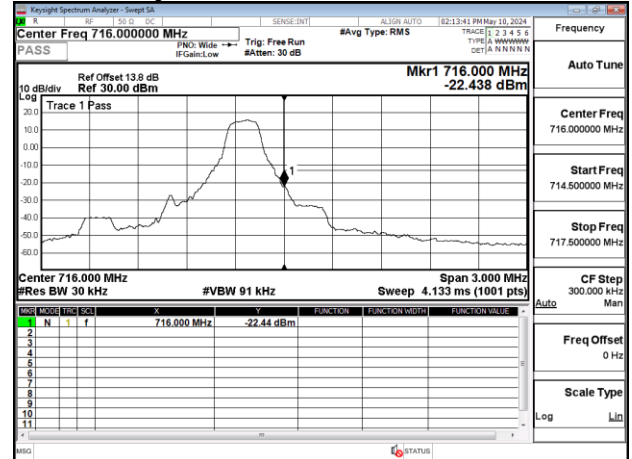
Band Edge_Band12_1.4MHz_QPSK_RB1_5_CH23173
