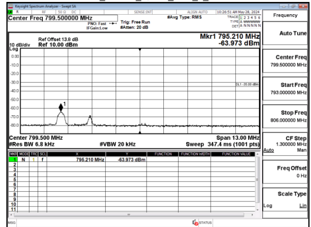
Emission Mask_Band14_5MHz_QPSK_RB1_0_CH23305
