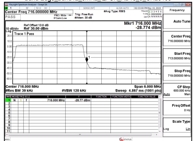
Band Edge_Band12_3MHz_QPSK_RB15_0_CH23165
