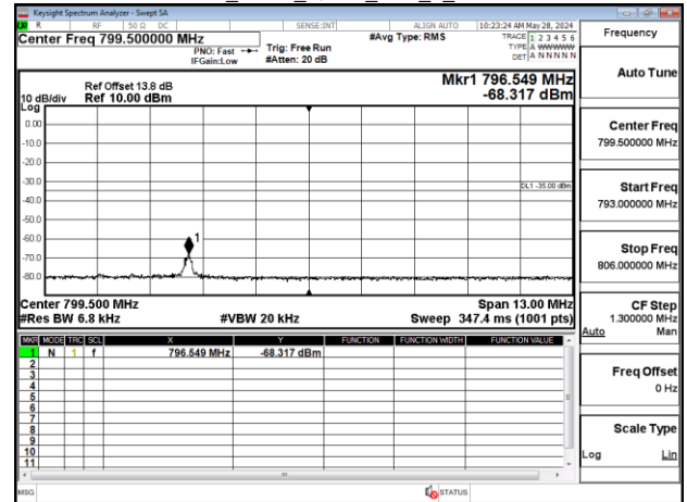
Band13_5MHz_QPSK_RB1_0_CH23230
