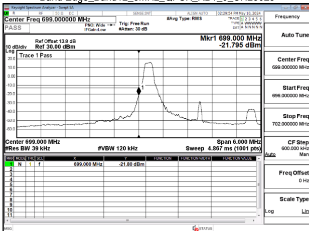
Band Edge_Band12_3MHz_QPSK_RB1_0_CH23025
