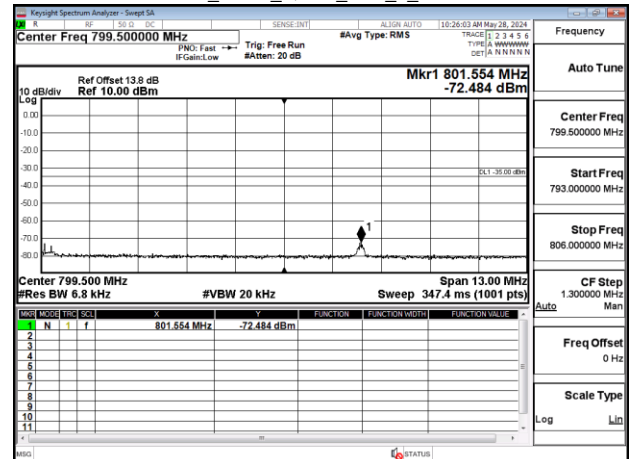
Band13_5MHz_QPSK_RB1_0_CH23255
