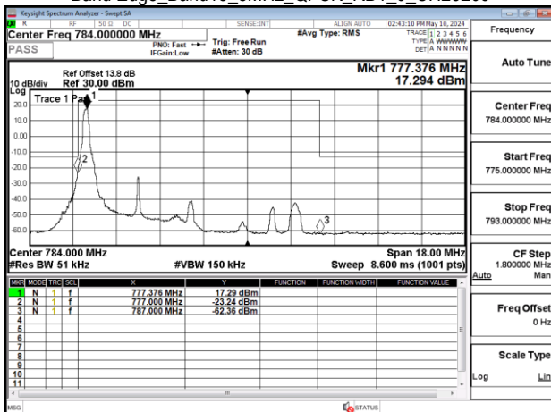
Band Edge_Band13_5MHz_QPSK_RB1_0_CH23205
