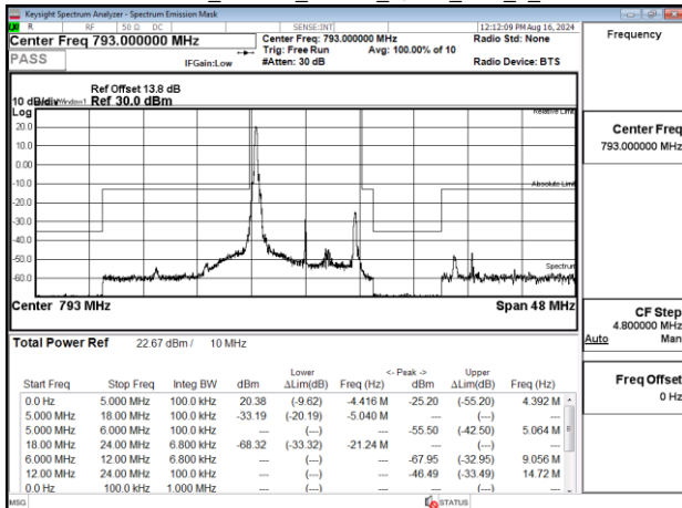
Emission Mask_Band14_10MHz_QPSK_RB1_0_CH23330
