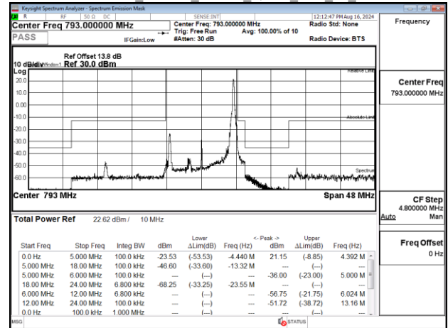
Emission Mask Band14_10MHz_QPSK_RB50_0_CH23330
