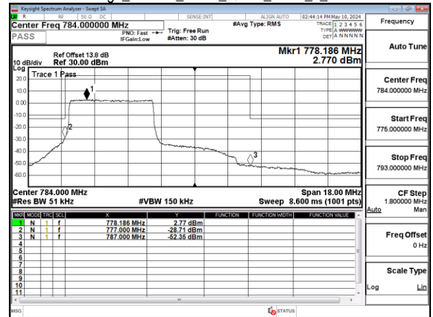
Band Edge_Band13_5MHz_QPSK_RB25_0_CH23255
