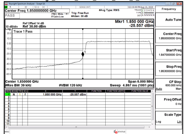
Band Edge_Band25_3MHz_QPSK_RB15_0_CH26055
