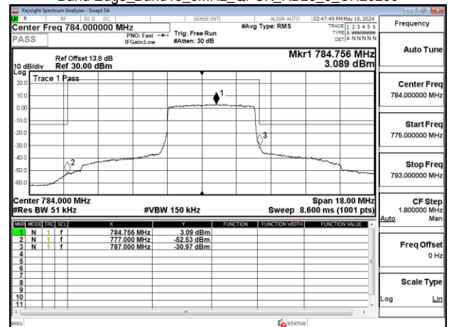
Band Edge_Band13_5MHz_QPSK_RB25_0_CH23255
