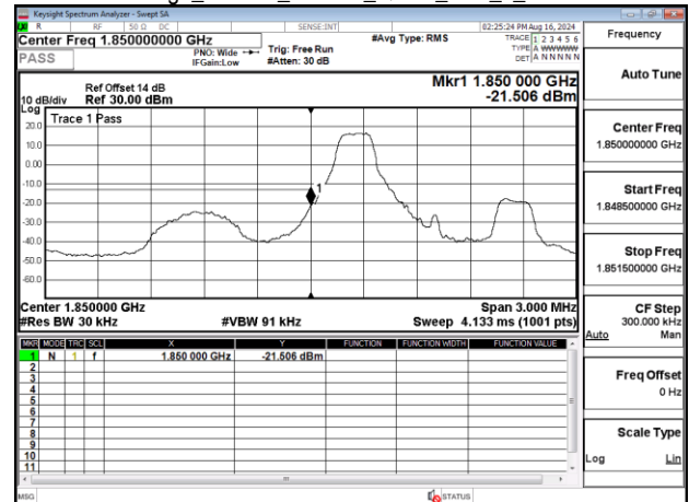
Band Edge_Band25_1.4MHz_QPSK_RB1_0_CH26047
