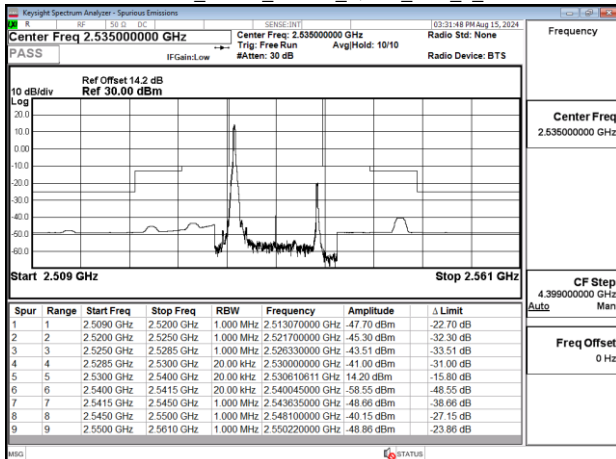
Emission Mask_Band7_10MHz_QPSK_RB1_0_CH21100
