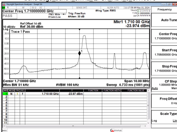
Band Edge_Band4_5MHz_QPSK_RB1_0_CH19975
