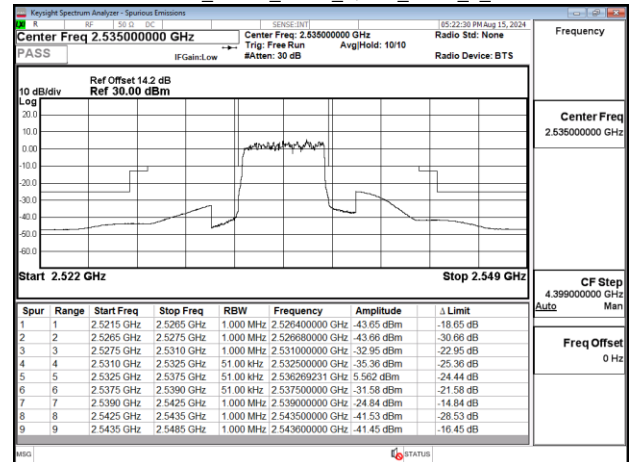
Emission Mask_Band7_5MHz_QPSK_RB25_0_CH21100
