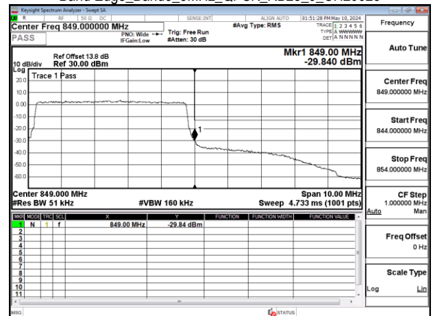
Band Edge_Band5_5MHz_QPSK_RB25_0_CH20625
