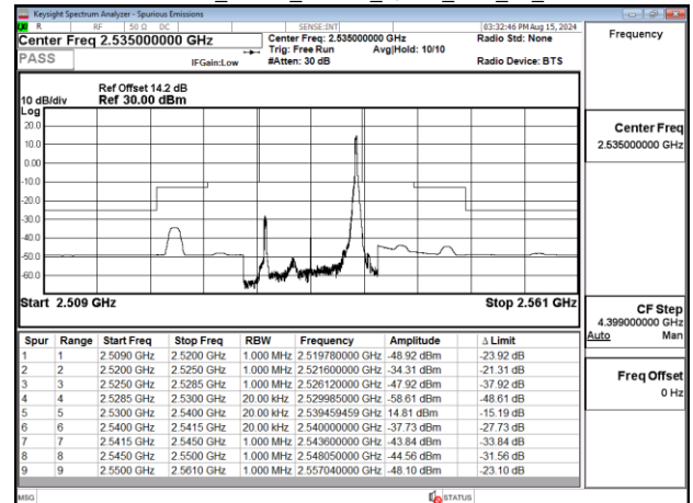
Emission Mask_Band7_10MHz_QPSK_RB1_49_CH21100
