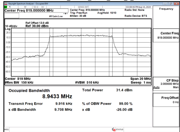
Band26-Part90s_10MHz_16QAM_RB50_0_CH26740
