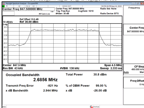
Band26_3MHz_QPSK_RB15_0_CH27025
