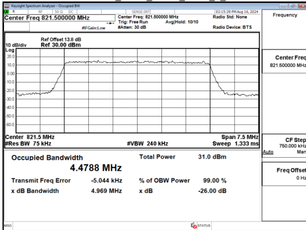
Band26-Part90s_5MHz_16QAM_RB25_0_CH26715
