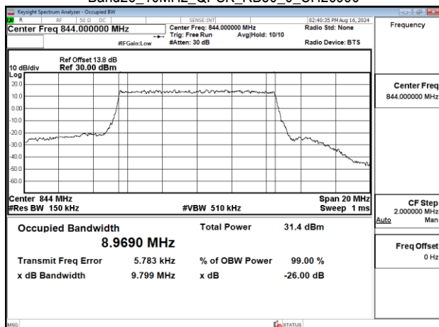
Band26_10MHz_QPSK_RB50_0_CH26990
