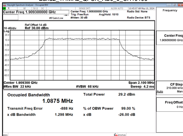
Band2_1.4MHz_QPSK_RB6_0_CH19193
