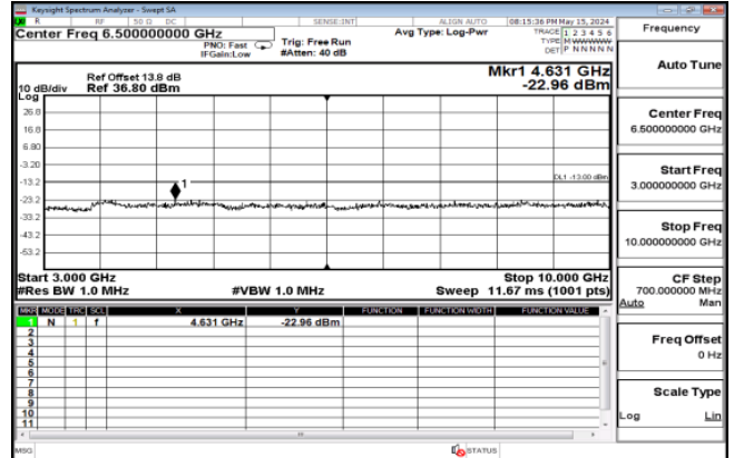
WCDMA_B5_MidCH4183-836.6
