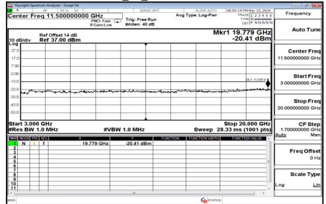
HSUPA_B2_HighCH9538-1907.6
