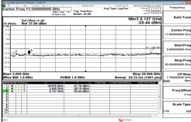
HSUPA_B4_MidCH1413-1732.6
