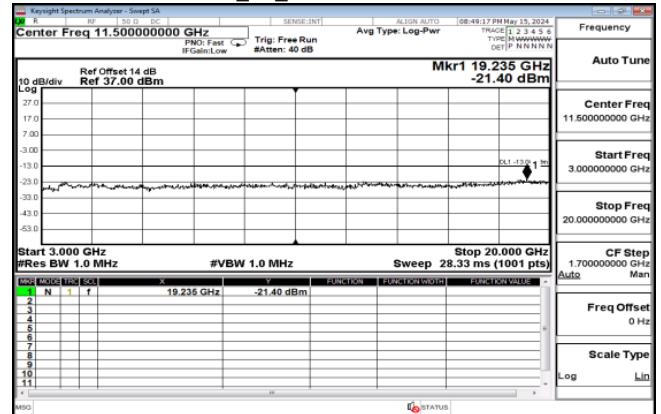
HSUPA_B2_MidCH9400-1880
