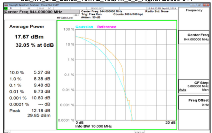
Cat_M1_LTE_Band5_10MHz_16QAM_6_0_HighCH20600-844
