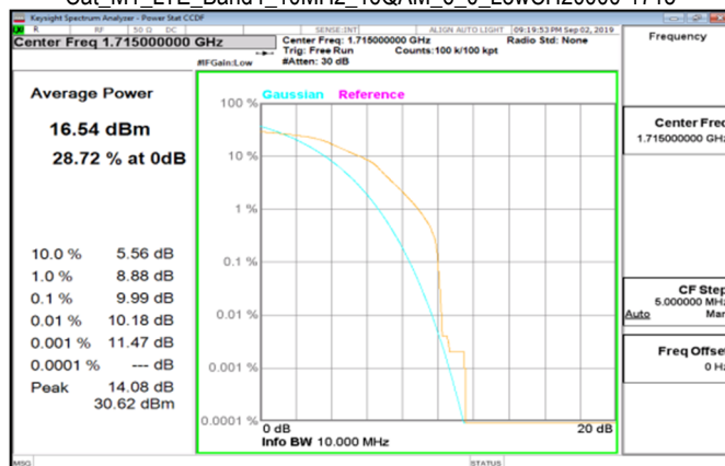
Cat M1_LTE_Band4_10MHz_16QAM_6_0_LowCH20000-1715
