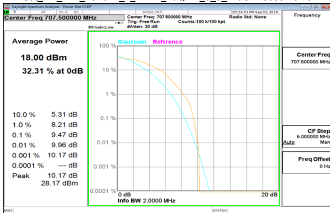
Cat M1 LTE_Band12_1_4MHz_16QAM_6_0_MidCH23095-707.5
