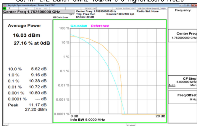
Cat M1_LTE_Band4_5MHz_16QAM_6_0_HighCH20375-1752.5
