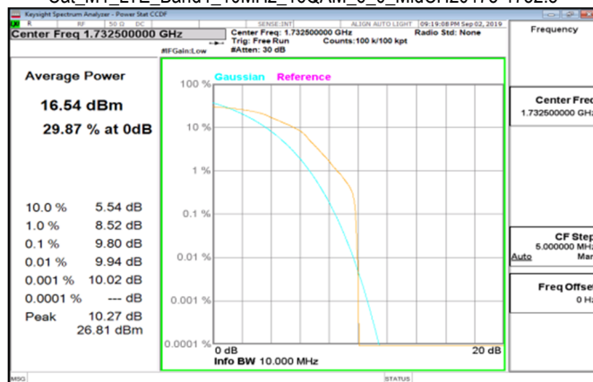
Cat M1_LTE_Band4_10MHz_16QAM_6_0_MidCH20175-1732.5
