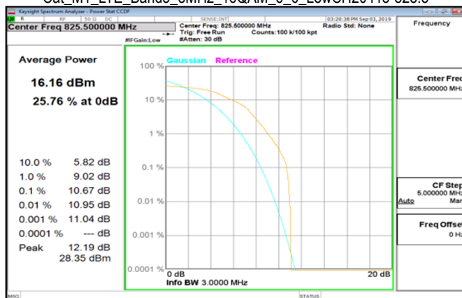
Cat M1 LTE Band5_3MHz_16QAM_6_0_LowCH20415-825.5
