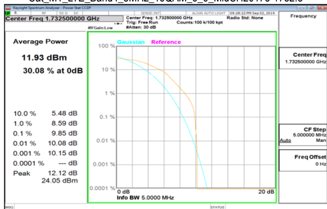
Cat M1_LTE_Band4_5MHz_16QAM_6_0_MidCH20175-1732.5
