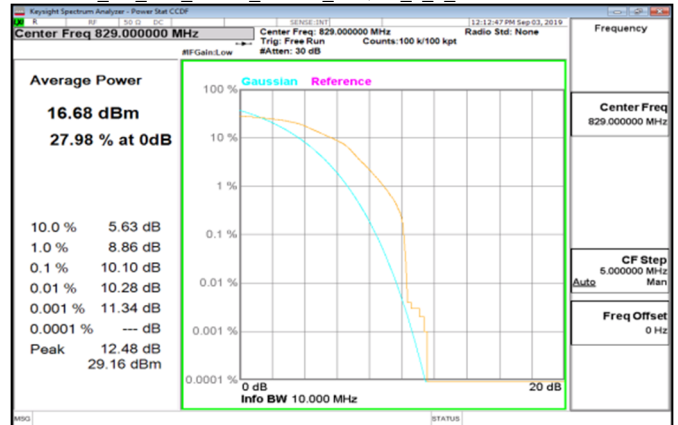
Cat_M1_LTE_Band5_10MHz_16QAM_6_0_LowCH20450-829
