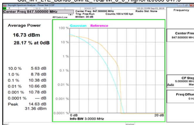
Cat M1 LTE Band5_3MHz_16QAM_6_0_HighCH20635-847.5
