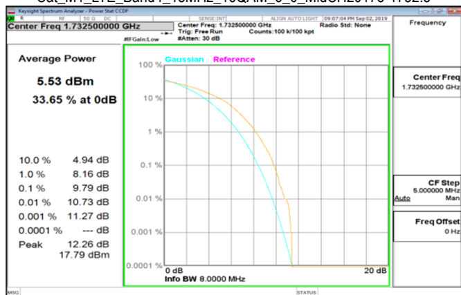
Cat_M1_LTE_Band4_15MHz_16QAM_6_0_MidCH20175-1732.5
