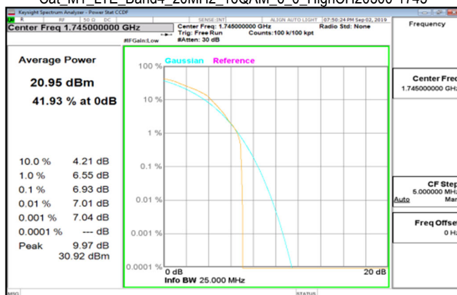
Cat_M1_LTE_Band4_20MHz_16QAM_6_0_HighCH20300-1745
