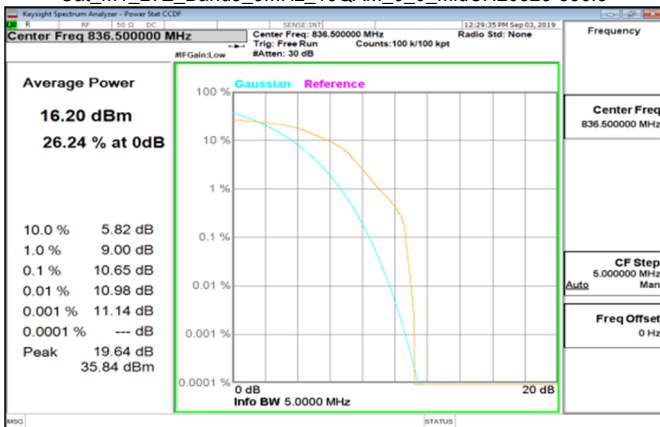
Cat_M1_LTE_Band5_5MHz_16QAM_6_0_MidCH20525-836.5
