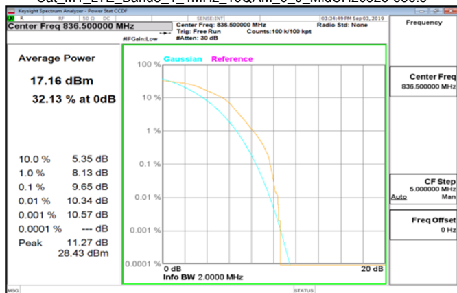
Cat M1 LTE Band5_1_4MHz_16QAM_6_0_MidCH20525-836.5
