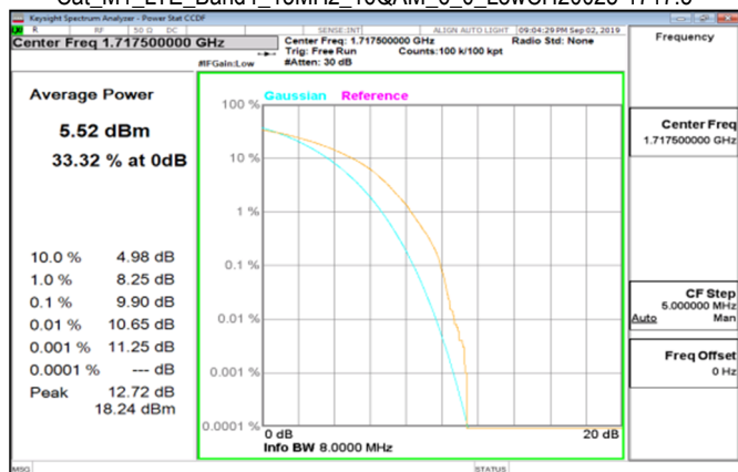
Cat_M1_LTE_Band4_15MHz_16QAM_6_0_LowCH20025-1717.5
