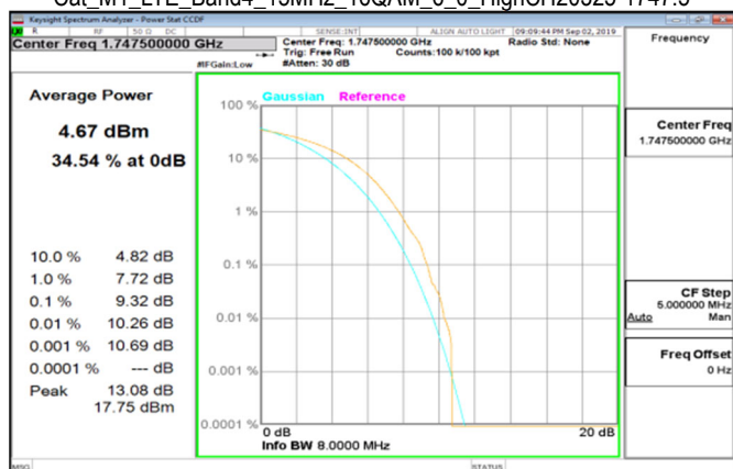
Cat_M1_LTE_Band4_15MHz_16QAM_6_0_HighCH20325-1747.5
