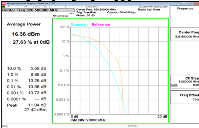
Cat_M1_LTE_Band5_5MHz_16QAM_6_0_LowCH20425-826.5
