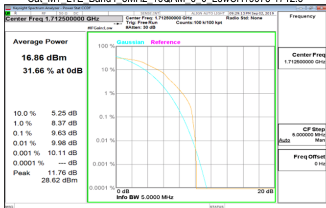
Cat M1_LTE_Band4_5MHz_16QAM_6_0_LowCH19975-1712.5
