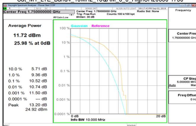
Cat M1_LTE_Band4_10MHz_16QAM_6_0_HighCH20350-1750
