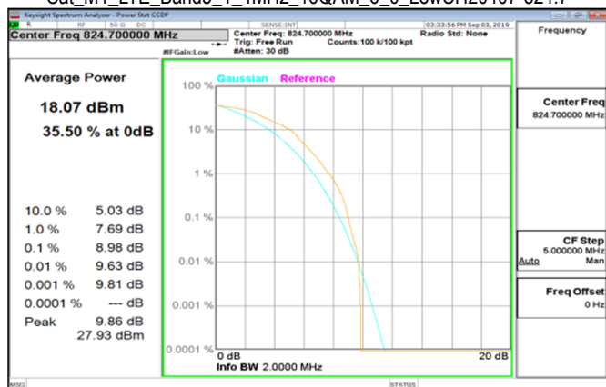
Cat M1 LTE Band5_1_4MHz_16QAM_6_0_LowCH20407-824.7
