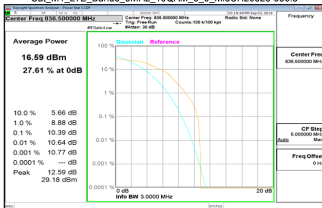
Cat M1 LTE Band5_3MHz_16QAM_6_0_MidCH20525-836.5
