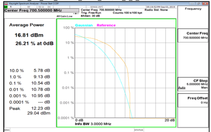
Cat M1 LTE_Band12_3MHz_16QAM_6_0_LowCH23025-700.5
