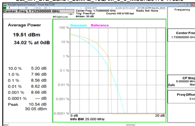
Cat_M1_LTE_Band4_20MHz_16QAM_6_0_MidCH20175-1732.5
