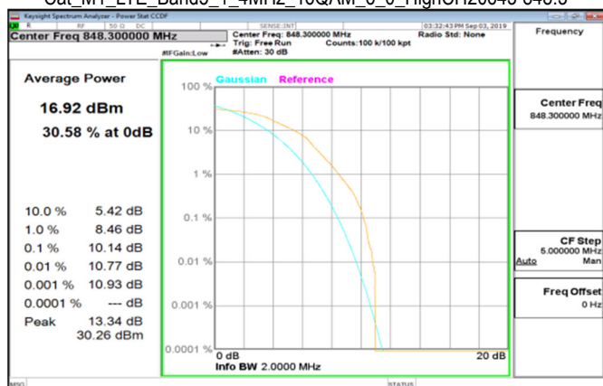
Cat M1 LTE Band5_1_4MHz_16QAM_6_0_HighCH20643-848.3
