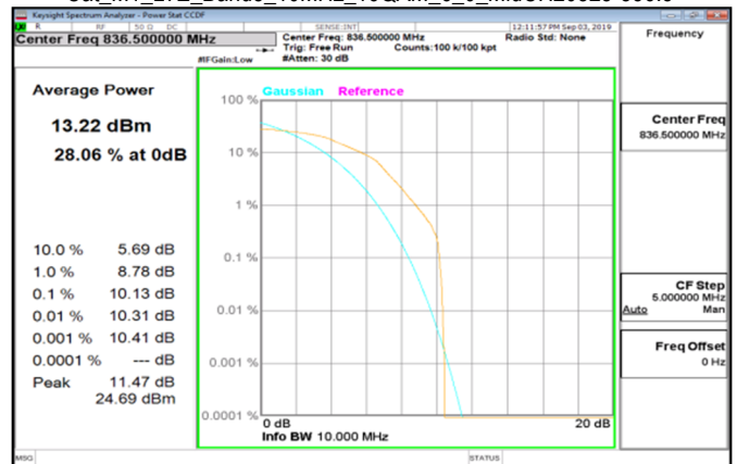
Cat_M1_LTE_Band5_10MHz_16QAM_6_0_MidCH20525-836.5
