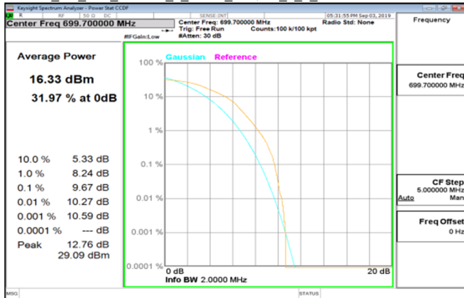
Cat M1 LTE_Band12_1_4MHz_16QAM_6_0_LowCH23017-699.7
