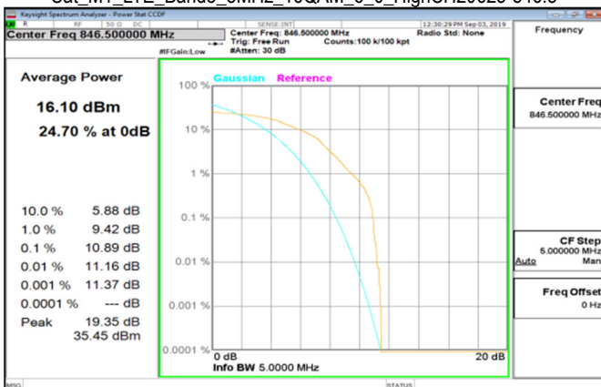
Cat_M1_LTE_Band5_5MHz_16QAM_6_0_HighCH20625-846.5
