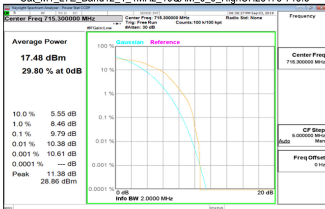
Cat M1 LTE_Band12_1_4MHz_16QAM_6_0_HighCH23173-715.3
