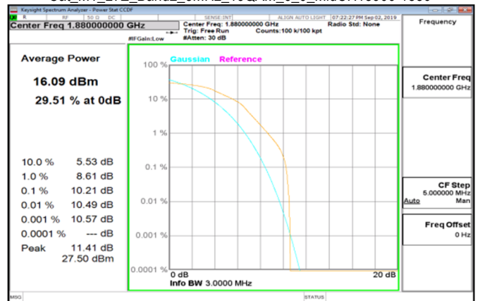
Cat M1 LTE_Band2_3MHz_16QAM_6_0_MidCH18900-1880
