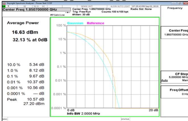
Cat M1 LTE_Band2_1_4MHz_16QAM_6_0_LowCH18607-1850.7
