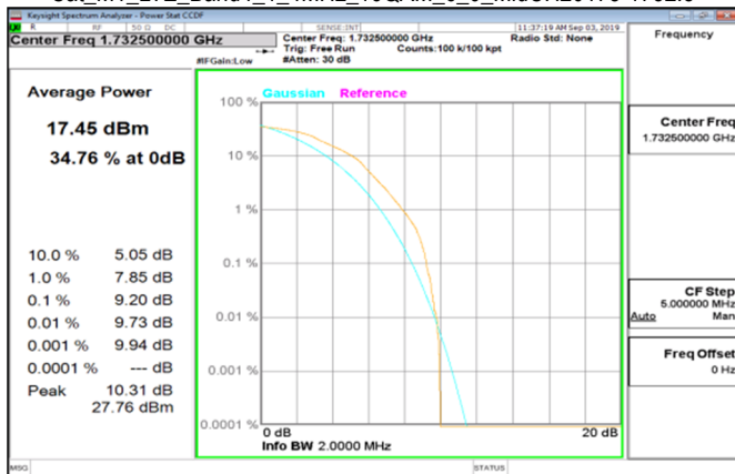
Cat M1 LTE_Band4_1_4MHz_16QAM_6_0_MidCH20175-1732.5
