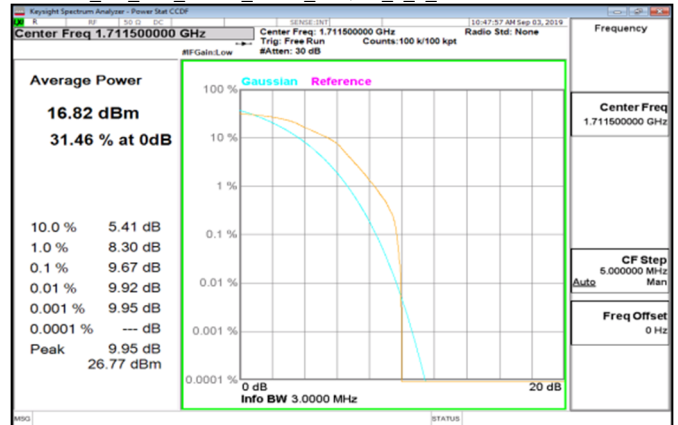
Cat M1 LTE_Band4_3MHz_16QAM_6_0_LowCH19965-1711.5
