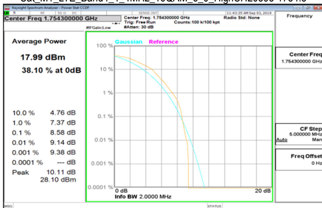
Cat M1 LTE_Band4_1_4MHz_16QAM_6_0_HighCH20393-1754.3
