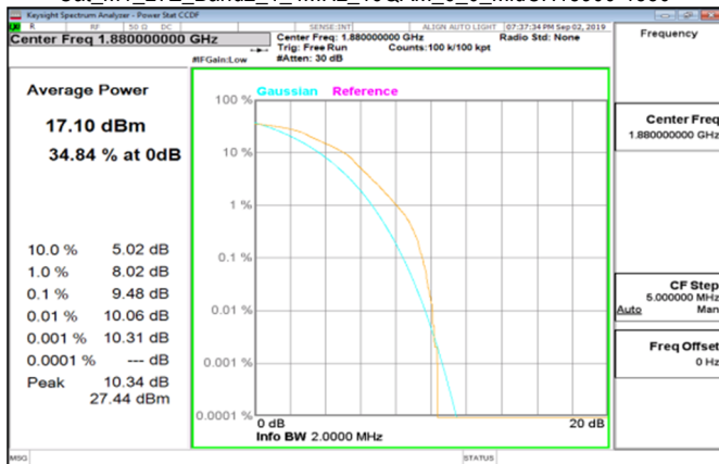
Cat M1 LTE_Band2_1_4MHz_16QAM_6_0_MidCH18900-1880
