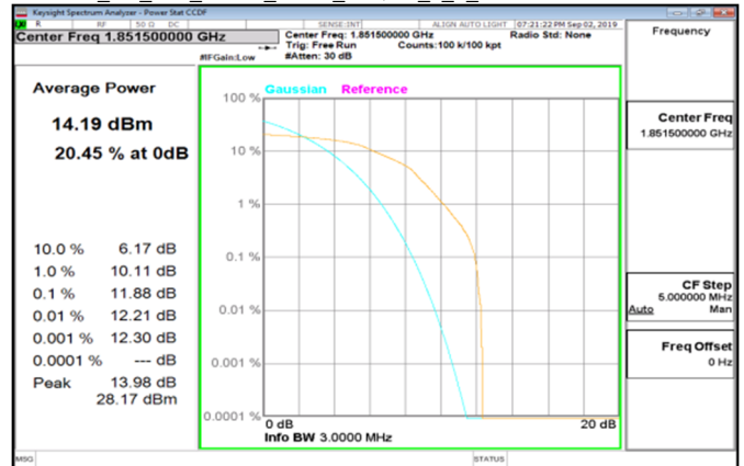
Cat M1 LTE_Band2_3MHz_16QAM_6_0_LowCH18615-1851.5
