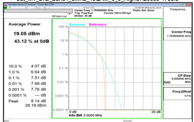
Cat M1 LTE_Band4_3MHz_16QAM_6_0_HighCH20385-1753.5
