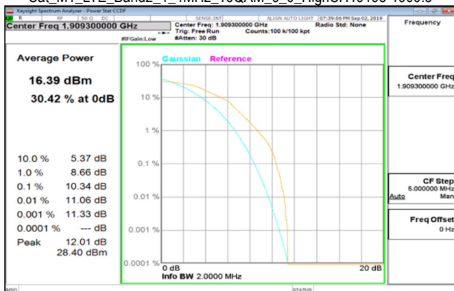
Cat M1 LTE_Band2_1_4MHz_16QAM_6_0_HighCH19193-1909.3
