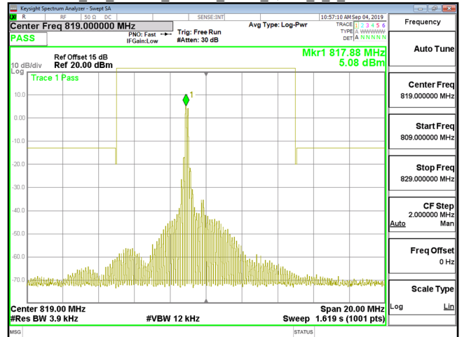
Cat_M1_Band26_Part90s_3MHz_QPSK_1_0_CH26740
