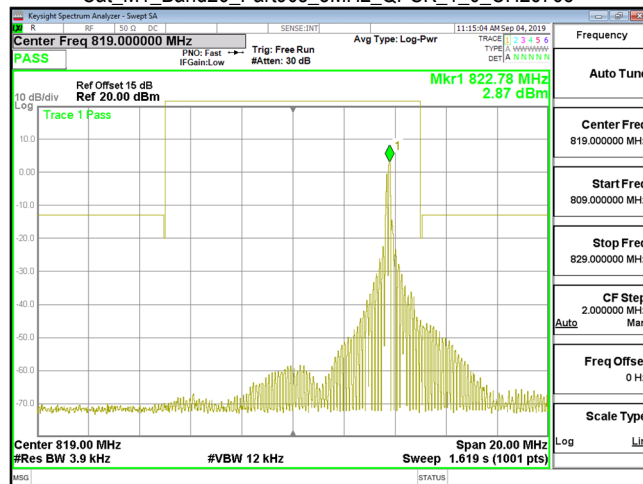
Cat M1_Band26_Part90s_5MHz_QPSK_1_0_CH26765
