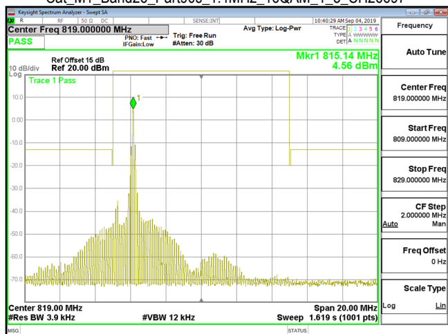
Cat_M1_Band26_Part90s_1.4MHz_16QAM_1_5_CH26697
