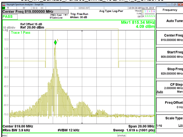
Cat M1_Band26_Part90s_3MHz_16QAM_1_5_CH26705
