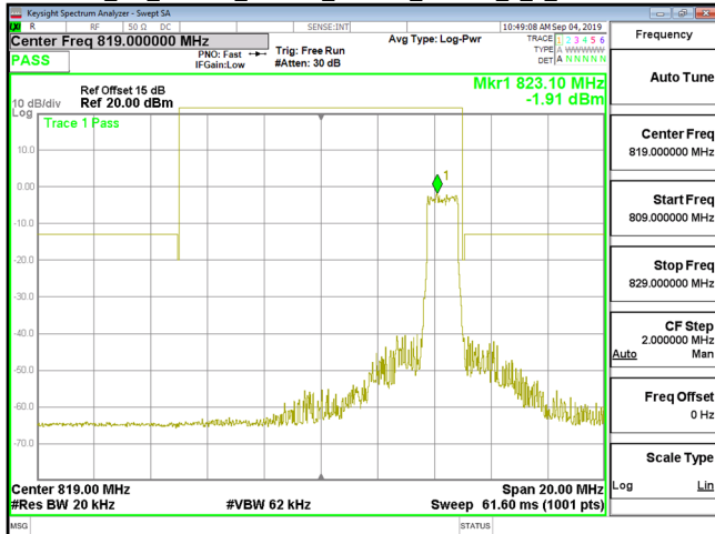
Cat_M1_Band26_Part90s_1.4MHz_16QAM_6_0_CH26783
