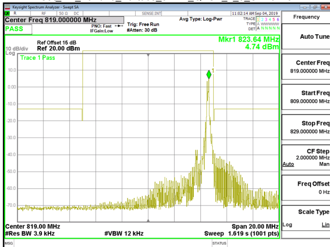
Cat_M1_Band26_Part90s_3MHz_QPSK_1_5_CH26775
