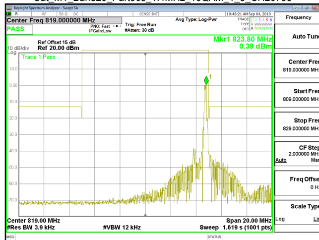
Cat_M1_Band26_Part90s_1.4MHz_16QAM_1_5_CH26783
