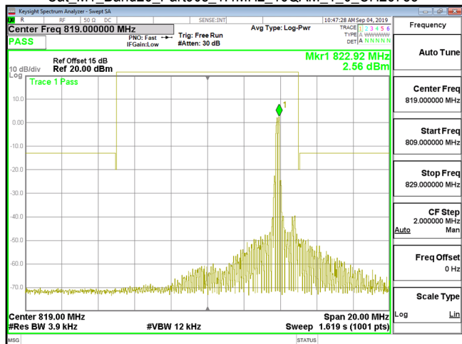
Cat_M1_Band26_Part90s_1.4MHz_16QAM_1_0_CH26783
