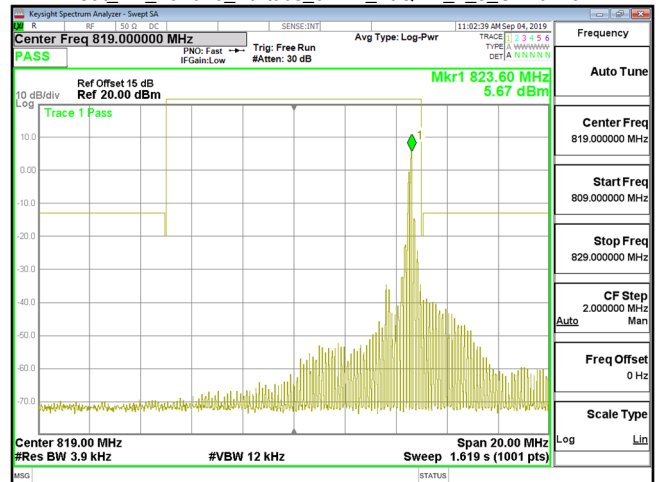
Cat M1_Band26_Part90s_3MHz_16QAM_1_5_CH26775
