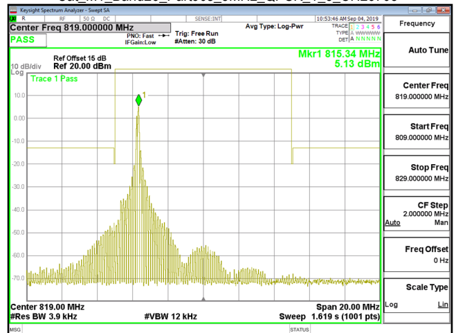
Cat_M1_Band26_Part90s_3MHz_QPSK_1_5_CH26705
