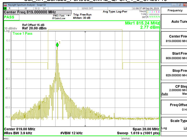
Cat M1_Band26_Part90s_5MHz_QPSK_1_5_CH26715
