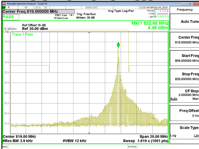
Cat M1_Band26_Part90s_3MHz_16QAM_1_0_CH26775
