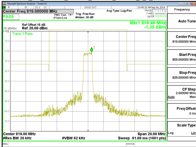
Cat_M1_Band26_Part90s_1.4MHz_16QAM_6_0_CH26740
