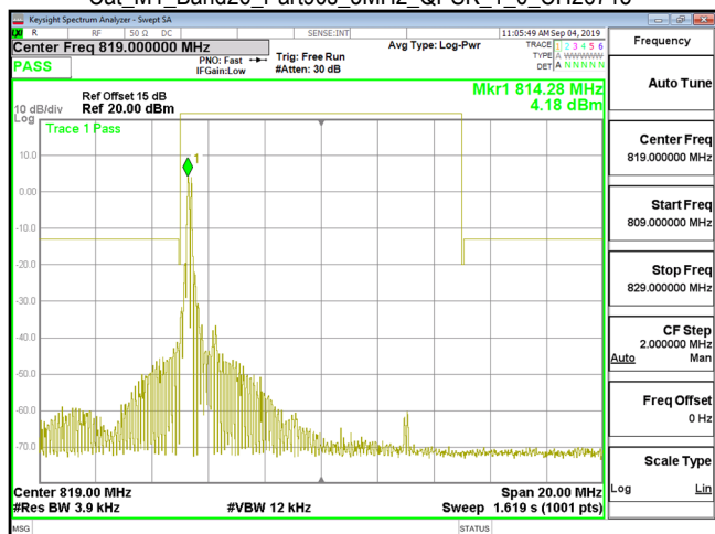
Cat M1_Band26_Part90s_5MHz_QPSK_1_0_CH26715
