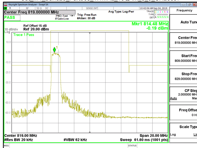
Cat_M1_Band26_Part90s_1.4MHz_16QAM_6_0_CH26697
