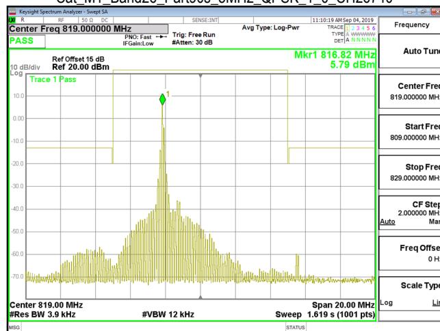
Cat M1_Band26_Part90s_5MHz_QPSK_1_0_CH26740
