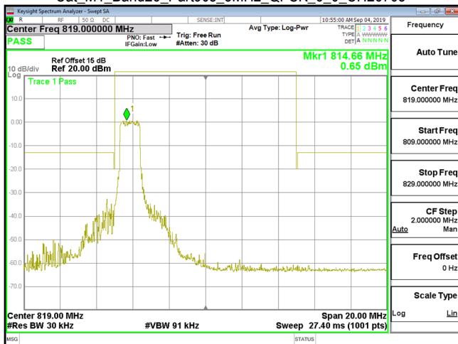
Cat_M1_Band26_Part90s_3MHz_QPSK_6_0_CH26705
