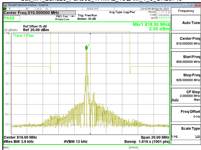
Cat_M1_Band26_Part90s_1.4MHz_16QAM_1_0_CH26740
