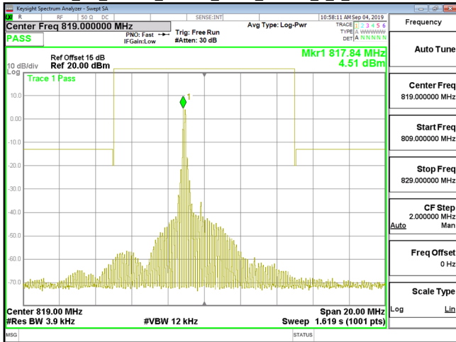
Cat M1_Band26_Part90s_3MHz_16QAM_1_0_CH26740
