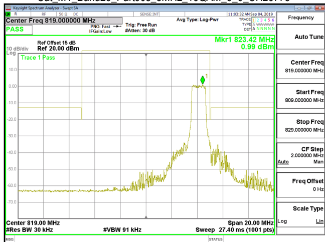
Cat M1_Band26_Part90s_3MHz_16QAM_6_0_CH26775
