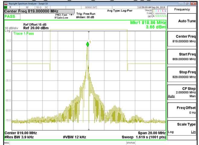
Cat M1_Band26_Part90s_3MHz_16QAM_1_5_CH26740
