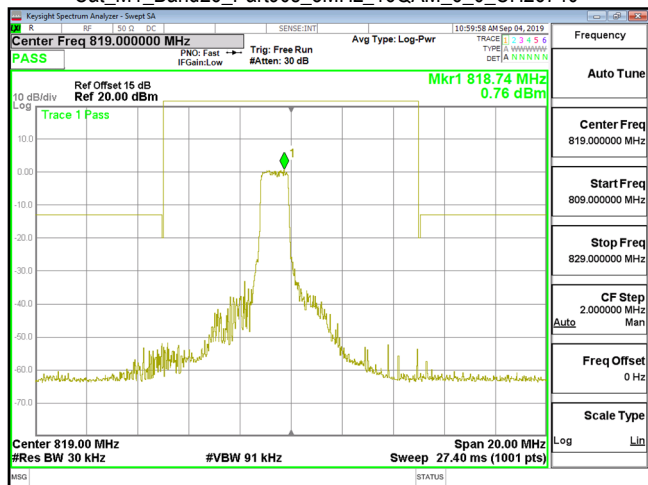
Cat M1_Band26_Part90s_3MHz_16QAM_6_0_CH26740
