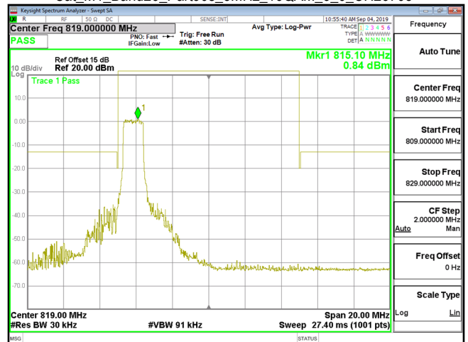
Cat M1_Band26_Part90s_3MHz_16QAM_6_0_CH26705
