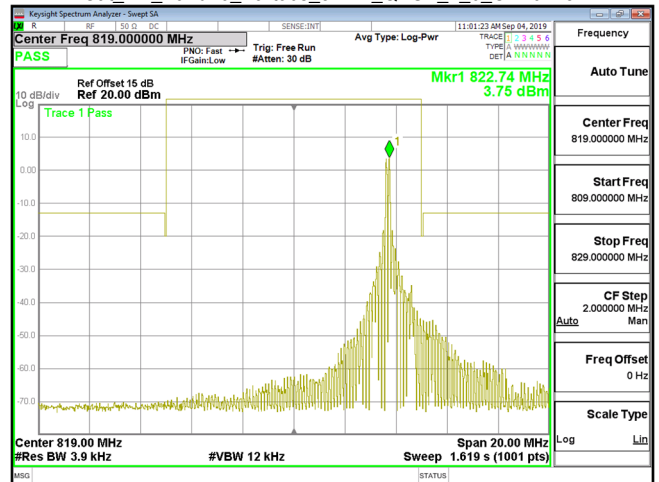
Cat_M1_Band26_Part90s_3MHz_QPSK_1_0_CH26775
