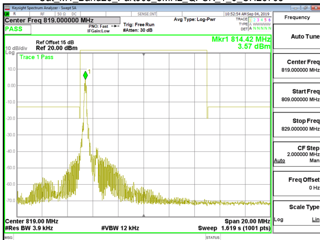
Cat_M1_Band26_Part90s_3MHz_QPSK_1_0_CH26705
