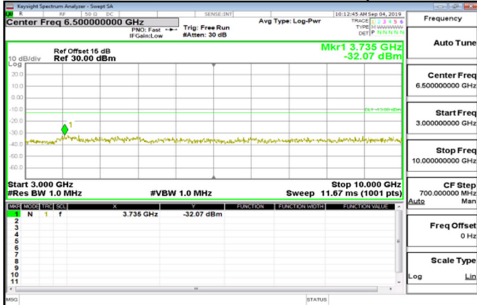
Cat_M1_3GHz~10GHz_Band26_Part90s_5MHz_QPSK_1_0_HighCH26765-821.5
