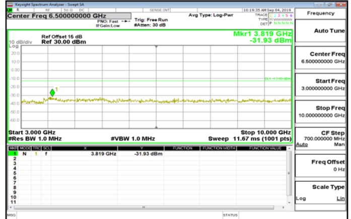
Cat M1_3GHz~10GHz_Band26_Part90s_3MHz_QPSK_1_0_LowCH26705-815.5
