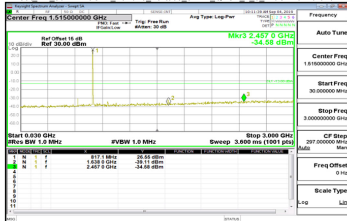
Cat_M1_30MHz~3GHz_Band26_Part90s_5MHz_QPSK_1_0_MidCH26740-819
