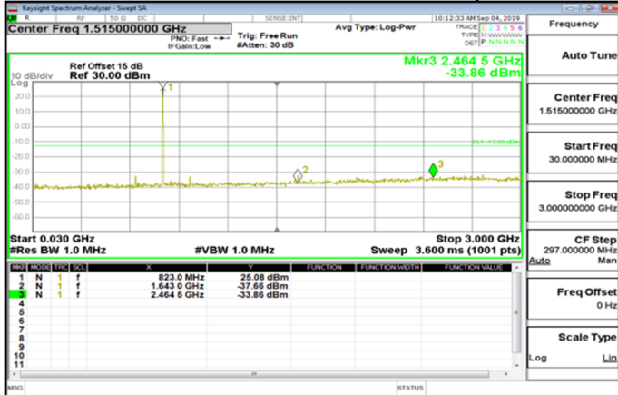
Cat_M1_30MHz~3GHz_Band26_Part90s_5MHz_QPSK_1_0_HighCH26765-821.5
