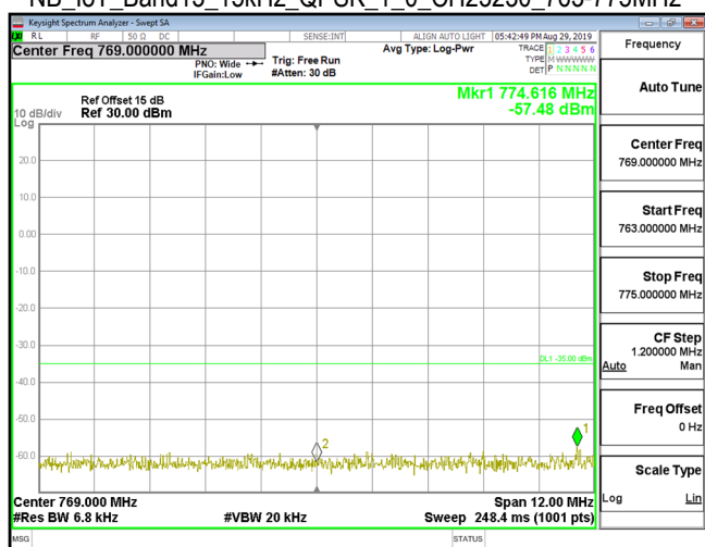
NB_IoT_Band13_15kHz_QPSK_1_0_CH23230_763-775MHz
