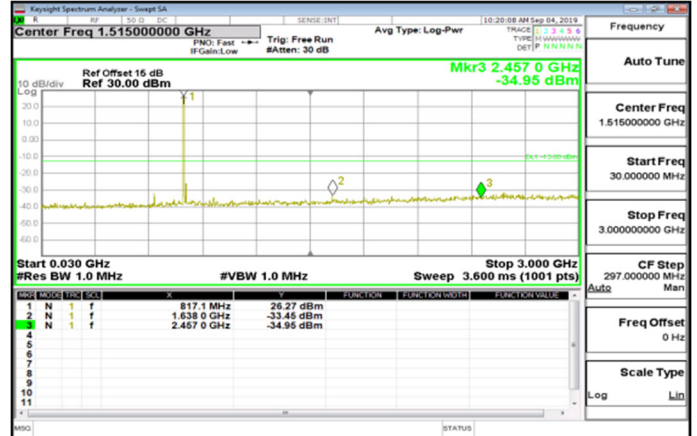
Cat M1_30MHz~3GHz_Band26_Part90s_3MHz_QPSK_1_0_MidCH26740-819
