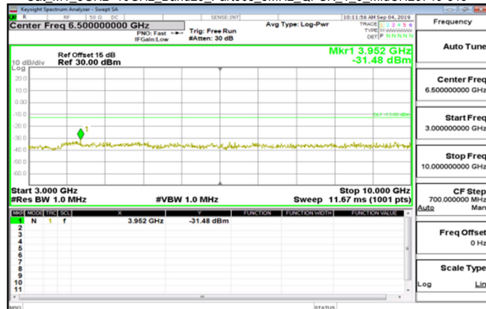
Cat_M1_3GHz~10GHz_Band26_Part90s_5MHz_QPSK_1_0_MidCH26740-819
