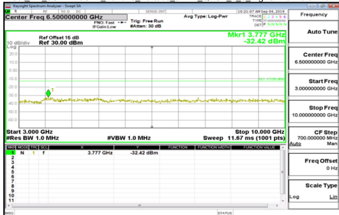
Cat_M1_3GHz~10GHz_Band26_Part90s_3MHz_QPSK_1_0_HighCH26775-822.5
