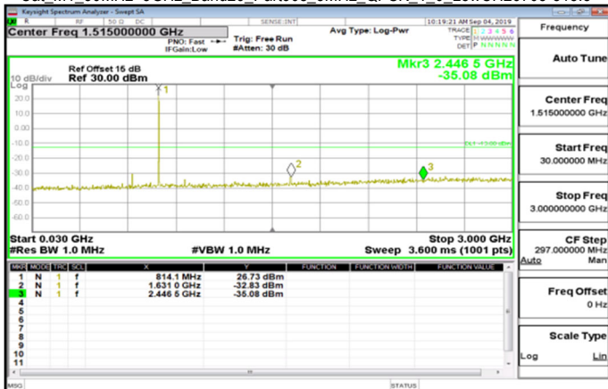
Cat M1_30MHz~3GHz_Band26_Part90s_3MHz_QPSK_1_0_LowCH26705-815.5
