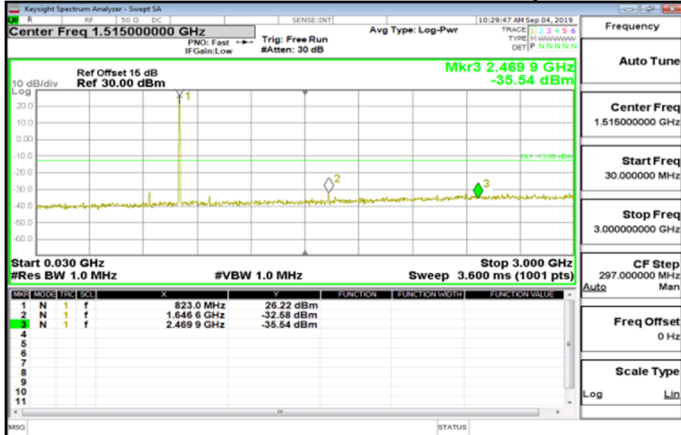
Cat M1_30MHz~3GHz_Band26_Part90s_1_4MHz_QPSK_1_0_HighCH26783-823.3
