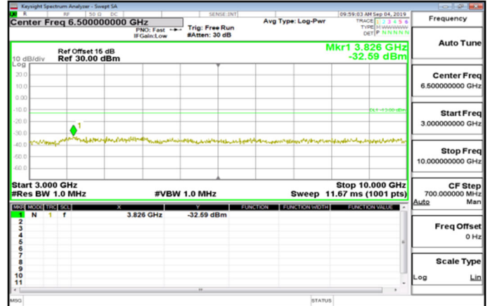
Cat_M1_3GHz~10GHz_Band26_Part90s_10MHz_QPSK_1_0_MidCH26740-819
