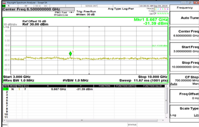
Cat M1_3GHz~10GHz_Band26_Part90s_1_4MHz_QPSK_1_0_HighCH26783-823.3
