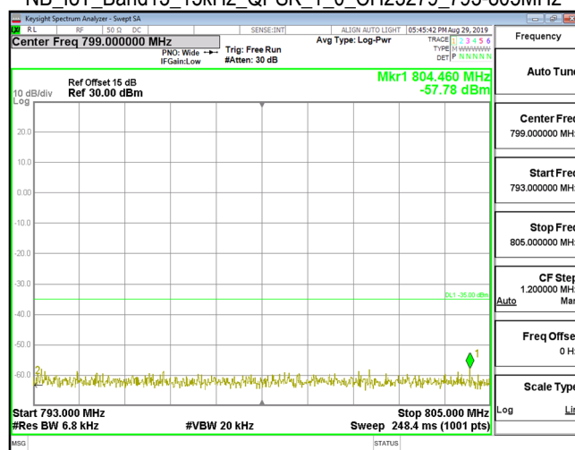
NB_IoT_Band13_15kHz_QPSK_1_0_CH23279_793-805MHz
