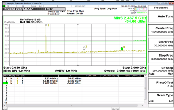
Cat_M1_30MHz~3GHz_Band26_Part90s_3MHz_QPSK_1_0_HighCH26775-822.5
