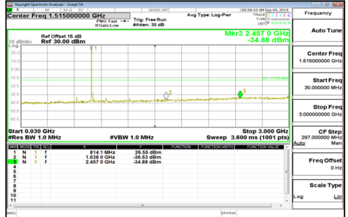
Cat_M1_30MHz~3GHz_Band26_Part90s_10MHz_QPSK_1_0_MidCH26740-819
