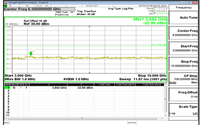
Cat_M1_3GHz~10GHz_Band26_3MHz_QPSK_1_0_LowCH26805-825.5
