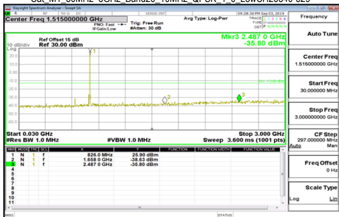
Cat_M1_30MHz~3GHz_Band26_10MHz_QPSK_1_0_LowCH26840-829
