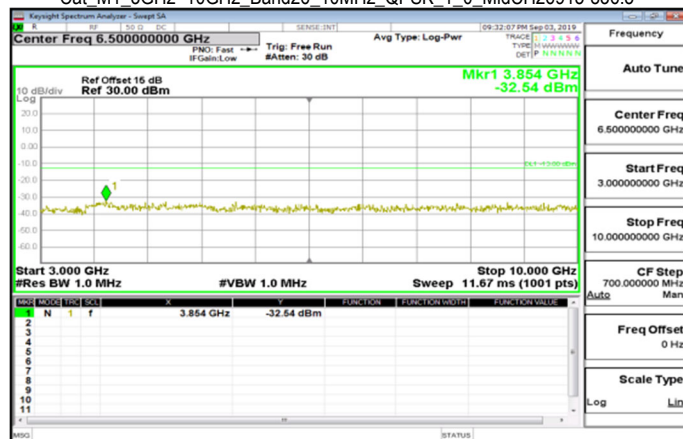
Cat_M1_3GHz~10GHz_Band26_10MHz_QPSK_1_0_MidCH26915-836.5
