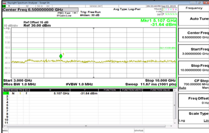
Cat_M1_3GHz~10GHz_Band26_10MHz_QPSK_1_0_HighCH26990-844
