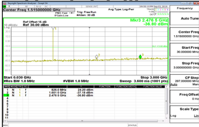
Cat_M1_30MHz~3GHz_Band26_3MHz_QPSK_1_0_LowCH26805-825.5
