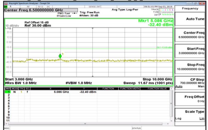
Cat_M1_3GHz~10GHz_Band26_3MHz_QPSK_1_0_MidCH26915-836.5
