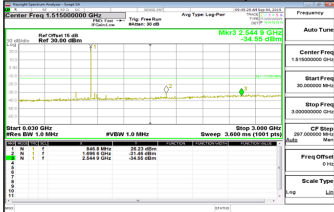
Cat_M1_30MHz~3GHz_Band26_1_4MHz_QPSK_1_0_HighCH27033-848.3
