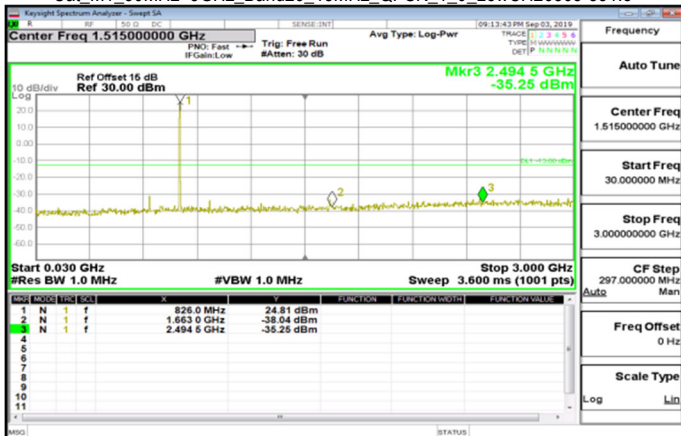
Cat_M1_30MHz~3GHz_Band26_15MHz_QPSK_1_0_LowCH26865-831.5
