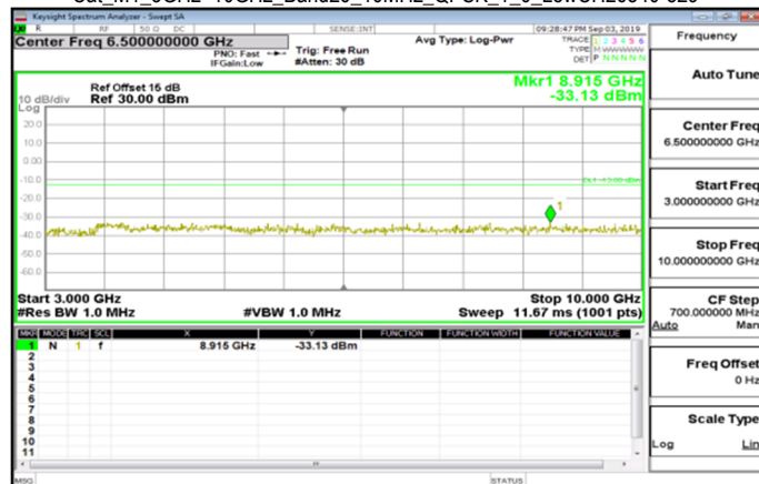
Cat_M1_3GHz~10GHz_Band26_10MHz_QPSK_1_0_LowCH26840-829
