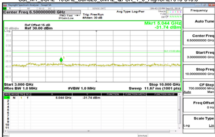
Cat_M1_3GHz~10GHz_Band26_5MHz_QPSK_1_0_HighCH27015-846.5
