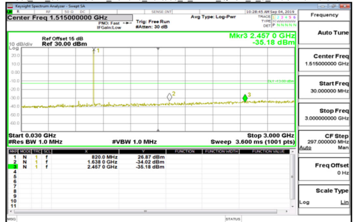
Cat M1_30MHz~3GHz_Band26_Part90s_1_4MHz_QPSK_1_0_MidCH26740-819
