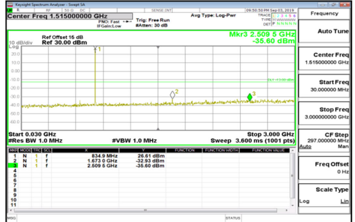
Cat_M1_30MHz~3GHz_Band26_3MHz_QPSK_1_0_MidCH26915-836.5
