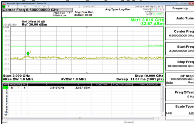
Cat M1_3GHz~10GHz_Band26_15MHz_QPSK_1_0_HighCH26965-841.5
