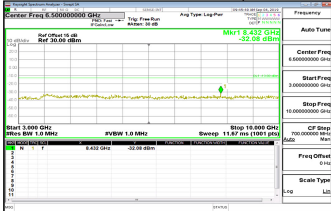
Cat_M1_3GHz~10GHz_Band26_1_4MHz_QPSK_1_0_HighCH27033-848.3
