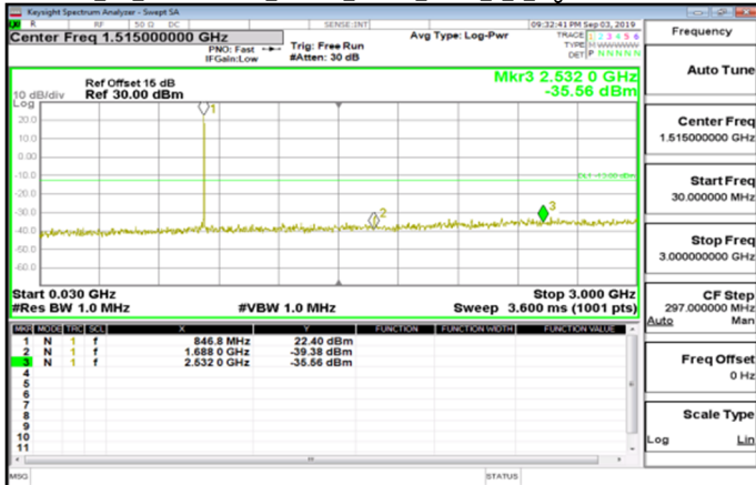
Cat_M1_30MHz~3GHz_Band26_10MHz_QPSK_1_0_HighCH26990-844
