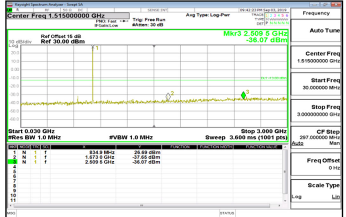
Cat_M1_30MHz~3GHz_Band26_5MHz_QPSK_1_0_MidCH26915-836.5
