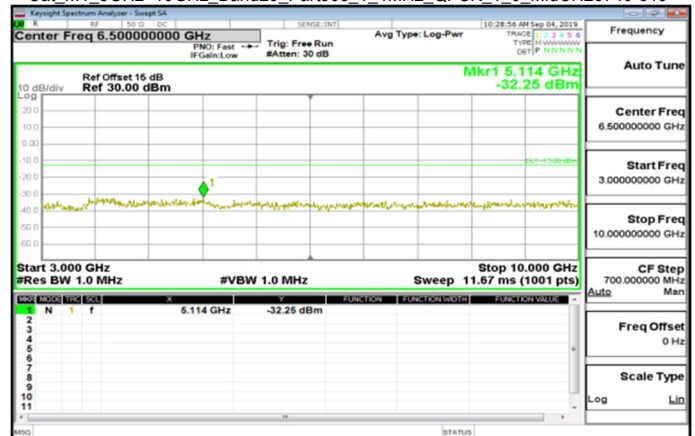
Cat M1_3GHz~10GHz_Band26_Part90s_1_4MHz_QPSK_1_0_MidCH26740-819
