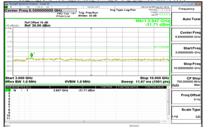
Cat_M1_3GHz~10GHz_Band26_15MHz_QPSK_1_0_MidCH26915-836.5
