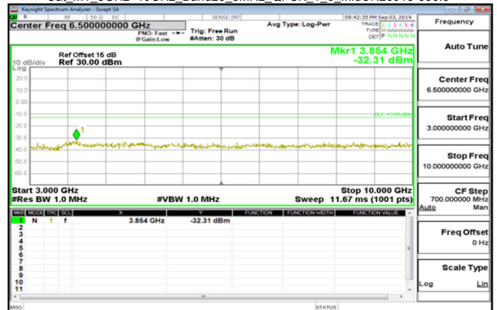
Cat_M1_3GHz~10GHz_Band26_5MHz_QPSK_1_0_MidCH26915-836.5
