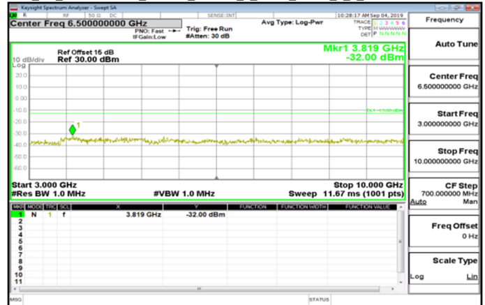
Cat M1_3GHz~10GHz_Band26_Part90s_1_4MHz_QPSK_1_0_LowCH26697-814.7
