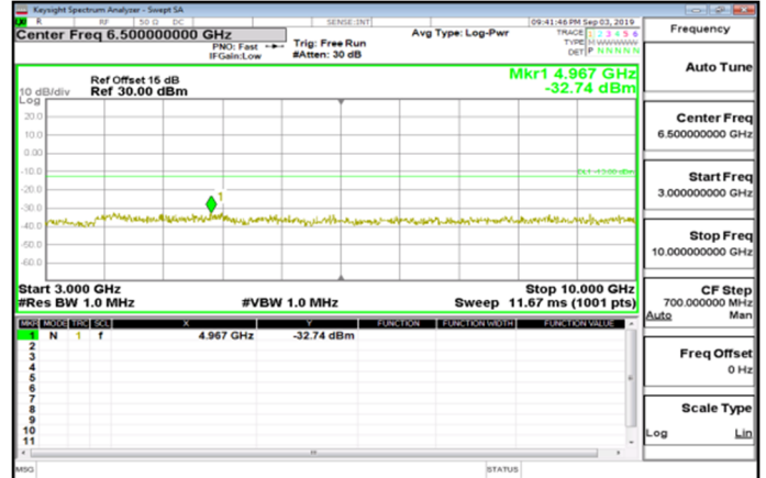
Cat_M1_3GHz~10GHz_Band26_5MHz_QPSK_1_0_LowCH26815-826.5
