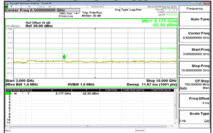
Cat_M1_3GHz~10GHz_Band26_15MHz_QPSK_1_0_LowCH26865-831.5
