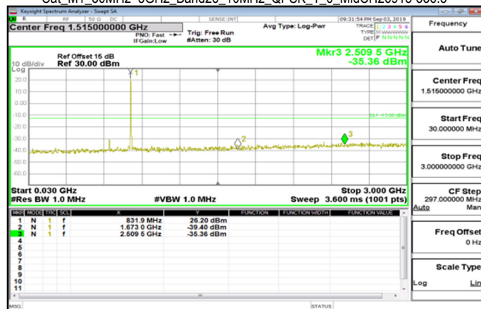
Cat_M1_30MHz~3GHz_Band26_10MHz_QPSK_1_0_MidCH26915-836.5
