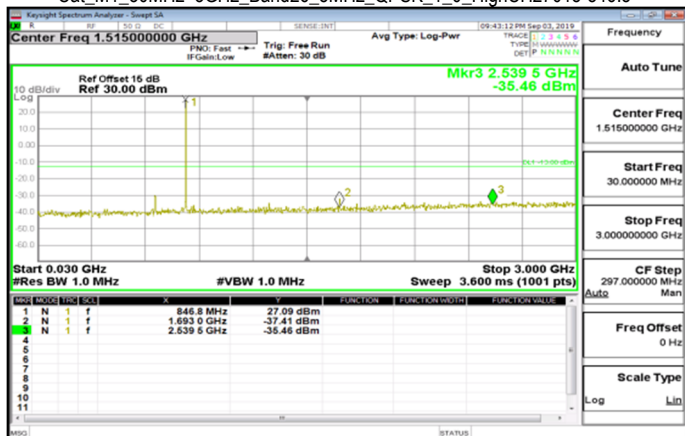
Cat_M1_30MHz~3GHz_Band26_5MHz_QPSK_1_0_HighCH27015-846.5
