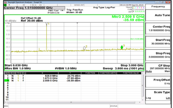
Cat_M1_30MHz~3GHz_Band26_15MHz_QPSK_1_0_MidCH26915-836.5
