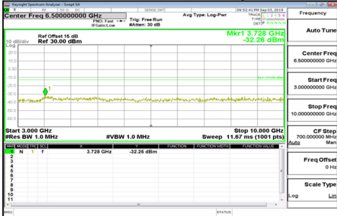
Cat_M1_3GHz~10GHz_Band26_3MHz_QPSK_1_0_HighCH27025-847.5
