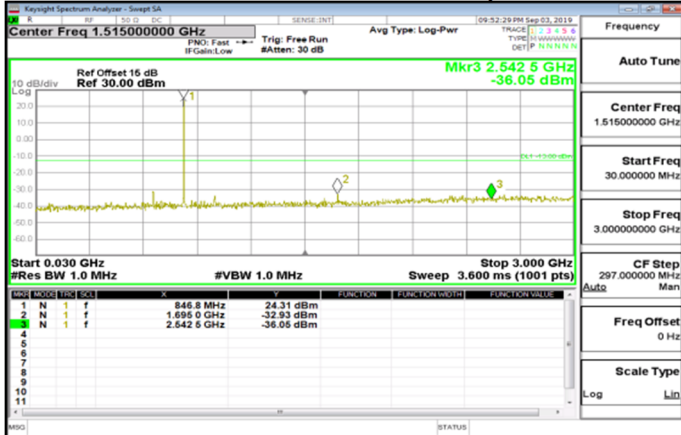
Cat_M1_30MHz~3GHz_Band26_3MHz_QPSK_1_0_HighCH27025-847.5
