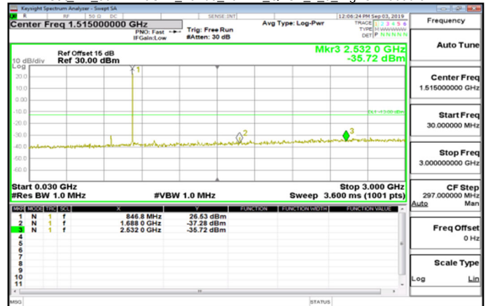
Cat M1_30MHz~3GHz_Band5_10MHz_QPSK_1_0_HighCH20600-844
