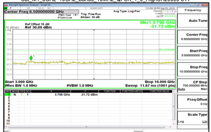
Cat M1_3GHz~10GHz_Band5_10MHz_QPSK_1_0_HighCH20600-844
