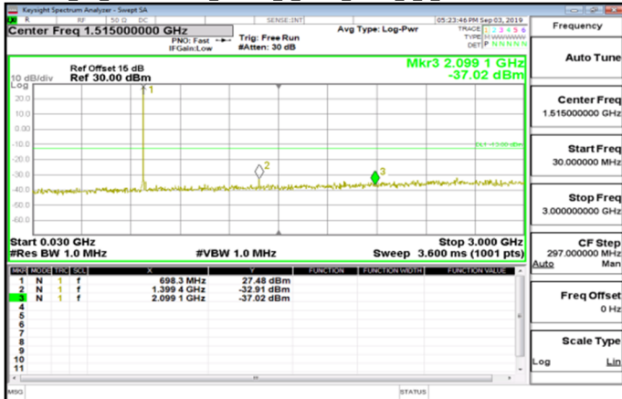
Cat M1_30MHz~3GHz_Band12_1.4MHz_QPSK_1_0_LowCH23017-699.7
