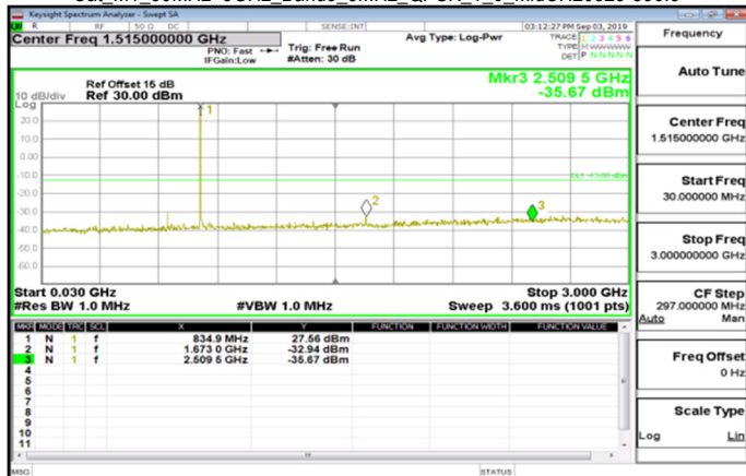
Cat_M1_30MHz~3GHz_Band5_3MHz_QPSK_1_0_MidCH20525-836.5
