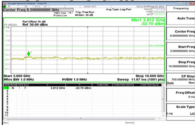
Cat_M1_3GHz~10GHz_Band5_3MHz_QPSK_1_0_LowCH20415-825.5
