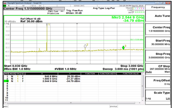
Cat_M1_30MHz~3GHz_Band5_1_4MHz_QPSK_1_0_HighCH20643-848.3
