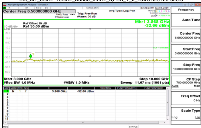
Cat_M1_3GHz~10GHz_Band5_5MHz_QPSK_1_0_LowCH20425-826.5
