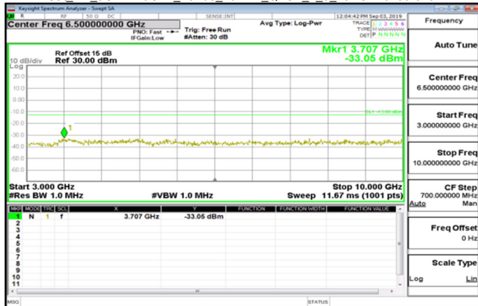
Cat M1_3GHz~10GHz_Band5_10MHz_QPSK_1_0_LowCH20450-829
