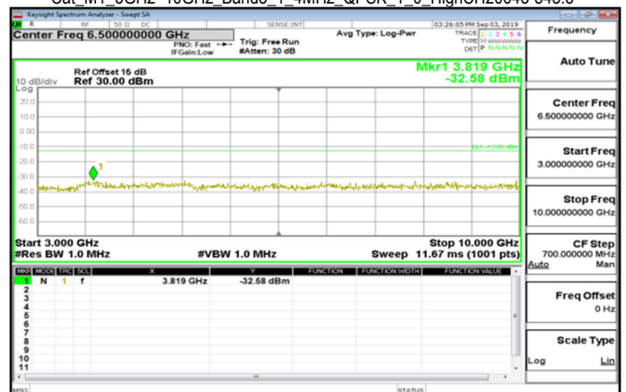
Cat_M1_3GHz~10GHz_Band5_1_4MHz_QPSK_1_0_HighCH20643-848.3
