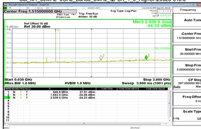
Cat_M1_30MHz~3GHz_Band5_5MHz_QPSK_1_0_HighCH20625-846.5
