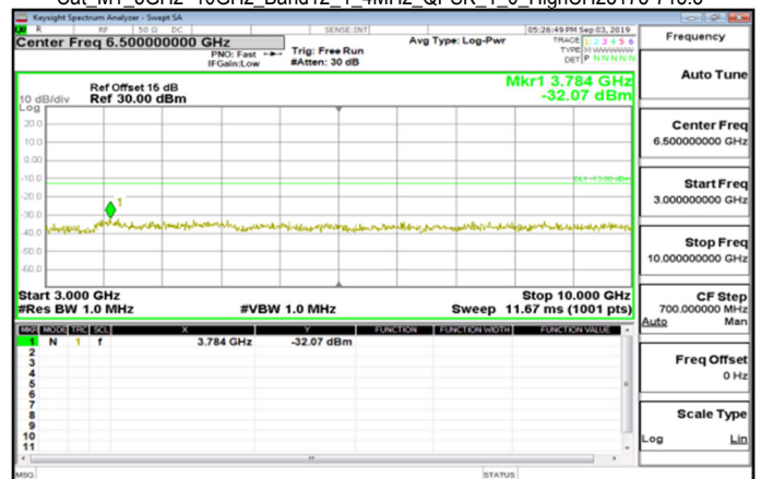
Cat M1_3GHz~10GHz_Band12_1.4MHz_QPSK_1_0_HighCH23173-715.3
