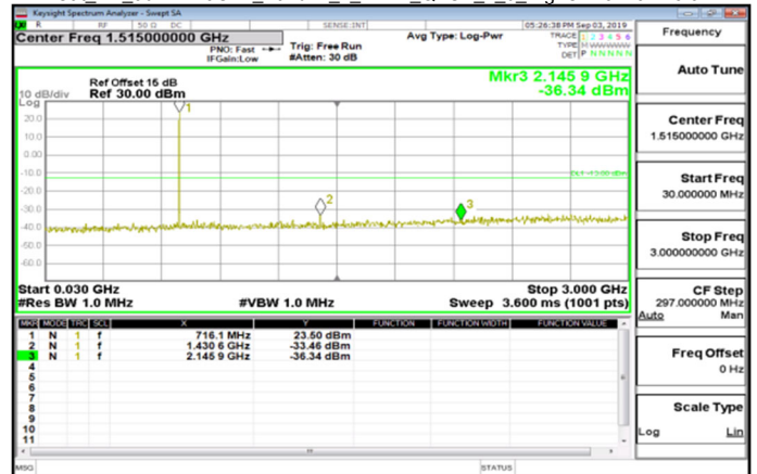
Cat M1_30MHz~3GHz_Band12_1.4MHz_QPSK_1_0_HighCH23173-715.3
