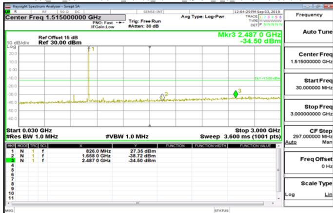
Cat M1_30MHz~3GHz_Band5_10MHz_QPSK_1_0_LowCH20450-829
