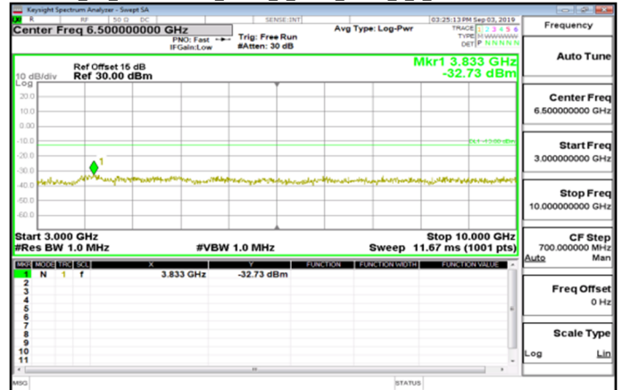
Cat_M1_3GHz~10GHz_Band5_1_4MHz_QPSK_1_0_MidCH20525-836.5
