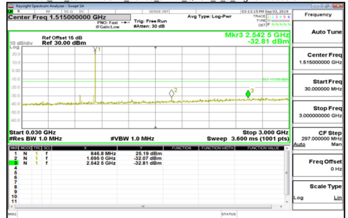
Cat_M1_30MHz~3GHz_Band5_3MHz_QPSK_1_0_HighCH20635-847.5
