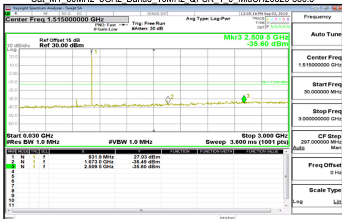
Cat M1_30MHz~3GHz_Band5_10MHz_QPSK_1_0_MidCH20525-836.5
