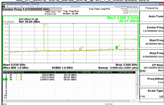
Cat_M1_30MHz~3GHz_Band5_5MHz_QPSK_1_0_MidCH20525-836.5
