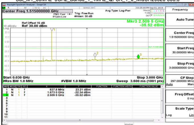
Cat_M1_30MHz~3GHz_Band5_1_4MHz_QPSK_1_0_MidCH20525-836.5
