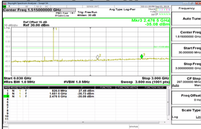
Cat_M1_30MHz~3GHz_Band5_3MHz_QPSK_1_0_LowCH20415-825.5
