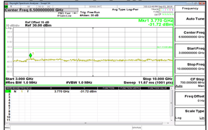
Cat_M1_3GHz~10GHz_Band5_3MHz_QPSK_1_0_MidCH20525-836.5
