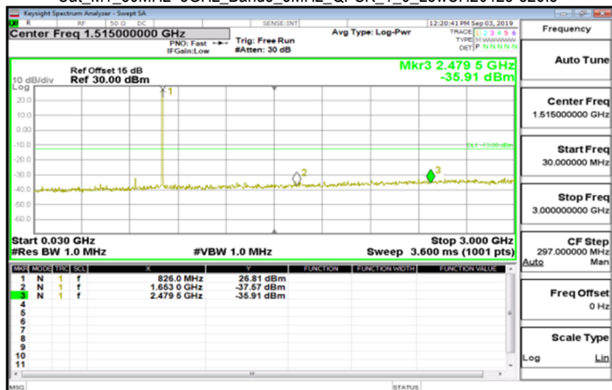
Cat_M1_30MHz~3GHz_Band5_5MHz_QPSK_1_0_LowCH20425-826.5
