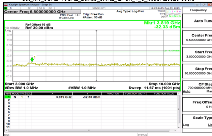
Cat_M1_3GHz~10GHz_Band5_5MHz_QPSK_1_0_MidCH20525-836.5
