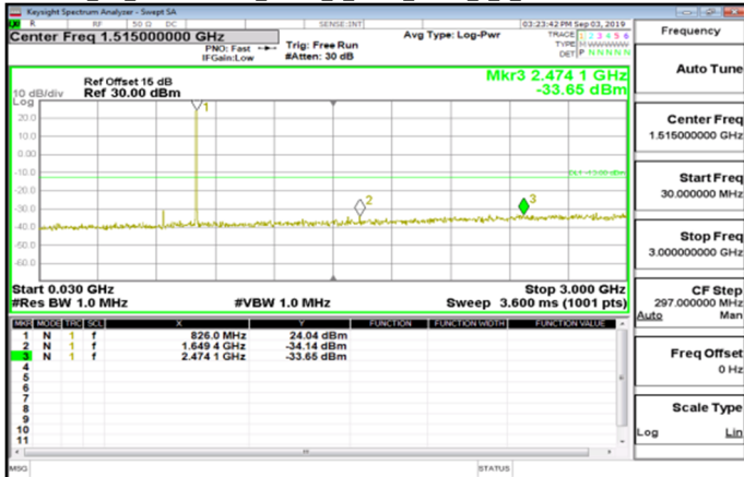
Cat_M1_30MHz~3GHz_Band5_1_4MHz_QPSK_1_0_LowCH20407-824.7
