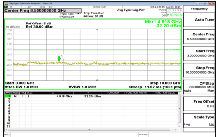
Cat M1_3GHz~10GHz_Band12_1.4MHz_QPSK_1_0_MidCH23095-707.5
