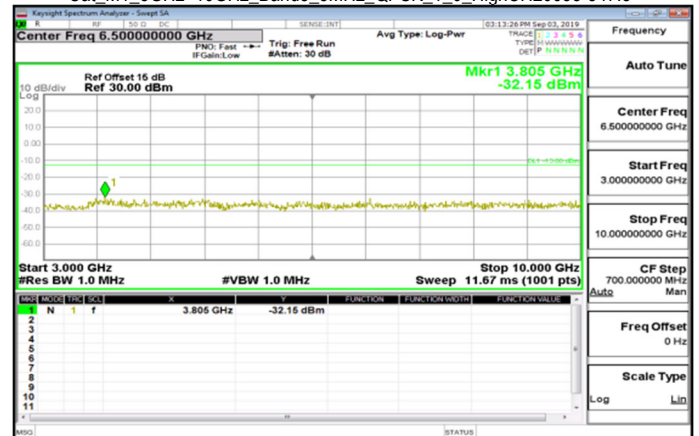
Cat_M1_3GHz~10GHz_Band5_3MHz_QPSK_1_0_HighCH20635-847.5
