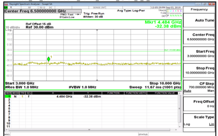
Cat M1_3GHz~10GHz_Band5_10MHz_QPSK_1_0_MidCH20525-836.5
