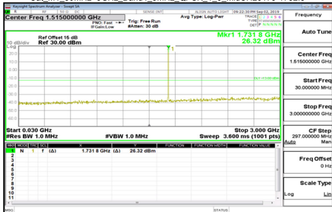
Cat M1_30MHz~3GHz_Band4_5MHz_QPSK_1_0_MidCH20175-1732.5
