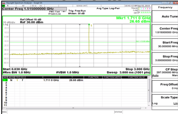
Cat M1_30MHz~3GHz_Band4_3MHz_QPSK_1_0_LowCH19965-1711.5
