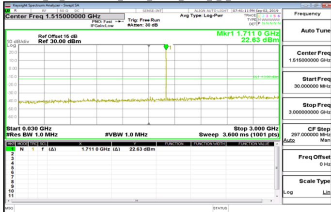
Cat M1_30MHz~3GHz_Band4_20MHz_QPSK_1_0_LowCH20050-1720
