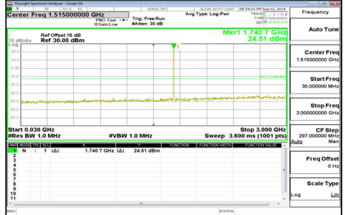
Cat_M1_30MHz~3GHz_Band4_15MHz_QPSK_1_0_HighCH20325-1747.5
