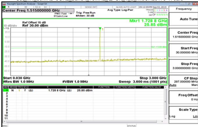
Cat M1_30MHz~3GHz_Band4_10MHz_QPSK_1_0_MidCH20175-1732.5
