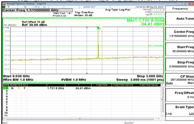
Cat M1_30MHz~3GHz_Band4_3MHz_QPSK_1_0_MidCH20175-1732.5
