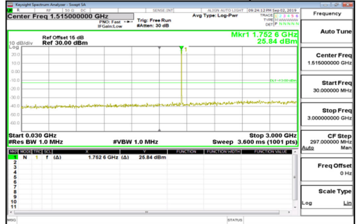
Cat M1_30MHz~3GHz_Band4_5MHz_QPSK_1_0_HighCH20375-1752.5
