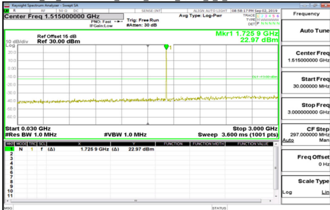
Cat_M1_30MHz~3GHz_Band4_15MHz_QPSK_1_0_MidCH20175-1732.5
