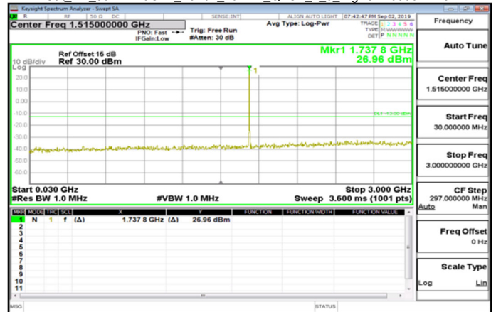
Cat M1_30MHz~3GHz_Band4_20MHz_QPSK_1_0_HighCH20300-1745
