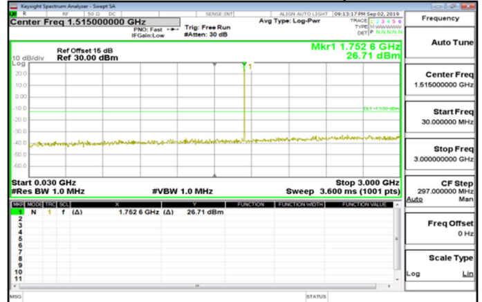
Cat M1_30MHz~3GHz_Band4_10MHz_QPSK_1_0_HighCH20350-1750
