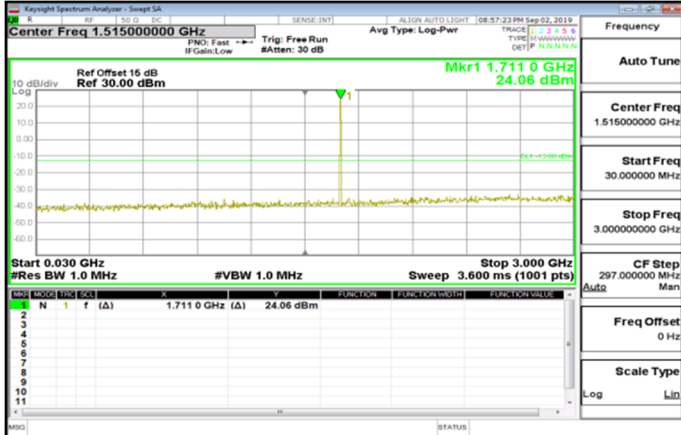
Cat_M1_30MHz~3GHz_Band4_15MHz_QPSK_1_0_LowCH20025-1717.5
