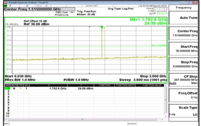
Cat M1_30MHz~3GHz_Band4_3MHz_QPSK_1_0_HighCH20385-1753.5
