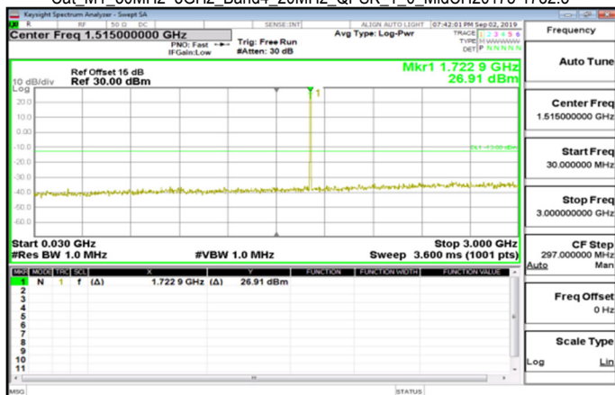
Cat M1_30MHz~3GHz_Band4_20MHz_QPSK_1_0_MidCH20175-1732.5
