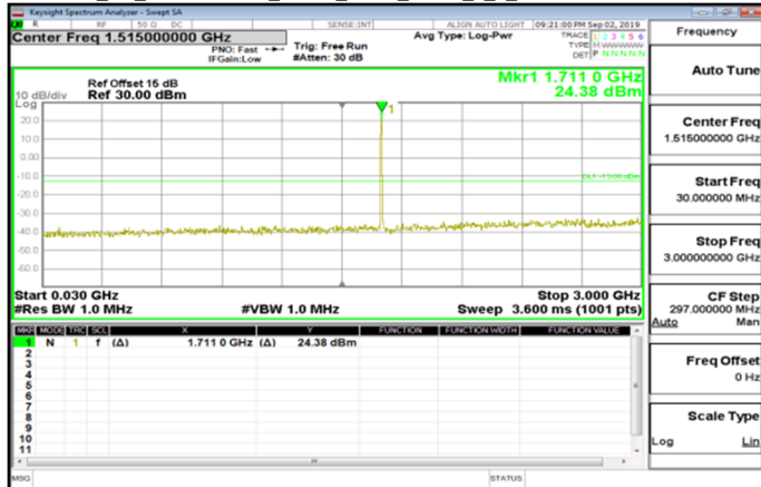
Cat M1_30MHz~3GHz_Band4_5MHz_QPSK_1_0_LowCH19975-1712.5
