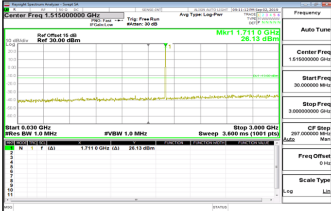
Cat M1_30MHz~3GHz_Band4_10MHz_QPSK_1_0_LowCH20000-1715
