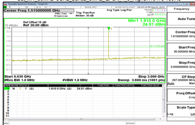
Cat_M1_30MHz~3GHz_Band2_5MHz_QPSK_1_0_HighCH19175-1907.5
