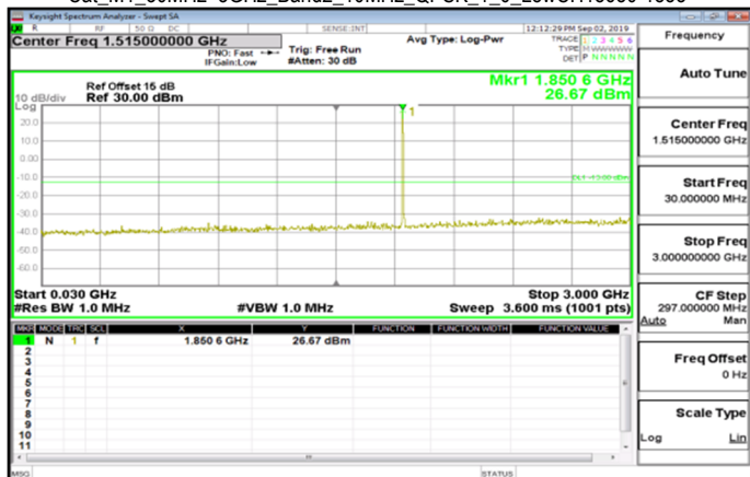
Cat M1_30MHz~3GHz_Band2_10MHz_QPSK_1_0_LowCH18650-1855
