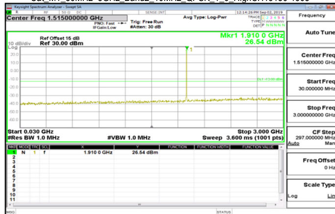
Cat M1_30MHz~3GHz_Band2_10MHz_QPSK_1_0_HighCH19150-1905
