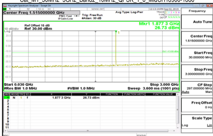
Cat M1_30MHz~3GHz_Band2_10MHz_QPSK_1_0_MidCH18900-1880
