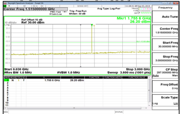
Cat M1_30MHz~3GHz_Band4_1_4MHz_QPSK_1_0_HighCH20393-1754.3
