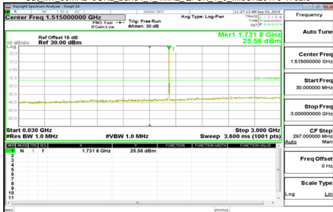
Cat M1_30MHz~3GHz_Band4_1_4MHz_QPSK_1_0_MidCH20175-1732.5
