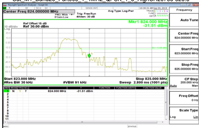
Cat_M1_Band26_Part90s_1_4MHz_QPSK_1_5_HighCH26783-823.3
