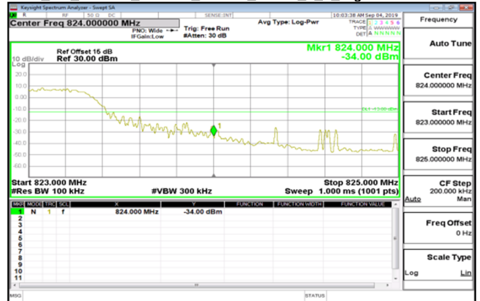
Cat_M1_Band26_Part90s_10MHz_QPSK_6_0_HighCH26740-819
