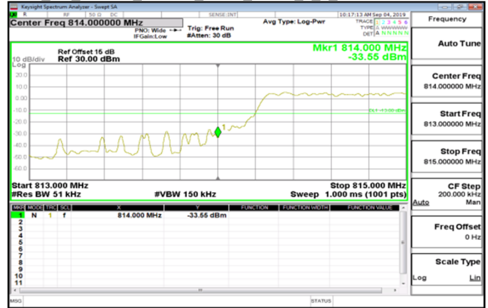
Cat M1_Band26_Part90s_5MHz_QPSK_6_0_LowCH26715-816.5
