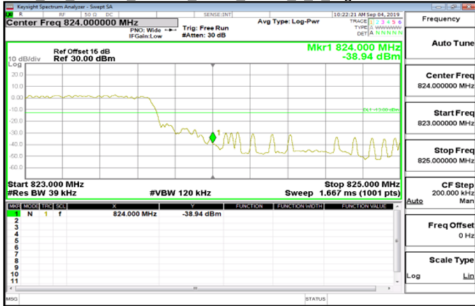
Cat M1_Band26_Part90s_3MHz_QPSK_6_0_HighCH26775-822.5
