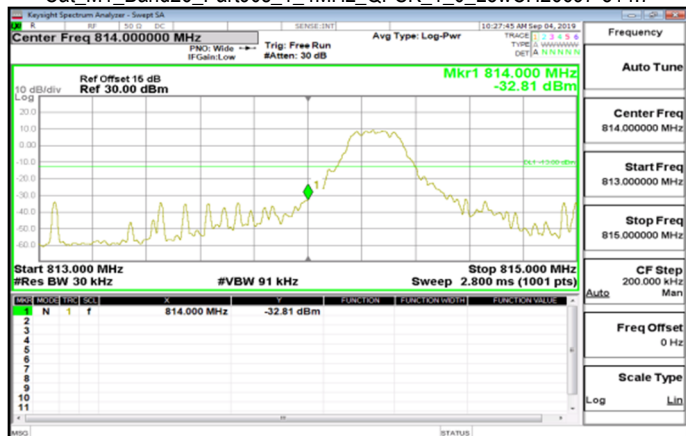
Cat_M1_Band26_Part90s_1_4MHz_QPSK_1_0_LowCH26697-814.7
