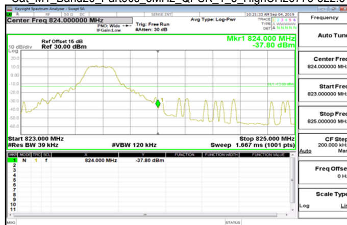
Cat_M1_Band26_Part90s_3MHz_QPSK_1_5_HighCH26775-822.5
