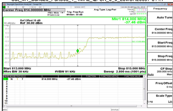
Cat_M1_Band26_Part90s_1_4MHz_QPSK_6_0_LowCH26697-814.7
