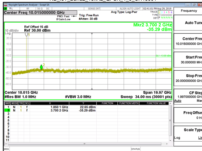
NB_IoT_Band2_15kHz_QPSK_1_0_CH18900
