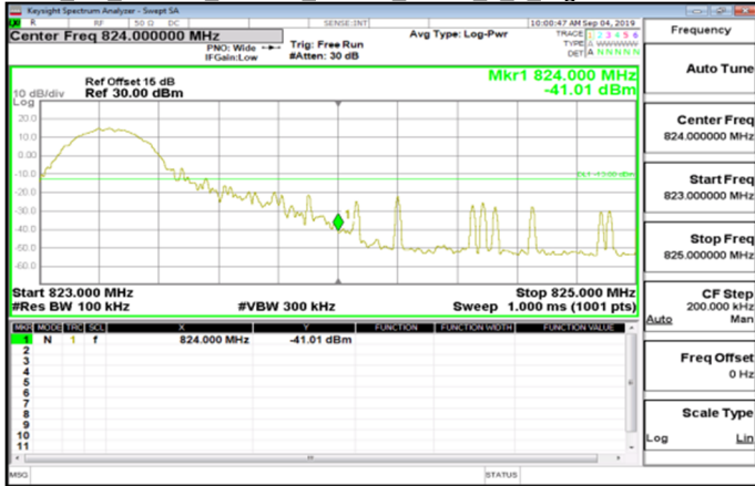
Cat_M1_Band26_Part90s_10MHz_QPSK_1_5_HighCH26740-819
