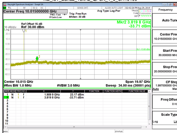
NB_IoT_Band2_15kHz_QPSK_1_0_CH19199
