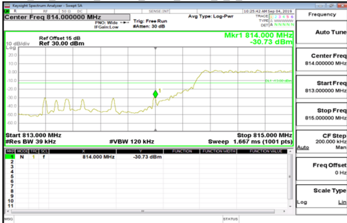
Cat M1_Band26_Part90s_3MHz_QPSK_6_0_LowCH26705-815.5
