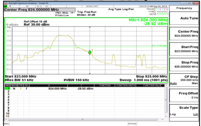
Cat M1_Band26_Part90s_5MHz_QPSK_1_5_HighCH26765-821.5
