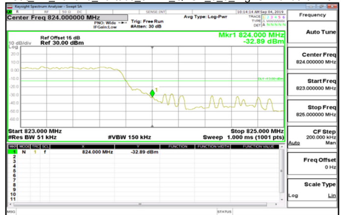
Cat M1_Band26_Part90s_5MHz_QPSK_6_0_HighCH26765-821.5
