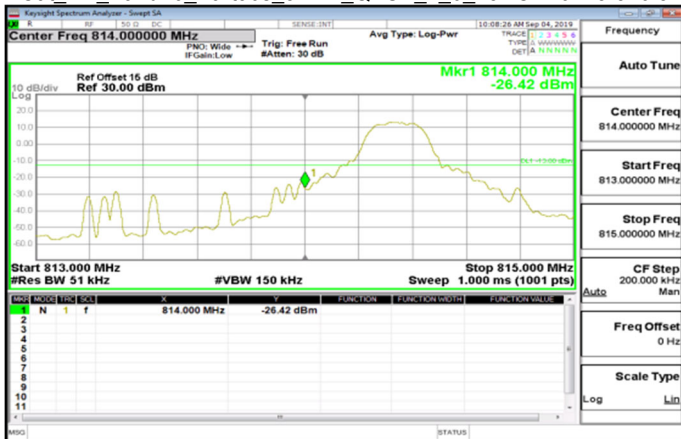
Cat M1_Band26_Part90s_5MHz_QPSK_1_0_LowCH26715-816.5
