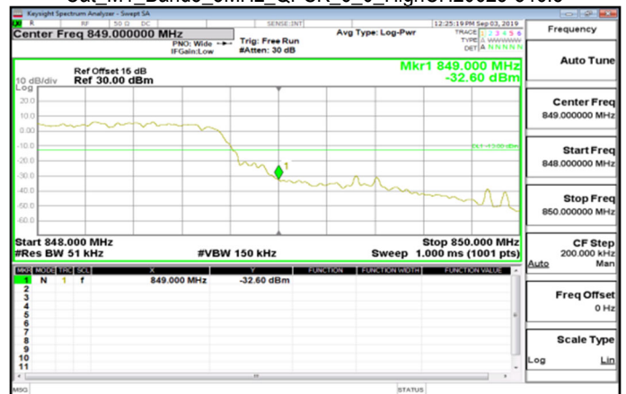
Cat_M1_Band5_5MHz_QPSK_6_0_HighCH20625-846.5
