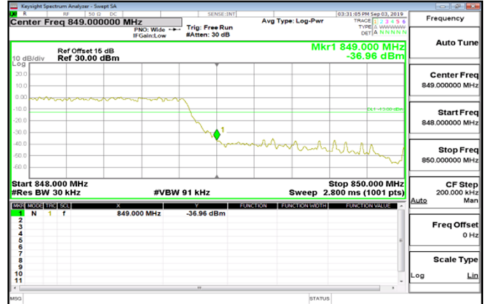
Cat M1_Band5_1_4MHz_QPSK_6_0_HighCH20643-848.3
