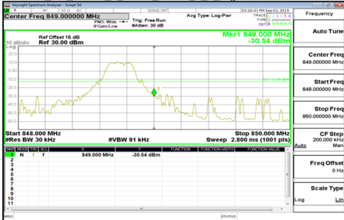
Cat M1_Band5_1_4MHz_QPSK_1_5_HighCH20643-848.3
