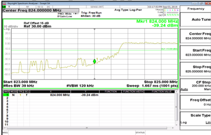
Cat_M1_Band5_3MHz_QPSK_6_0_LowCH20415-825.5
