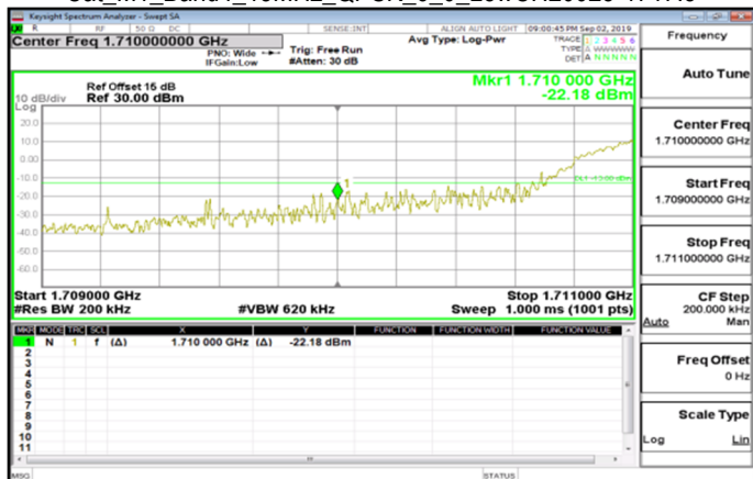
Cat_M1_Band4_15MHz_QPSK_6_0_LowCH20025-1717.5
