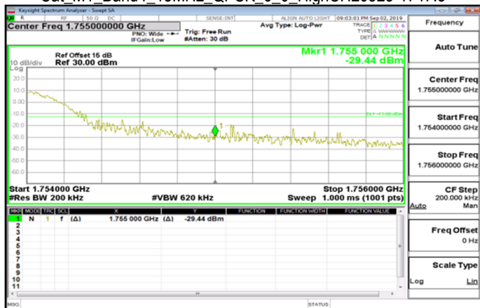
Cat_M1_Band4_15MHz_QPSK_6_0_HighCH20325-1747.5
