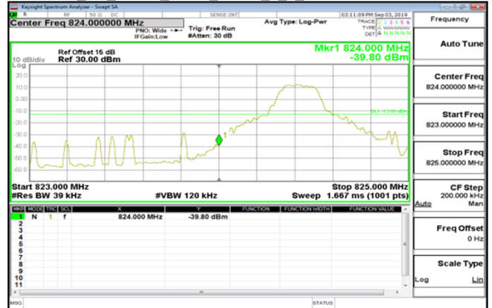
Cat M1_Band5_3MHz_QPSK_1_0_LowCH20415-825.5
