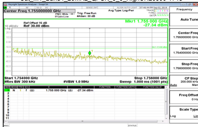
Cat_M1_Band4_20MHz_QPSK_6_0_HighCH20300-1745
