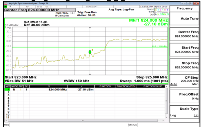
Cat_M1_Band5_5MHz_QPSK_6_0_LowCH20425-826.5
