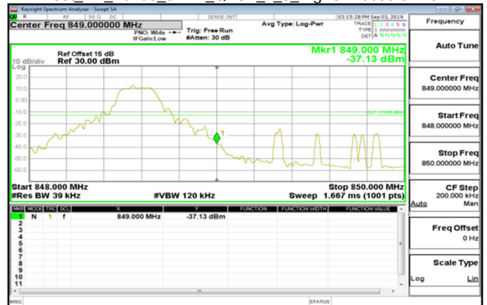
Cat M1_Band5_3MHz_QPSK_1_5_HighCH20635-847.5
