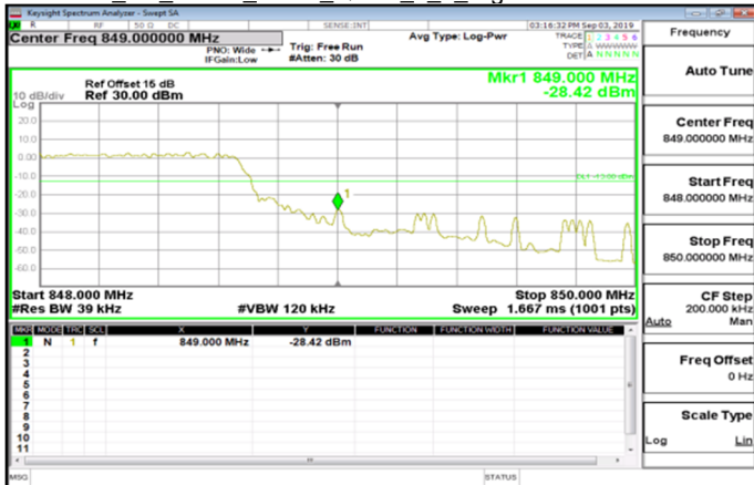
Cat_M1_Band5_3MHz_QPSK_6_0_HighCH20635-847.5
