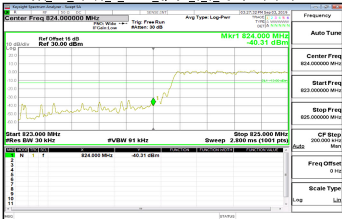
Cat M1_Band5_1_4MHz_QPSK_6_0_LowCH20407-824.7
