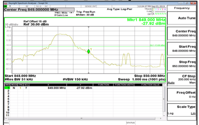
Cat_M1_Band5_5MHz_QPSK_1_5_HighCH20625-846.5
