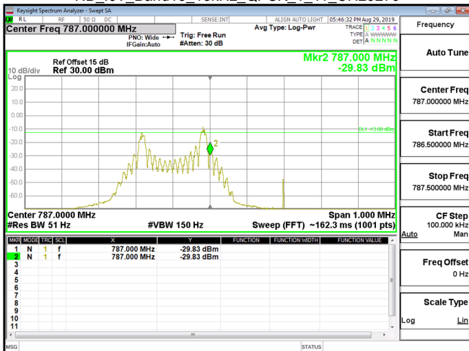
NB_IoT_Band13_15kHz_QPSK_1_11_CH23279
