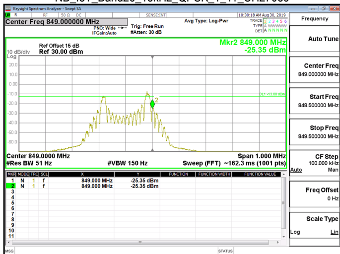
NB_IoT_Band26_15kHz_QPSK_1_11_CH27039
