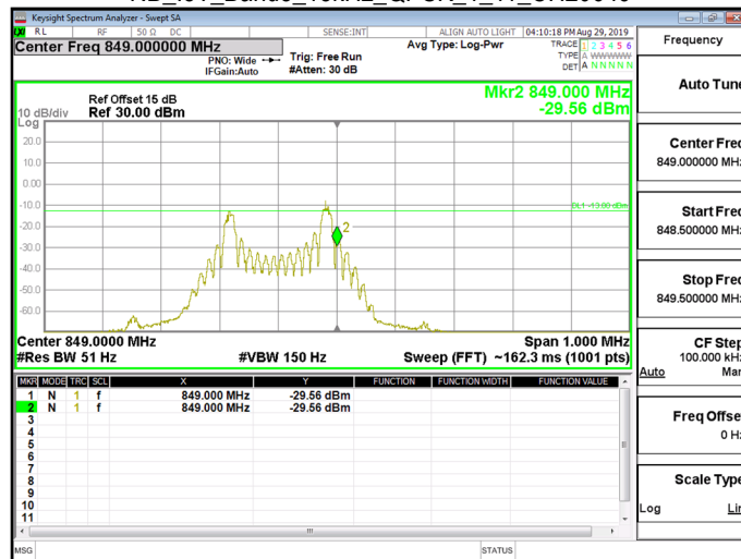
NB_IoT_Band5_15kHz_QPSK_12_0_CH20401
