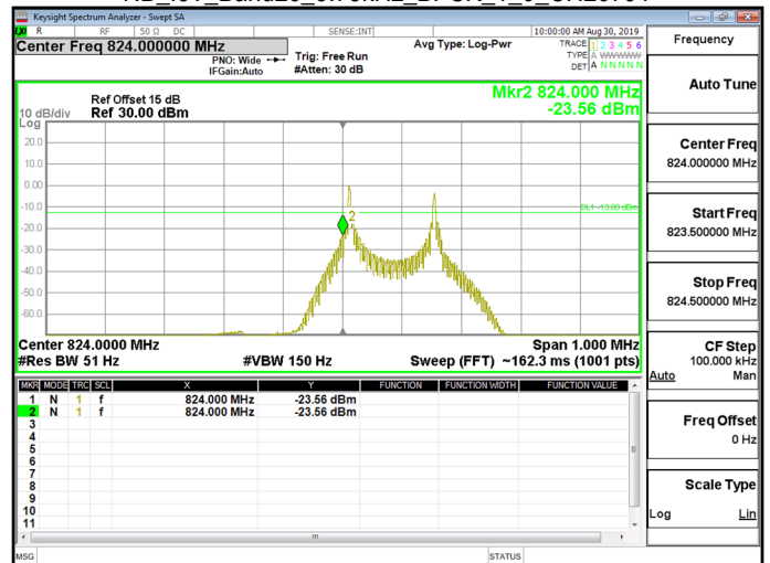
NB_IoT_Band26_3.75kHz_BPSK_1_0_CH26791
