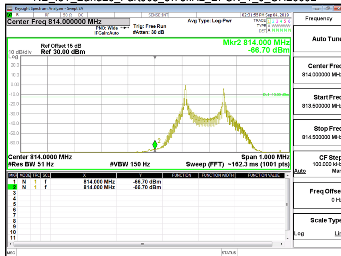
NB_IoT_Band26_Part90s_3.75kHz_BPSK_1_0_CH26692
