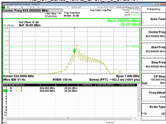
NB_IoT_Band5_15kHz_QPSK_1_0_CH20401
