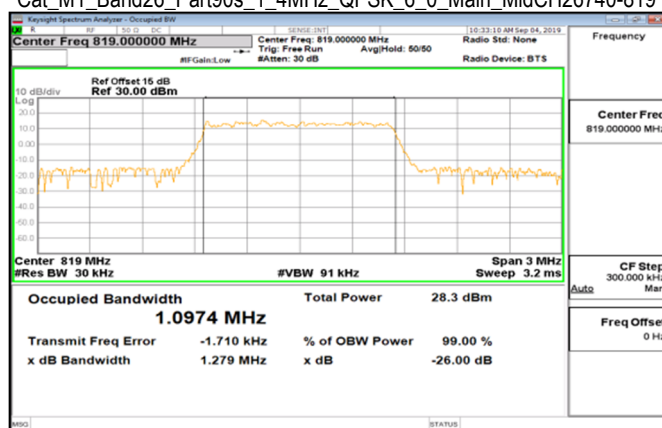
Cat_M1_Band26_Part90s_1_4MHz_QPSK_6_0_Main_MidCH26740-819
