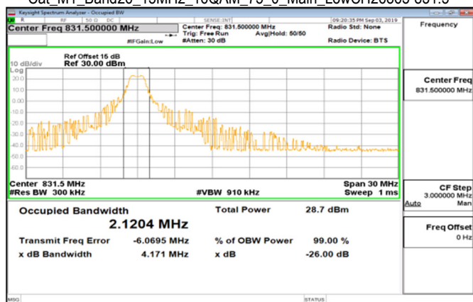
Cat_M1_Band26_15MHz_16QAM_75_0_Main_LowCH26865-831.5
