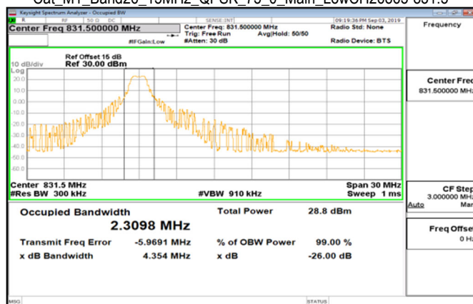
Cat_M1_Band26_15MHz_QPSK_75_0_Main_LowCH26865-831.5
