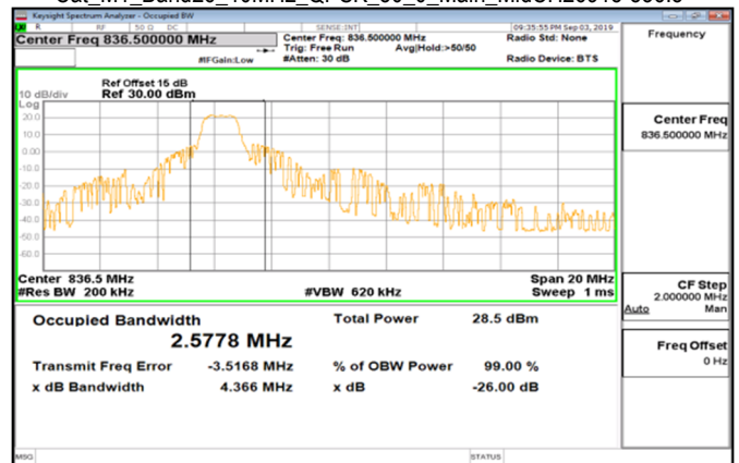
Cat_M1_Band26_10MHz_QPSK_50_0_Main_MidCH26915-836.5
