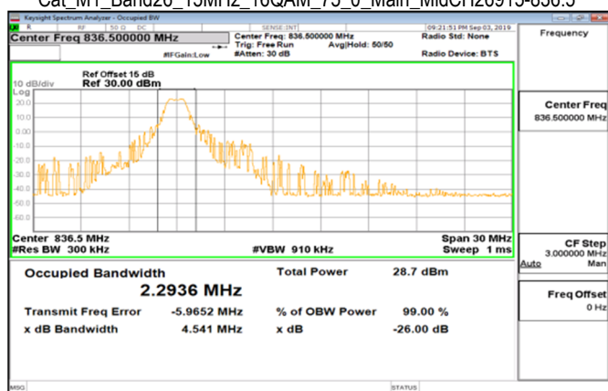
Cat_M1_Band26_15MHz_16QAM_75_0_Main_MidCH26915-836.5
