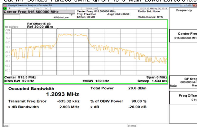
Cat_M1_Band26_Part90s_3MHz_QPSK_15_0_Main_LowCH26705-815.5
