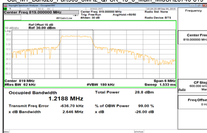
Cat_M1_Band26_Part90s_3MHz_QPSK_15_0_Main_MidCH26740-819
