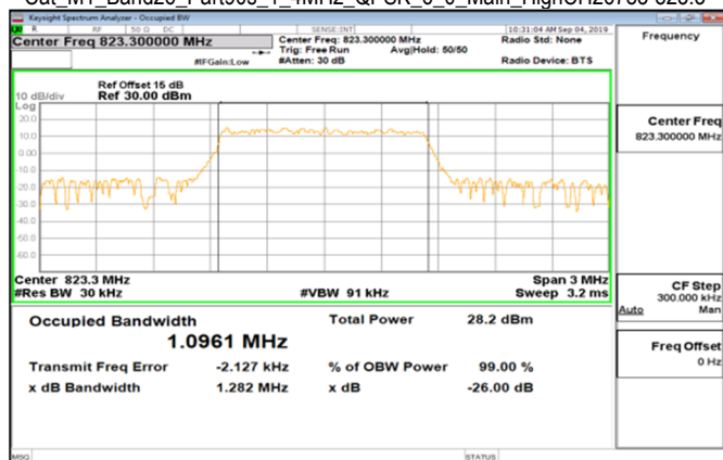
Cat_M1_Band26_Part90s_1_4MHz_QPSK_6_0_Main_HighCH26783-823.3
