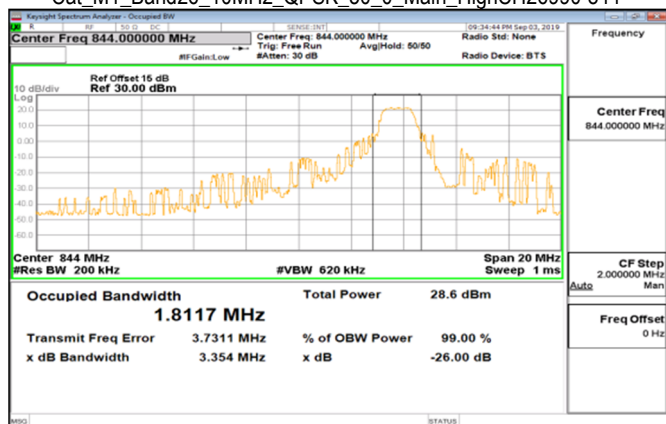
Cat_M1_Band26_10MHz_QPSK_50_0_Main_HighCH26990-844
