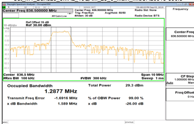
Cat_M1_Band26_5MHz_16QAM_25_0_Main_MidCH26915-836.5
