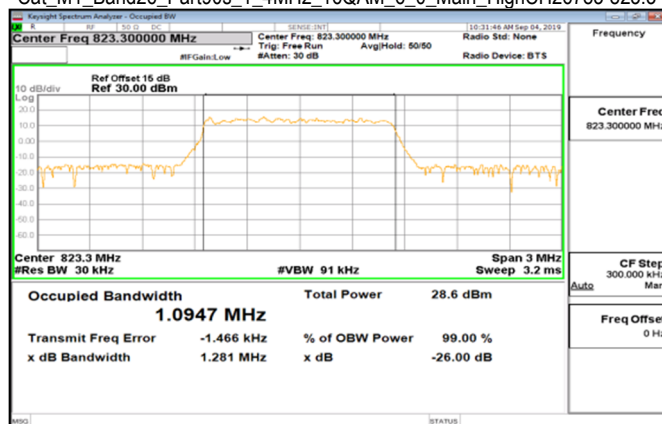
Cat_M1_Band26_Part90s_1_4MHz_16QAM_6_0_Main_HighCH26783-823.3
