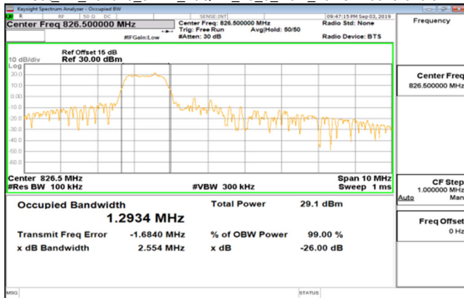
Cat_M1_Band26_5MHz_16QAM_25_0_Main_LowCH26815-826.5
