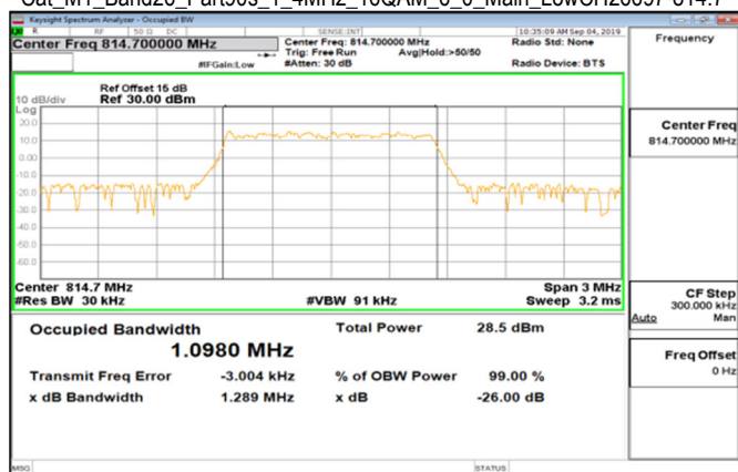
Cat_M1_Band26_Part90s_1_4MHz_16QAM_6_0_Main_LowCH26697-814.7
