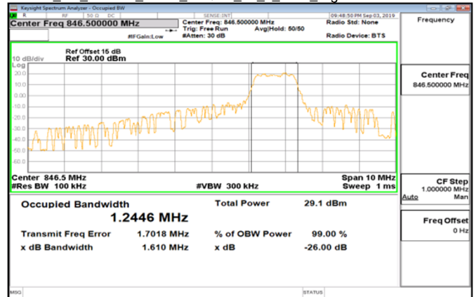
Cat_M1_Band26_5MHz_16QAM_25_0_Main_HighCH27015-846.5
