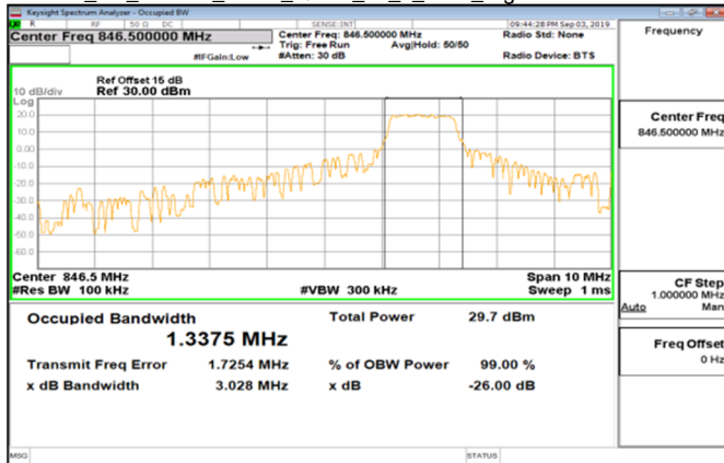
Cat_M1_Band26_5MHz_QPSK_25_0_Main_HighCH27015-846.5
