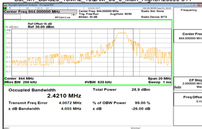
Cat_M1_Band26_10MHz_16QAM_50_0_Main_HighCH26990-844
