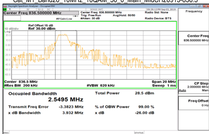
Cat_M1_Band26_10MHz_16QAM_50_0_Main_MidCH26915-836.5
