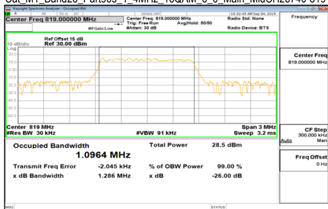
Cat_M1_Band26_Part90s_1_4MHz_16QAM_6_0_Main_MidCH26740-819
