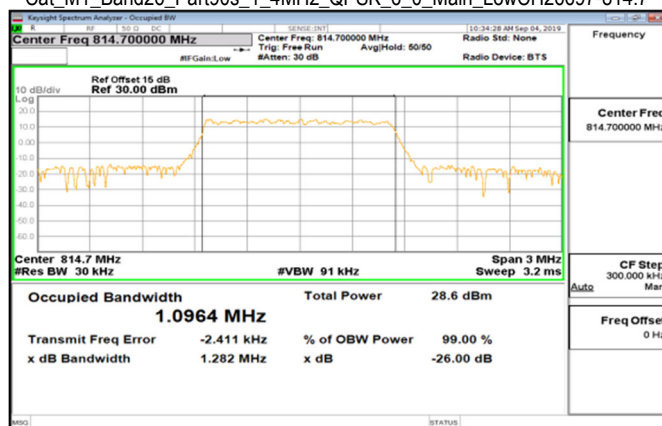
Cat_M1_Band26_Part90s_1_4MHz_QPSK_6_0_Main_LowCH26697-814.7
