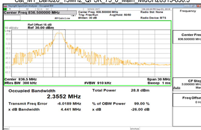
Cat_M1_Band26_15MHz_QPSK_75_0_Main_MidCH26915-836.5
