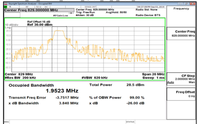
Cat_M1_Band26_10MHz_QPSK_50_0_Main_LowCH26840-829
