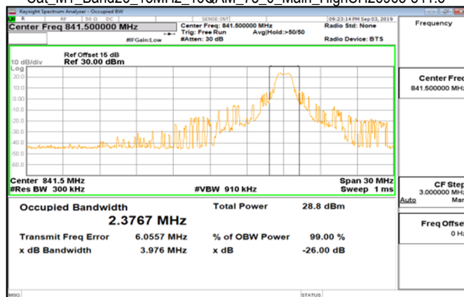
Cat_M1_Band26_15MHz_16QAM_75_0_Main_HighCH26965-841.5
