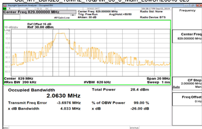
Cat_M1_Band26_10MHz_16QAM_50_0_Main_LowCH26840-829
