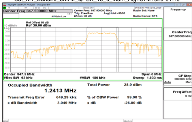
Cat_M1_Band26_3MHz_QPSK_15_0_Main_HighCH27025-847.5
