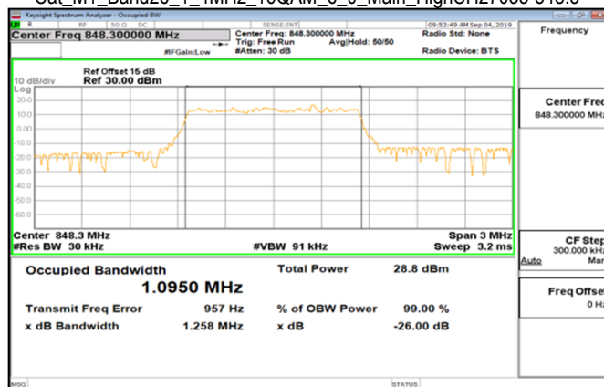
Cat_M1_Band26_1_4MHz_16QAM_6_0_Main_HighCH27033-848.3
