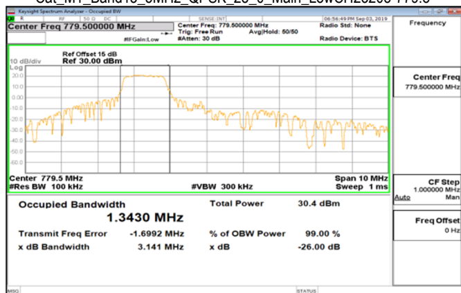
Cat_M1_Band13_5MHz_QPSK_25_0_Main_LowCH23205-779.5
