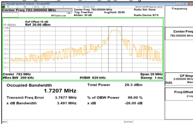
Cat_M1_Band13_10MHz_QPSK_50_0_Main_HighCH23230-782
