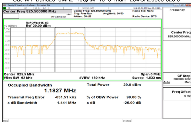
Cat_M1_Band26_3MHz_16QAM_15_0_Main_LowCH26805-825.5
