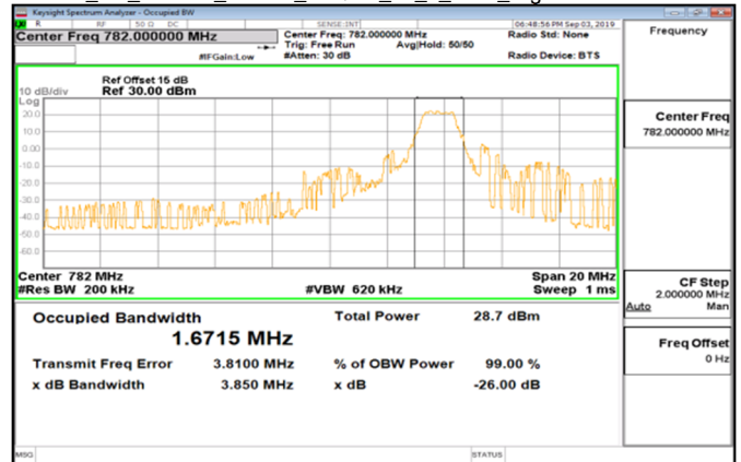
Cat_M1_Band13_10MHz_16QAM_50_0_Main_HighCH23230-782
