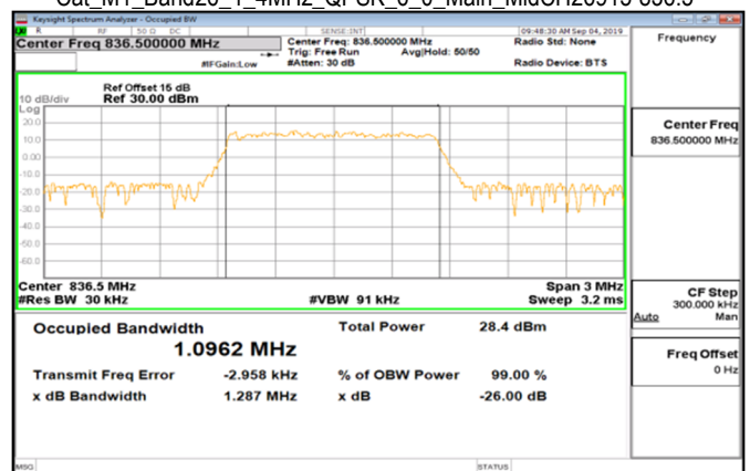
Cat_M1_Band26_1_4MHz_QPSK_6_0_Main_MidCH26915-836.5
