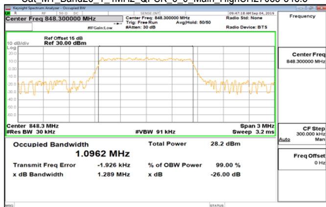
Cat_M1_Band26_1_4MHz_QPSK_6_0_Main_HighCH27033-848.3
