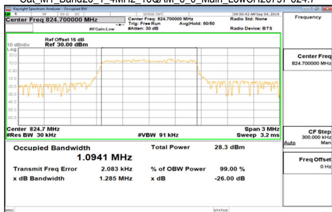
Cat_M1_Band26_1_4MHz_16QAM_6_0_Main_LowCH26797-824.7
