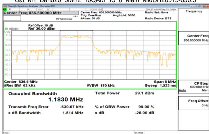
Cat_M1_Band26_3MHz_16QAM_15_0_Main_MidCH26915-836.5
