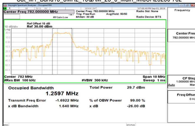
Cat_M1_Band13_5MHz_16QAM_25_0_Main_MidCH23230-782
