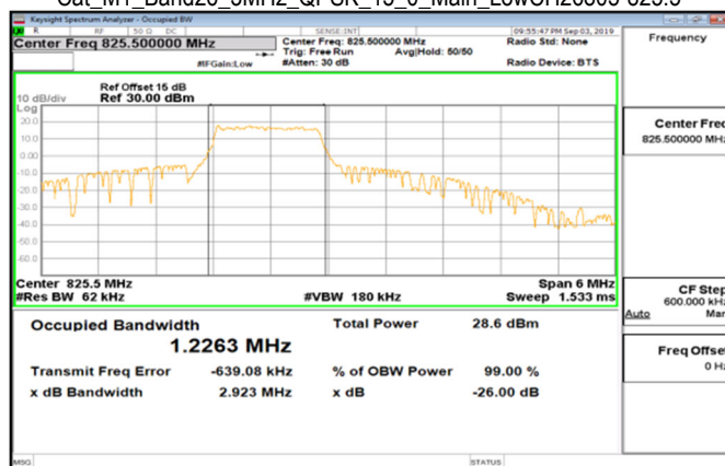
Cat_M1_Band26_3MHz_QPSK_15_0_Main_LowCH26805-825.5
