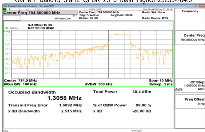
Cat_M1_Band13_5MHz_QPSK_25_0_Main_HighCH23255-784.5
