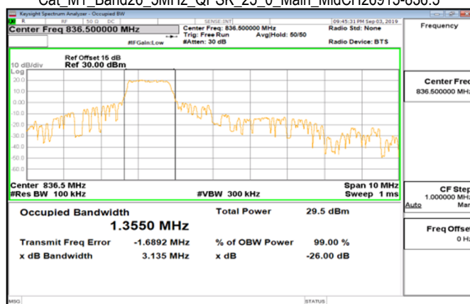
Cat_M1_Band26_5MHz_QPSK_25_0_Main_MidCH26915-836.5
