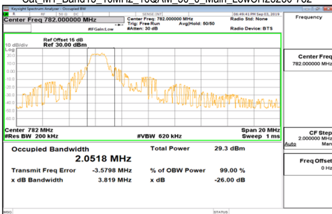
Cat_M1_Band13_10MHz_16QAM_50_0_Main_LowCH23230-782
