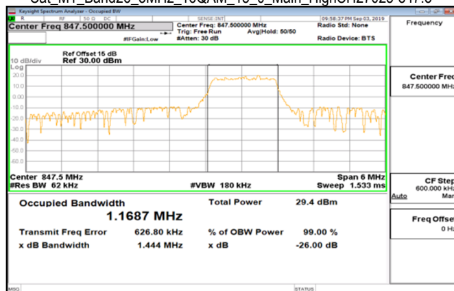
Cat_M1_Band26_3MHz_16QAM_15_0_Main_HighCH27025-847.5
