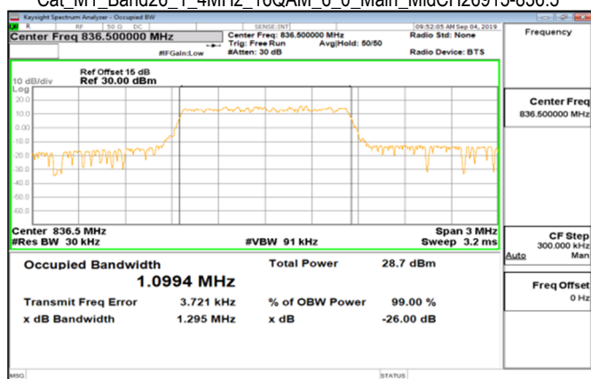
Cat_M1_Band26_1_4MHz_16QAM_6_0_Main_MidCH26915-836.5
