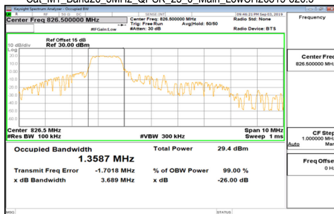
Cat_M1_Band26_5MHz_QPSK_25_0_Main_LowCH26815-826.5
