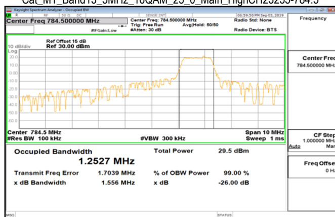
Cat_M1_Band13_5MHz_16QAM_25_0_Main_HighCH23255-784.5
