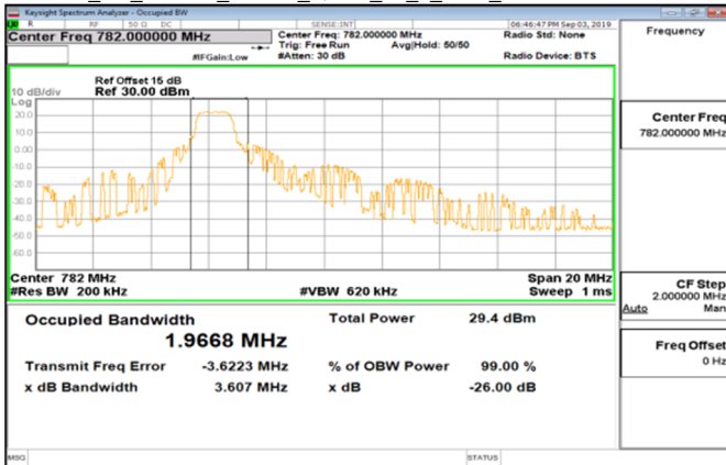
Cat_M1_Band13_10MHz_QPSK_50_0_Main_LowCH23230-782
