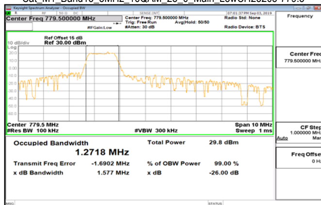
Cat_M1_Band13_5MHz_16QAM_25_0_Main_LowCH23205-779.5
