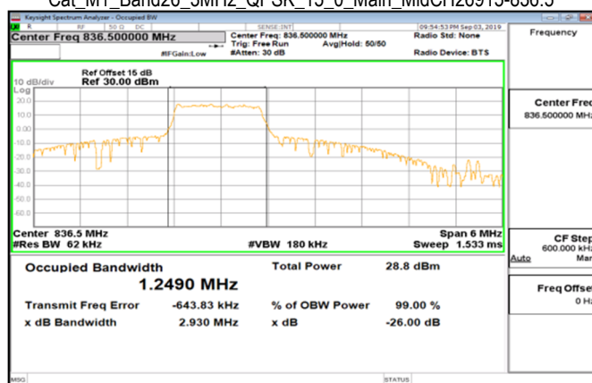
Cat_M1_Band26_3MHz_QPSK_15_0_Main_MidCH26915-836.5
