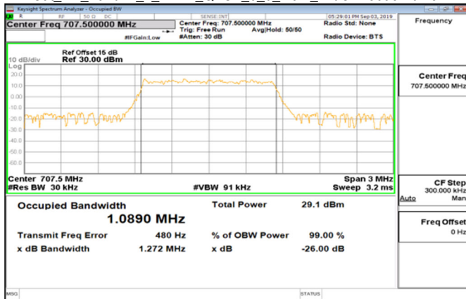
Cat_M1_Band12_1_4MHz_QPSK_6_0_Main_MidCH23095-707.5
