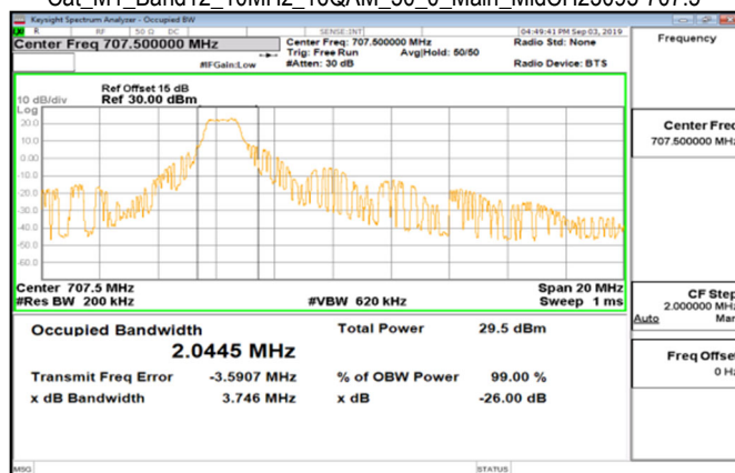
Cat_M1_Band12_10MHz_16QAM_50_0_Main_MidCH23095-707.5
