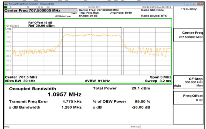
Cat_M1_Band12_1_4MHz_16QAM_6_0_Main_MidCH23095-707.5
