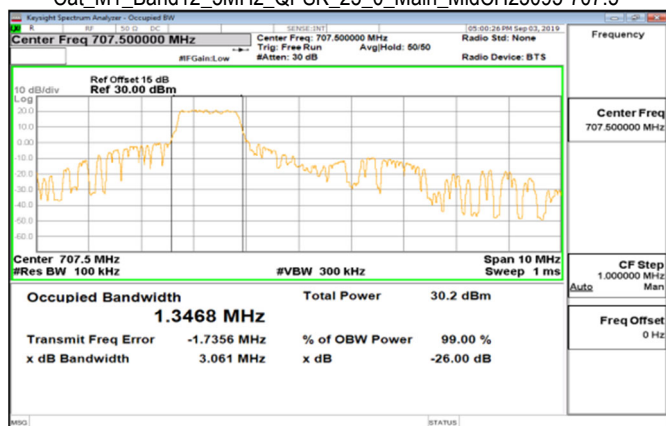
Cat_M1_Band12_5MHz_QPSK_25_0_Main_MidCH23095-707.5
