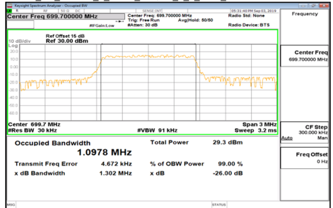
Cat_M1_Band12_1_4MHz_16QAM_6_0_Main_LowCH23017-699.7
