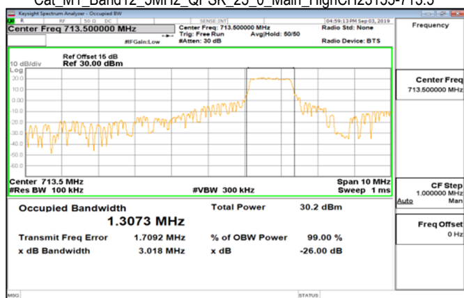
Cat_M1_Band12_5MHz_QPSK_25_0_Main_HighCH23155-713.5
