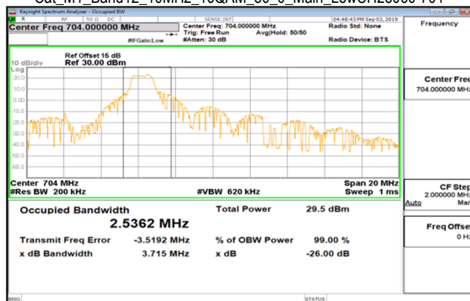
Cat_M1_Band12_10MHz_16QAM_50_0_Main_LowCH23060-704
