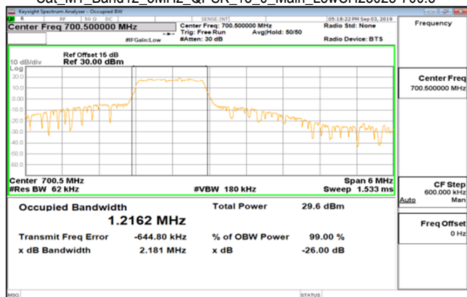
Cat_M1_Band12_3MHz_QPSK_15_0_Main_LowCH23025-700.5
