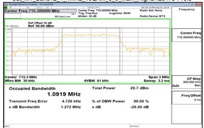
Cat_M1_Band12_1_4MHz_16QAM_6_0_Main_HighCH23173-715.3
