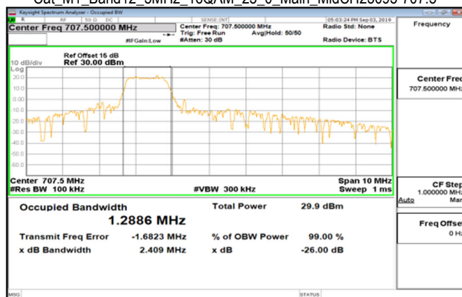
Cat_M1_Band12_5MHz_16QAM_25_0_Main_MidCH23095-707.5
