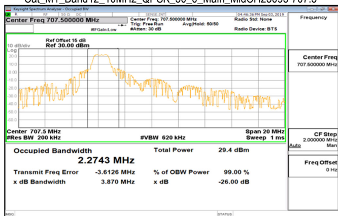
Cat_M1_Band12_10MHz_QPSK_50_0_Main_MidCH23095-707.5
