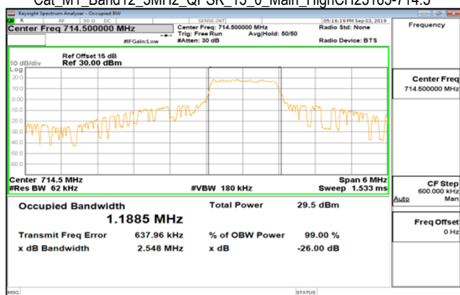
Cat_M1_Band12_3MHz_QPSK_15_0_Main_HighCH23165-714.5
