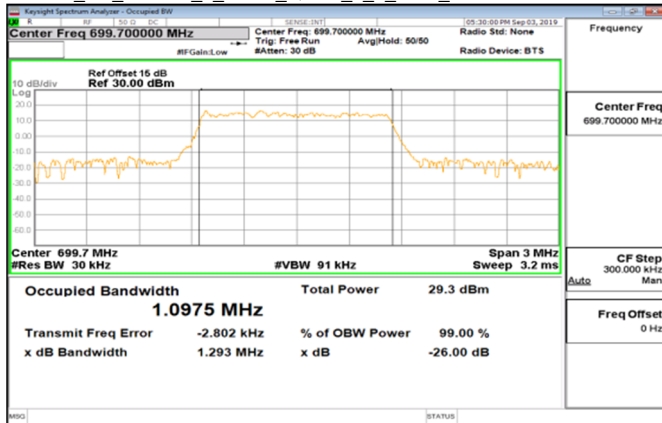
Cat_M1_Band12_1_4MHz_QPSK_6_0_Main_LowCH23017-699.7
