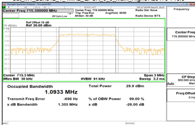
Cat_M1_Band12_1_4MHz_QPSK_6_0_Main_HighCH23173-715.3
