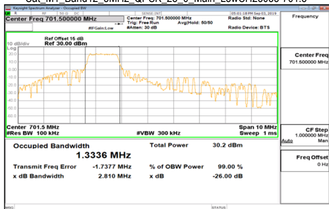
Cat_M1_Band12_5MHz_QPSK_25_0_Main_LowCH23035-701.5
