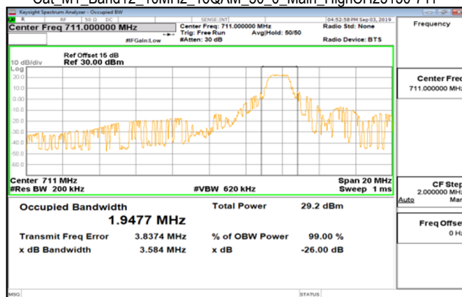
Cat_M1_Band12_10MHz_16QAM_50_0_Main_HighCH23130-711
