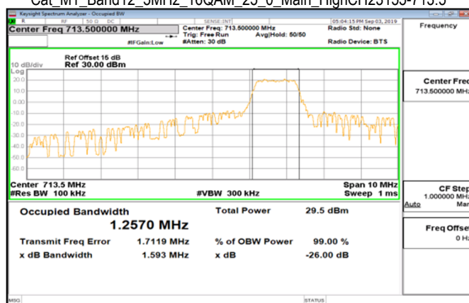
Cat_M1_Band12_5MHz_16QAM_25_0_Main_HighCH23155-713.5
