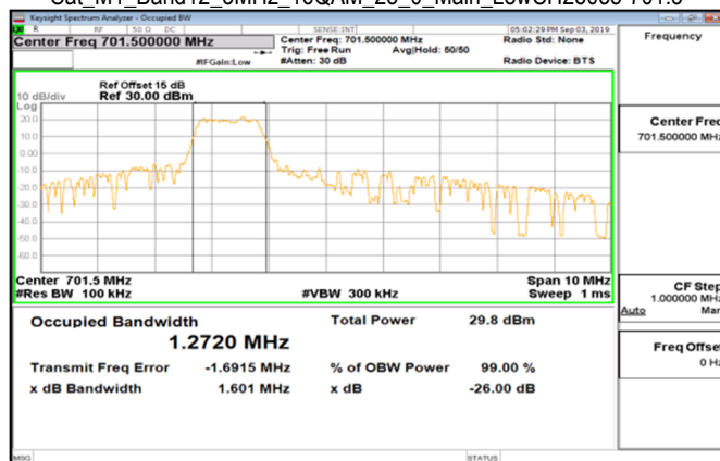
Cat_M1_Band12_5MHz_16QAM_25_0_Main_LowCH23035-701.5
