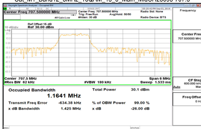
Cat_M1_Band12_3MHz_16QAM_15_0_Main_MidCH23095-707.5
