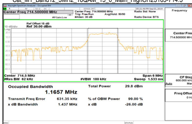
Cat_M1_Band12_3MHz_16QAM_15_0_Main_HighCH23165-714.5
