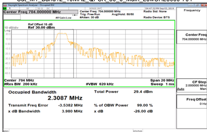
Cat_M1_Band12_10MHz_QPSK_50_0_Main_LowCH23060-704
