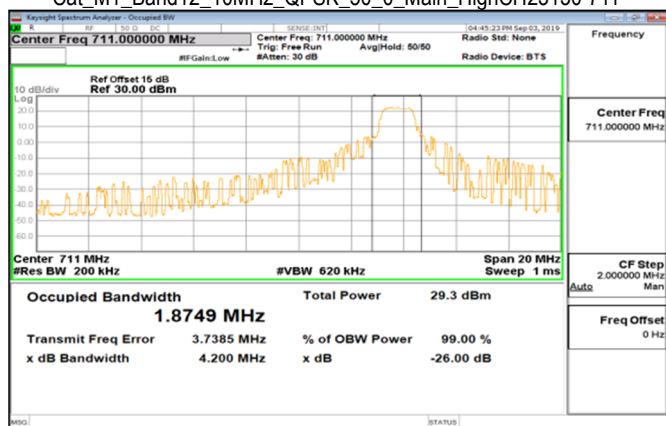
Cat_M1_Band12_10MHz_QPSK_50_0_Main_HighCH23130-711
