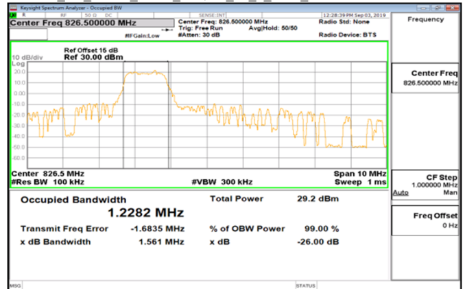
Cat_M1_Band5_5MHz_16QAM_25_0_Main_LowCH20425-826.5
