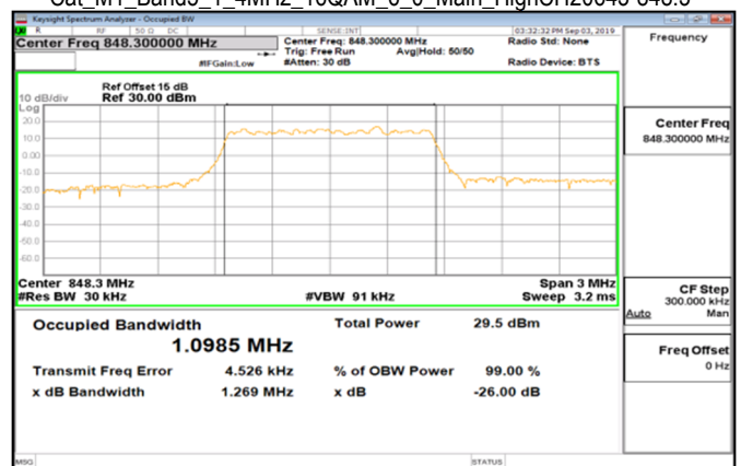
Cat_M1_Band5_1_4MHz_16QAM_6_0_Main_HighCH20643-848.3
