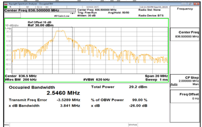
Cat_M1_Band5_10MHz_16QAM_50_0_Main_MidCH20525-836.5
