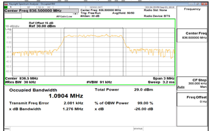
Cat_M1_Band5_1_4MHz_16QAM_6_0_Main_MidCH20525-836.5
