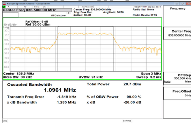
Cat_M1_Band5_1_4MHz_QPSK_6_0_Main_MidCH20525-836.5
