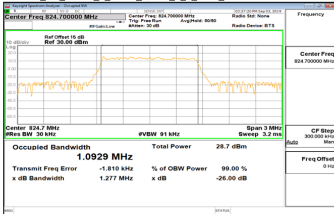
Cat_M1_Band5_1_4MHz_QPSK_6_0_Main_LowCH20407-824.7
