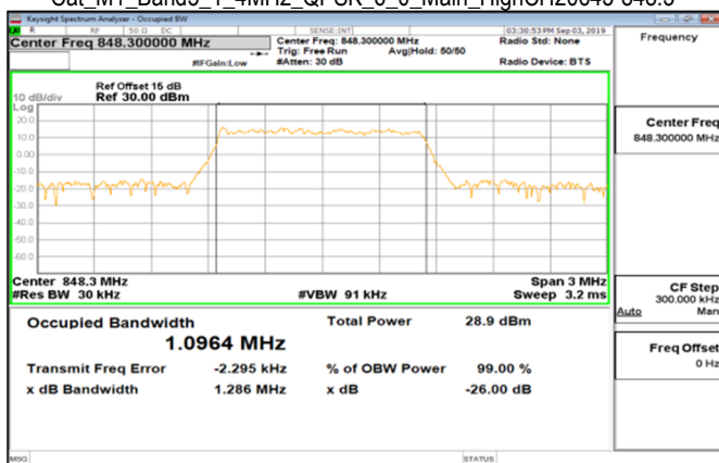
Cat_M1_Band5_1_4MHz_QPSK_6_0_Main_HighCH20643-848.3
