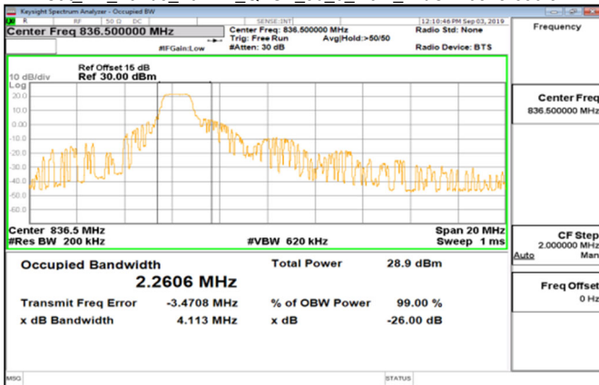
Cat_M1_Band5_10MHz_QPSK_50_0_Main_MidCH20525-836.5
