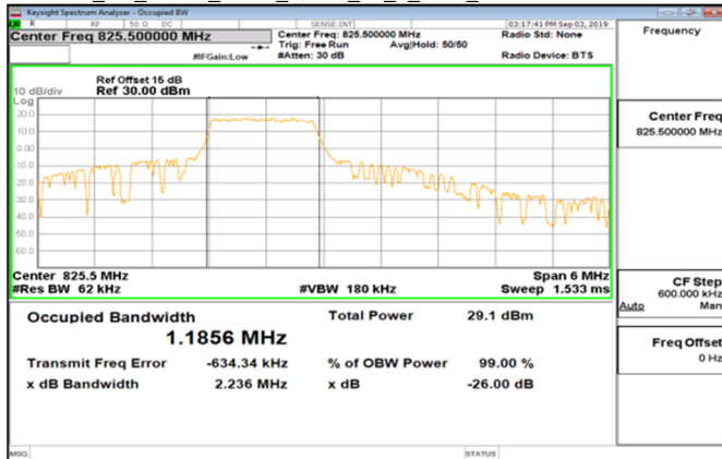
Cat_M1_Band5_3MHz_QPSK_15_0_Main_LowCH20415-825.5
