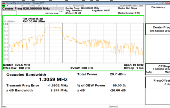
Cat_M1_Band5_5MHz_QPSK_25_0_Main_LowCH20425-826.5
