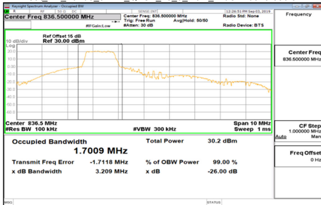
Cat_M1_Band5_5MHz_QPSK_25_0_Main_MidCH20525-836.5
