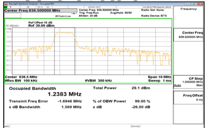
Cat_M1_Band5_5MHz_16QAM_25_0_Main_MidCH20525-836.5
