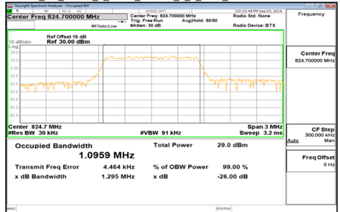
Cat_M1_Band5_1_4MHz_16QAM_6_0_Main_LowCH20407-824.7
