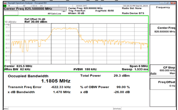
Cat_M1_Band5_3MHz_16QAM_15_0_Main_LowCH20415-825.5
