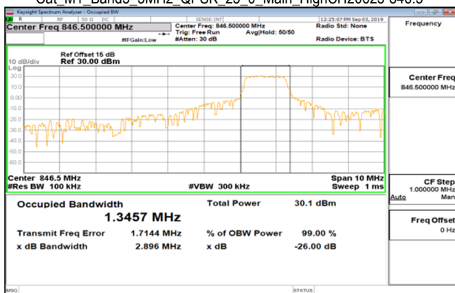
Cat_M1_Band5_5MHz_QPSK_25_0_Main_HighCH20625-846.5
