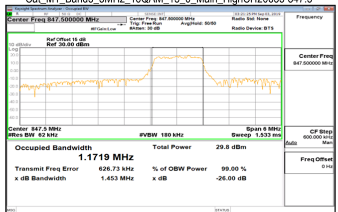
Cat_M1_Band5_3MHz_16QAM_15_0_Main_HighCH20635-847.5
