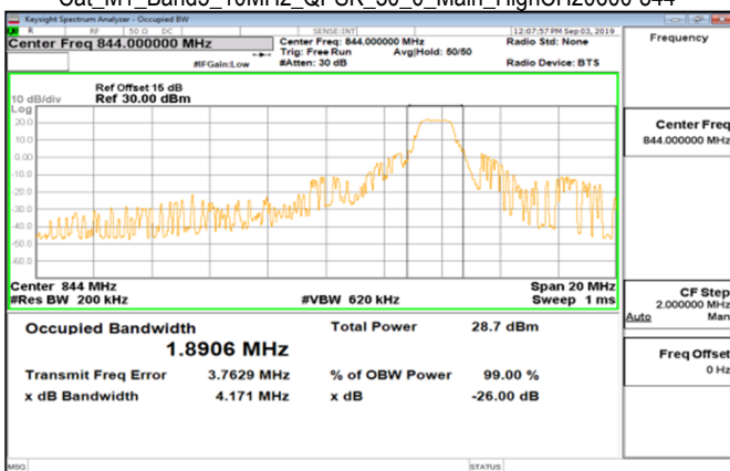
Cat_M1_Band5_10MHz_QPSK_50_0_Main_HighCH20600-844
