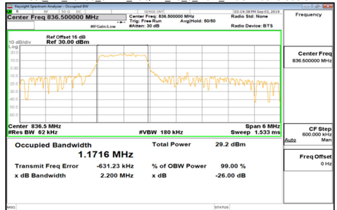
Cat_M1_Band5_3MHz_16QAM_15_0_Main_MidCH20525-836.5
