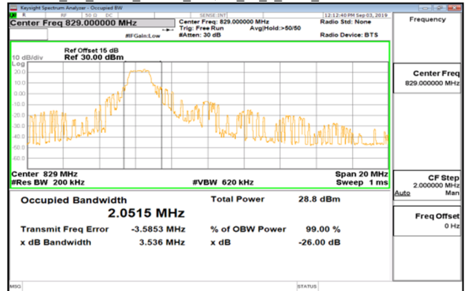
Cat_M1_Band5_10MHz_16QAM_50_0_Main_LowCH20450-829
