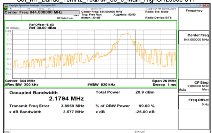
Cat_M1_Band5_10MHz_16QAM_50_0_Main_HighCH20600-844
