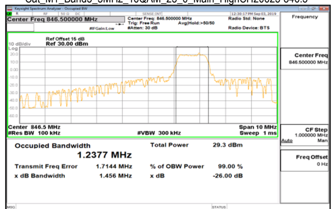
Cat_M1_Band5_5MHz_16QAM_25_0_Main_HighCH20625-846.5
