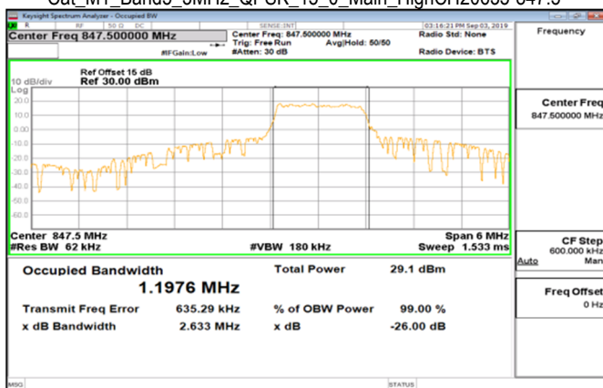
Cat_M1_Band5_3MHz_QPSK_15_0_Main_HighCH20635-847.5
