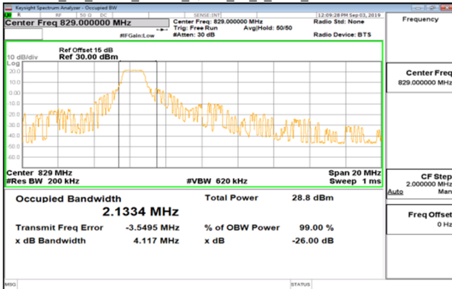
Cat_M1_Band5_10MHz_QPSK_50_0_Main_LowCH20450-829
