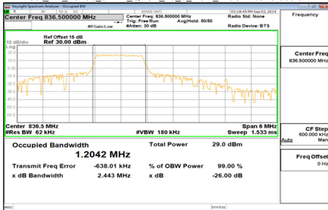
Cat_M1_Band5_3MHz_QPSK_15_0_Main_MidCH20525-836.5
