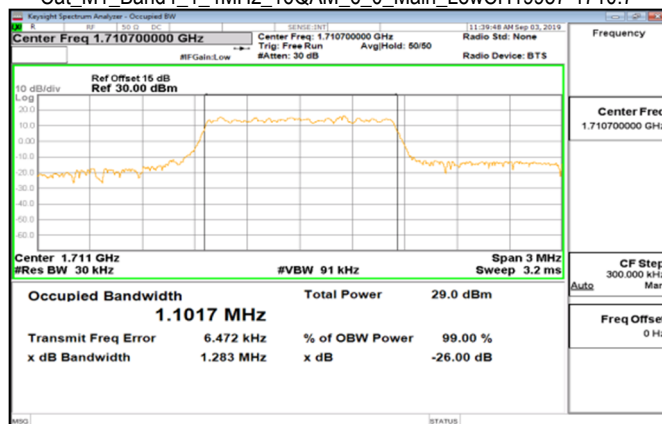
Cat M1_Band4_1_4MHz_16QAM_6_0_Main_LowCH19957-1710.7
