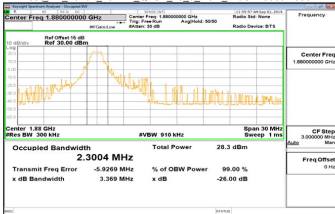
Cat M1_Band2_15MHz_QPSK_75_0_Main_MidCH18900-1880
