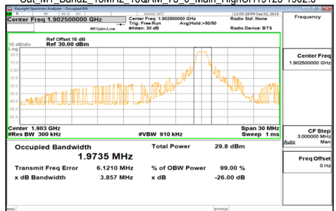
Cat M1_Band2_15MHz_16QAM_75_0_Main_HighCH19125-1902.5
