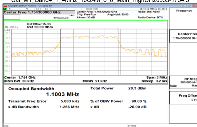
Cat M1_Band4_1_4MHz_16QAM_6_0_Main_HighCH20393-1754.3
