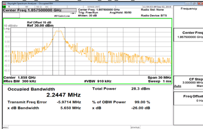
Cat M1_Band2_15MHz_QPSK_75_0_Main_LowCH18675-1857.5
