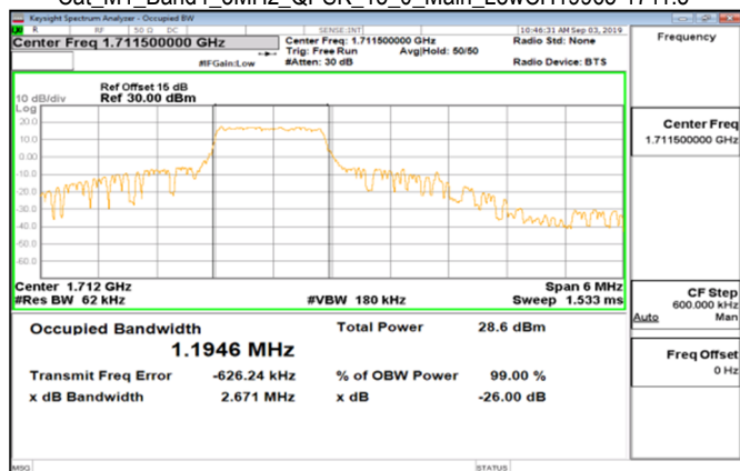
Cat_M1_Band4_3MHz_QPSK_15_0_Main_LowCH19965-1711.5
