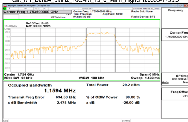
Cat_M1_Band4_3MHz_16QAM_15_0_Main_HighCH20385-1753.5
