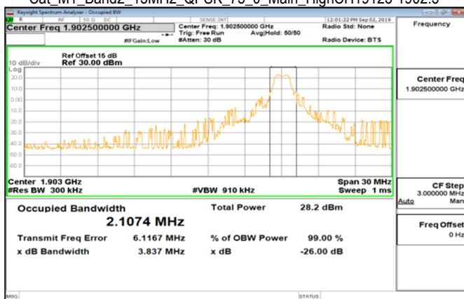
Cat M1_Band2_15MHz_QPSK_75_0_Main_HighCH19125-1902.5
