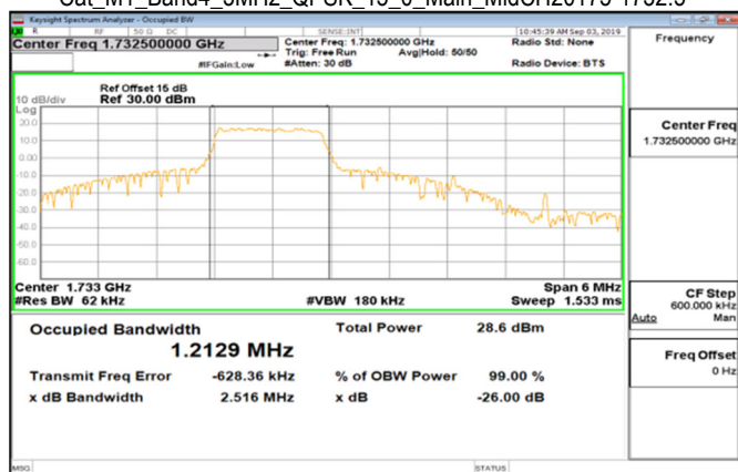
Cat_M1_Band4_3MHz_QPSK_15_0_Main_MidCH20175-1732.5
