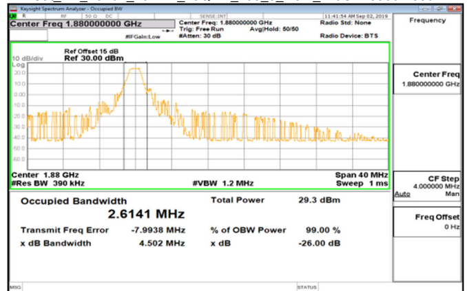
Cat M1_Band2_20MHz_16QAM_100_0_Main_MidCH18900-1880
