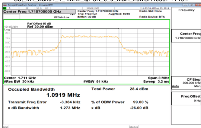
Cat M1_Band4_1_4MHz_QPSK_6_0_Main_LowCH19957-1710.7
