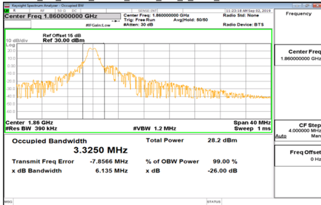
Cat M1_Band2_20MHz_QPSK_100_0_Main_LowCH18700-1860
