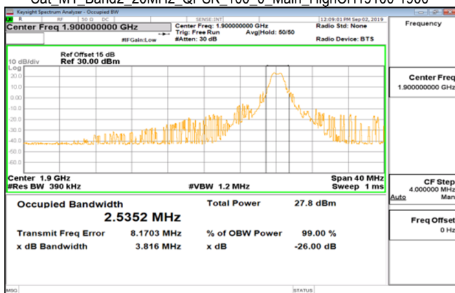
Cat M1_Band2_20MHz_QPSK_100_0_Main_HighCH19100-1900
