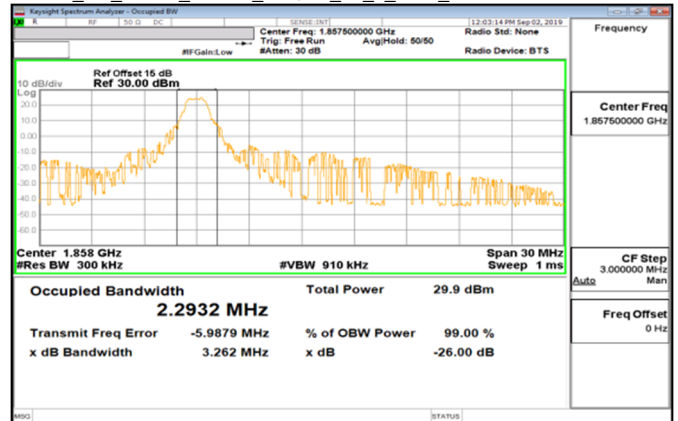
Cat M1_Band2_15MHz_16QAM_75_0_Main_LowCH18675-1857.5
