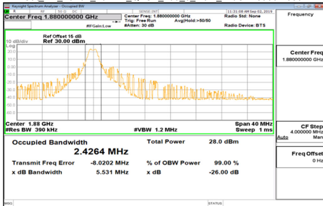
Cat M1_Band2_20MHz_QPSK_100_0_Main_MidCH18900-1880
