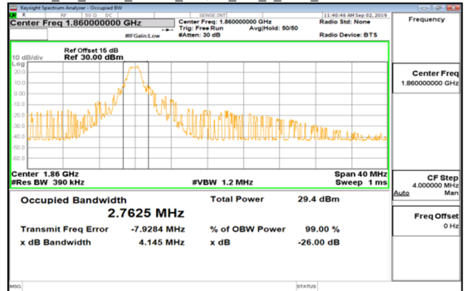
Cat M1_Band2_20MHz_16QAM_100_0_Main_LowCH18700-1860
