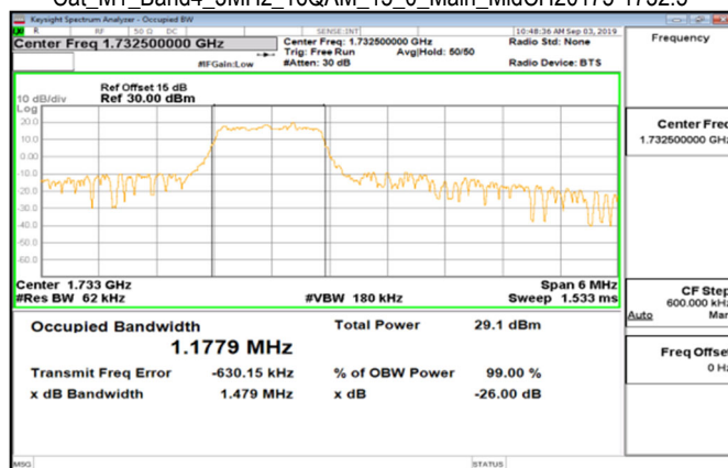
Cat_M1_Band4_3MHz_16QAM_15_0_Main_MidCH20175-1732.5
