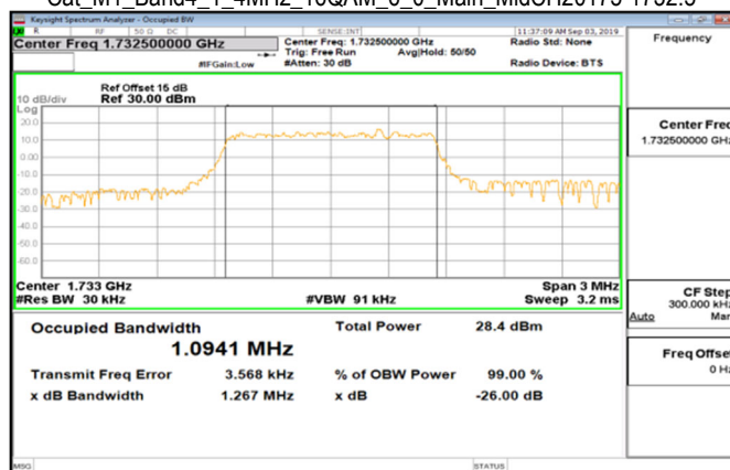
Cat M1_Band4_1_4MHz_16QAM_6_0_Main_MidCH20175-1732.5
