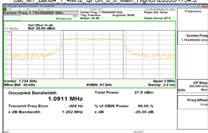
Cat M1_Band4_1_4MHz_QPSK_6_0_Main_HighCH20393-1754.3
