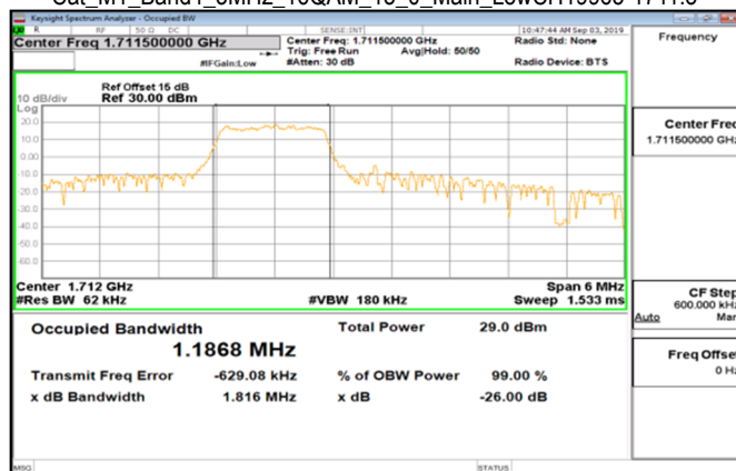
Cat_M1_Band4_3MHz_16QAM_15_0_Main_LowCH19965-1711.5
