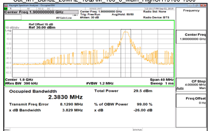
Cat M1_Band2_20MHz_16QAM_100_0_Main_HighCH19100-1900
