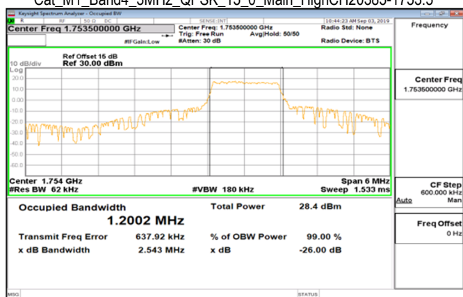
Cat_M1_Band4_3MHz_QPSK_15_0_Main_HighCH20385-1753.5
