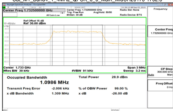
Cat M1_Band4_1_4MHz_QPSK_6_0_Main_MidCH20175-1732.5
