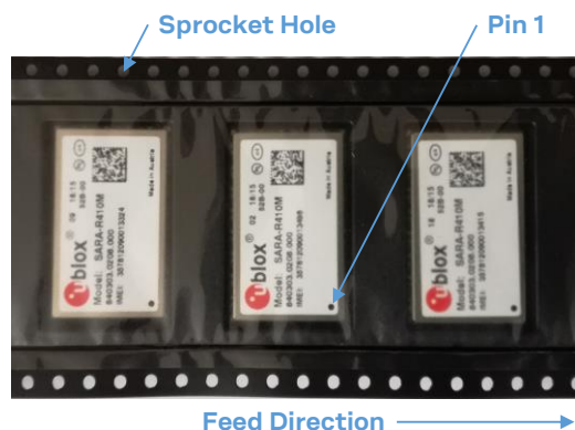
Figure 5: Orientation of SARA-R4/N4 series modules on tape
