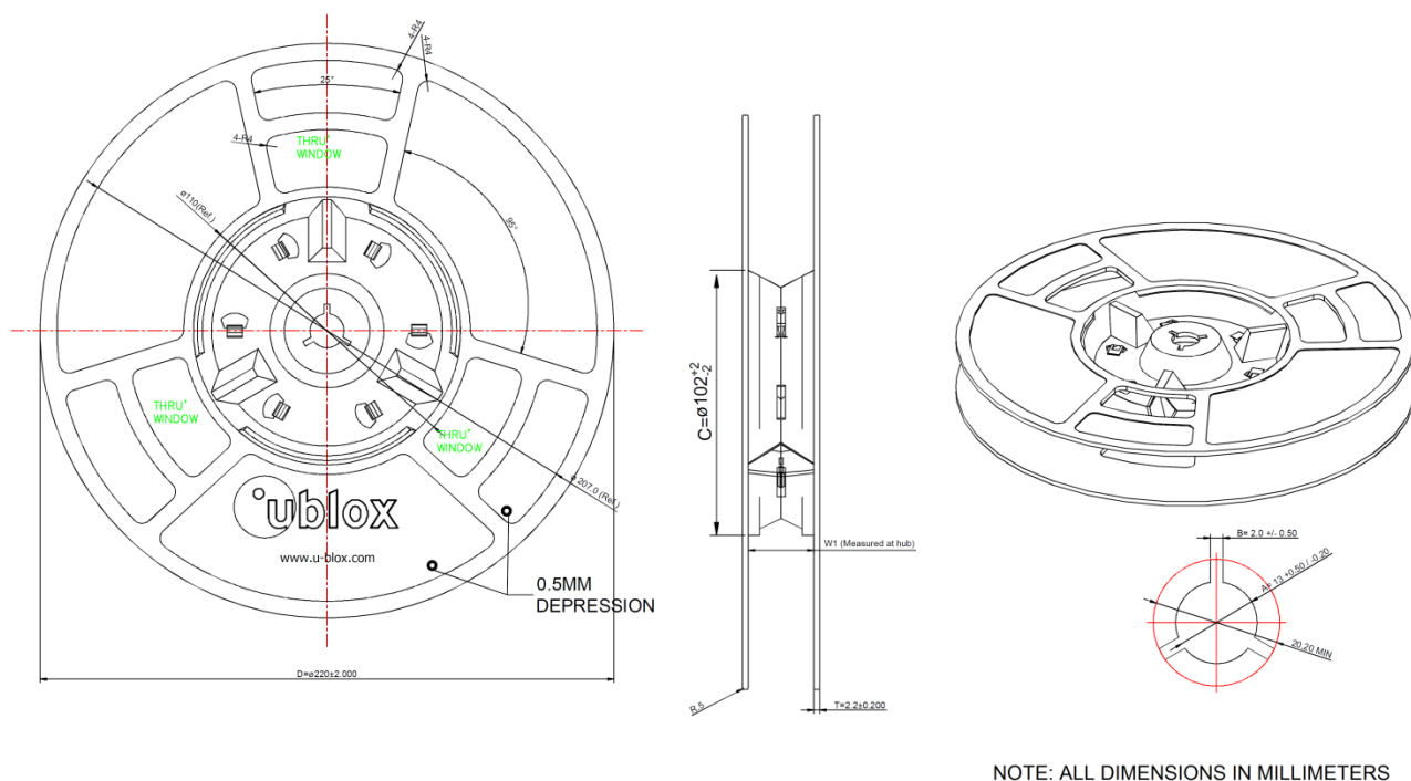
Figure 4: SARA-R4/N4 series modules reel
