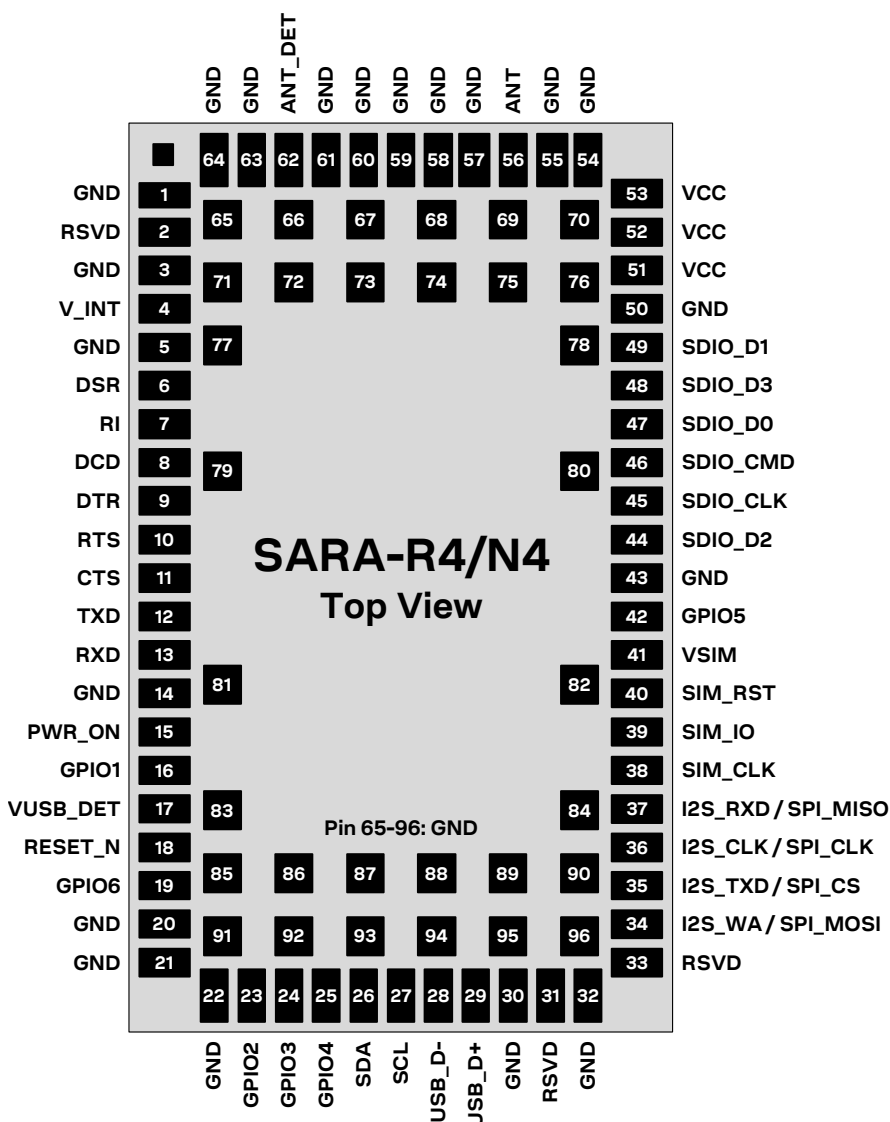
Figure 2: SARA-R4/N4 series pin assignment (top view)
