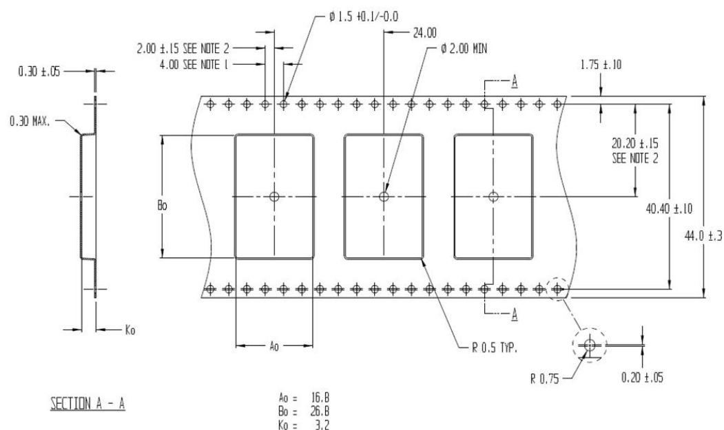
Figure 6: SARA-R4/N4 series modules tape
