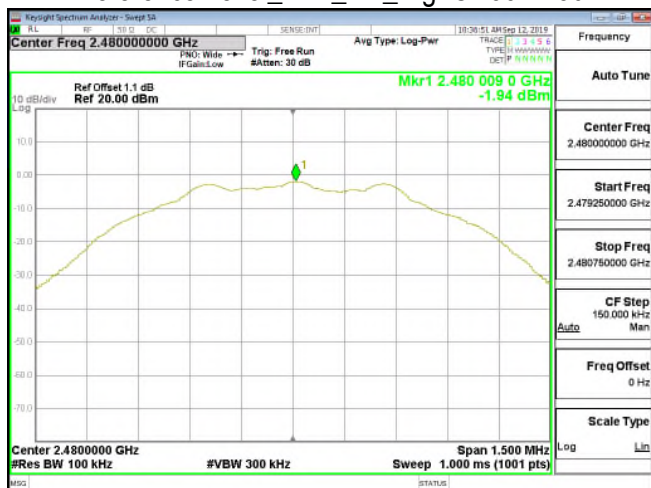
Reference Level_BLE_1M_HighCH39-2480
