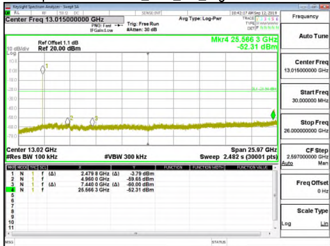
Spurious Emission_BLE_1M_HighCH39-2480
