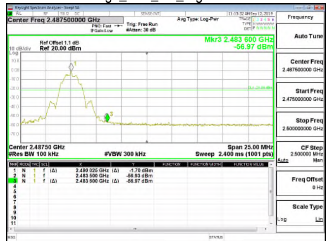
Band Edge_BLE_2M_HighCH39-2480
