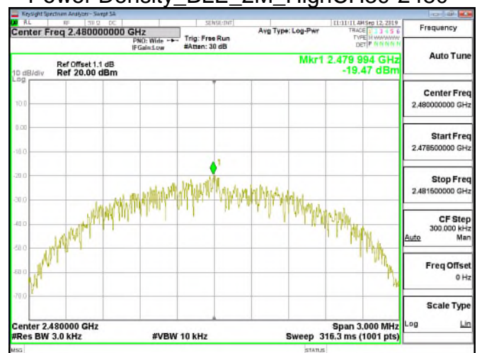
Power Density_BLE_2M_HighCH39-2480
