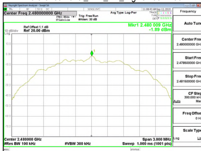
Reference Level_BLE_2M_HighCH39-2480
