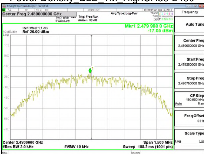
Power Density_BLE_1M_HighCH39-2480
