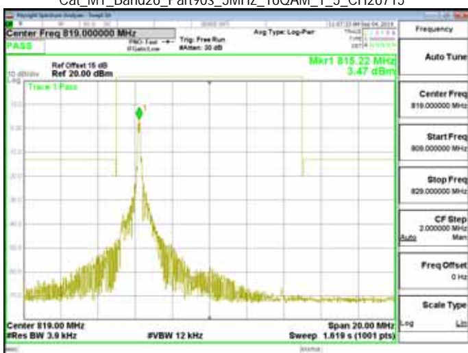
Cat_M1_Band26_Part90s_5MHz_16QAM_1_5_CH26715
