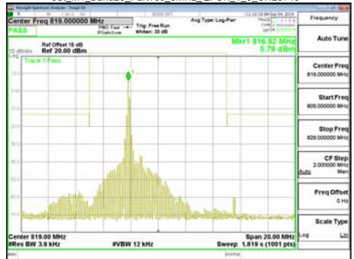
Cat_M1_Band26_Part90s_5MHz_QPSK_1_0_CH26765
