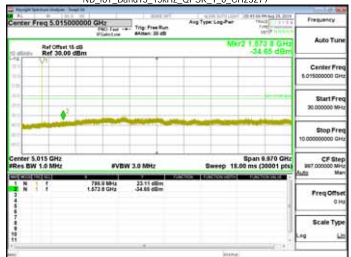
NB_IoT_Band13_15kHz_QPSK_1_0_CH23279
