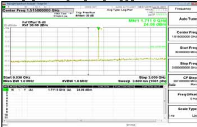
Cat_M1_30MHz-3GHz_Band4_15MHz_QPSK_1_0_LowCH20025-1717.5
