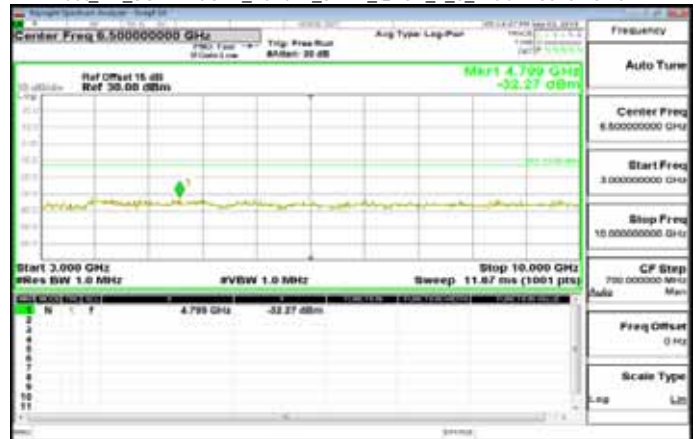
Cat_M1_3GHz-10GHz_Band12_3MHz_QPSK_1_0_MidCH23095-707.5
