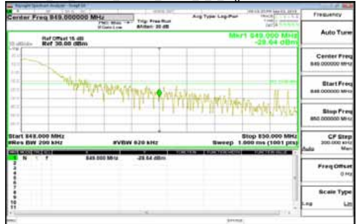
Cat_M1_Band26_15MHz_QPSK_1_5_HighCH26965-841.5
