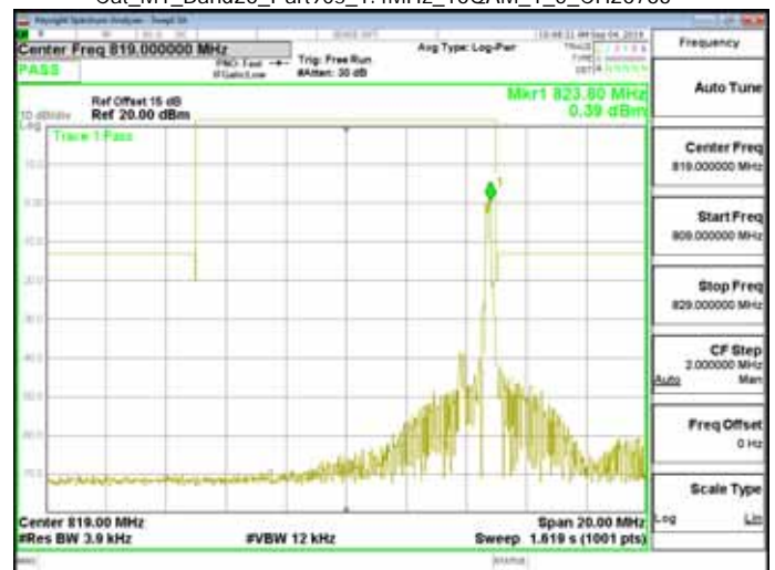
Cat_M1_Band26_Part90s_1.4MHz_16QAM_6_0_CH26697
