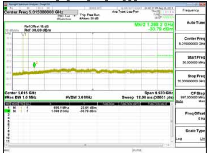
NB_IoT_Band12_15kHz_QPSK_1_0_CH23095
