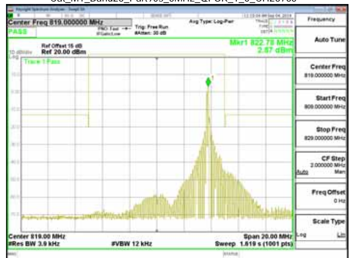
Cat_M1_Band26_Part90s_5MHz_QPSK_1_5_CH26715
