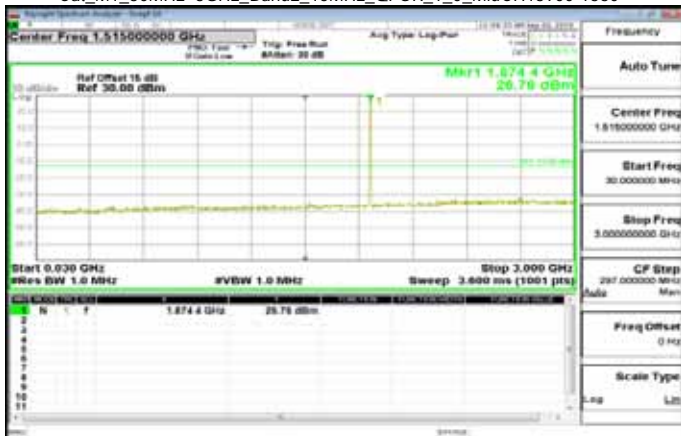
Cat_M1_30MHz-3GHz_Band2_15MHz_QPSK_1_0_MidCH18900-1880
