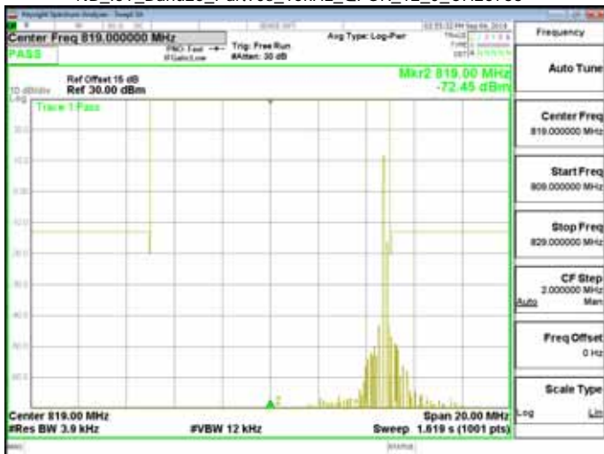
Cat_M1_Band26_Part90s_1.4MHz_QPSK_1_0_CH26697
