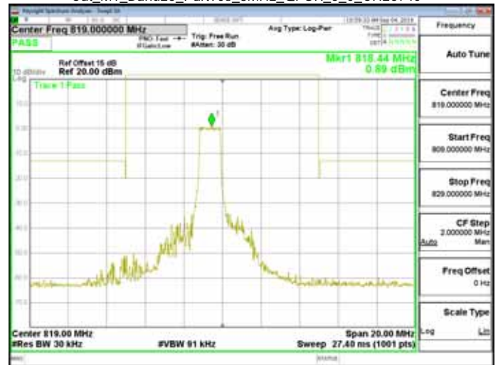
Cat_M1_Band26_Part90s_3MHz_QPSK_6_0_CH26775
