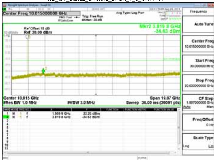
NB_IoT_Band2_3.75kHz_BPSK_1_0_CH19199
