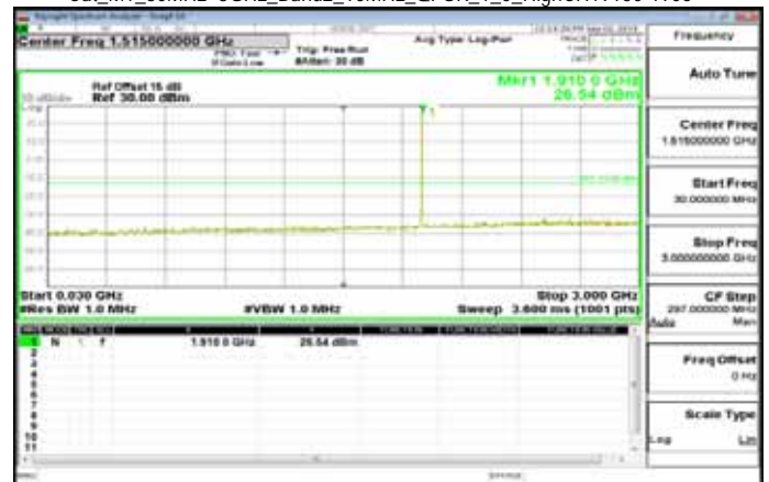
Cat_M1_30MHz-3GHz_Band2_10MHz_QPSK_1_0_HighCH19150-1905
