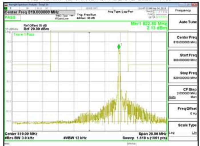
Cat_M1_Band26_Part90s_1.4MHz_QPSK_1_5_CH26697
