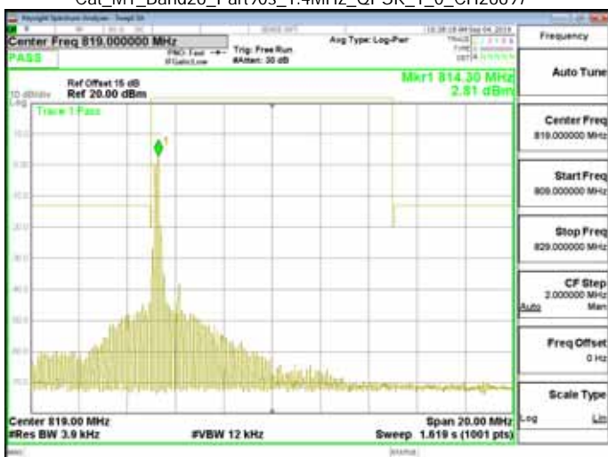
Cat_M1_Band26_Part90s_1.4MHz_QPSK_1_0_CH26697
