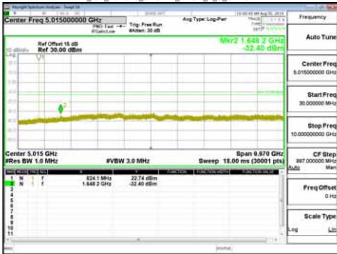
NB_IoT_Band26_3.75kHz_BPSK_1_0_CH26915
