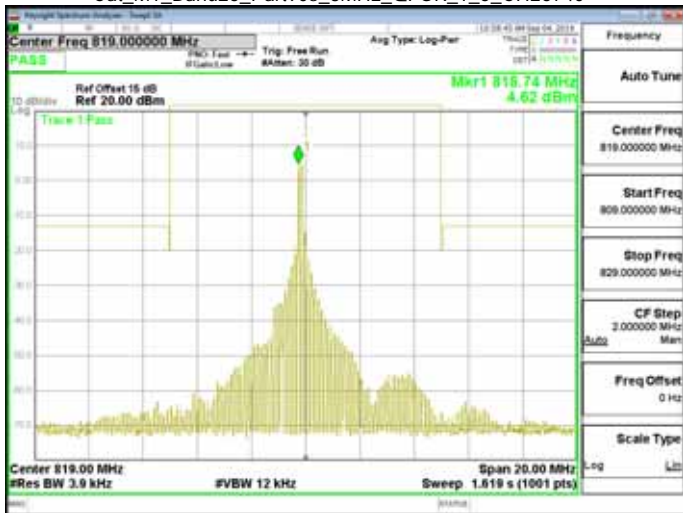
Cat_M1_Band26_Part90s_3MHz_QPSK_1_5_CH26775
