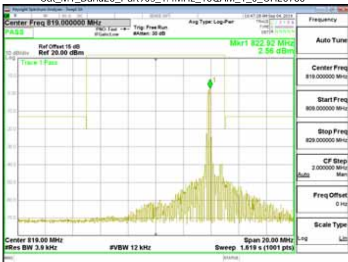
Cat_M1_Band26_Part90s_1.4MHz_16QAM_1_5_CH26697
