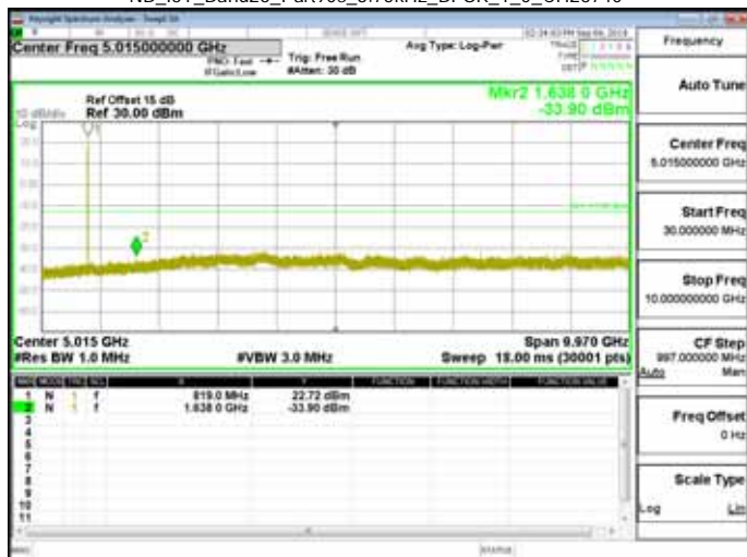
NB_IoT_Band26_Part90s_3.75kHz_BPSK_1_0_CH26788
