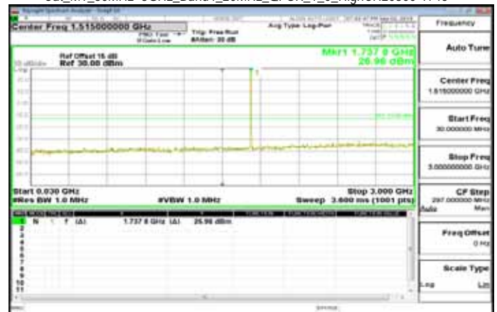
Cat_M1_30MHz-3GHz_Band4_20MHz_QPSK_1_0_HighCH20300-1745
