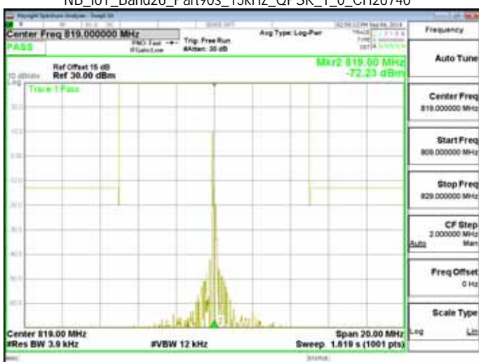
NB_IoT_Band26_Part90s_15kHz_QPSK_1_0_CH26740
