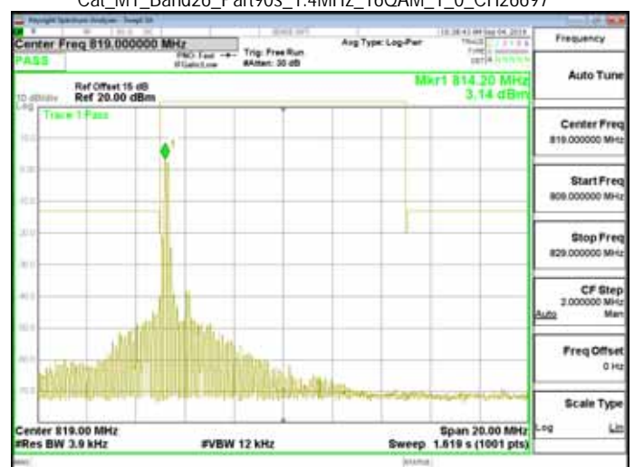
Cat_M1_Band26_Part90s_1.4MHz_16QAM_1_0_CH26697
