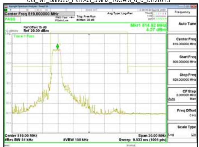
Cat_M1_Band26_Part90s_5MHz_16QAM_6_0_CH26715
