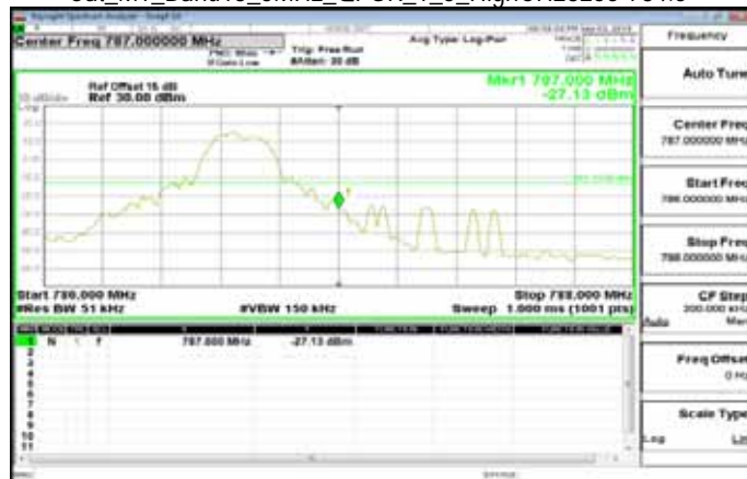
Cat_M1_Band13_5MHz_QPSK_1_5_HighCH23255-784.5
