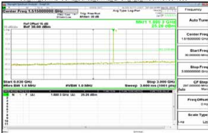
Cat_M1_30MHz-3GHz_Band2_3MHz_OPSK_1_0_MidCH18900-1880
