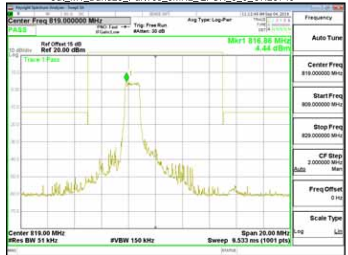
Cat_M1_Band26_Part90s_5MHz_QPSK_6_0_CH26765
