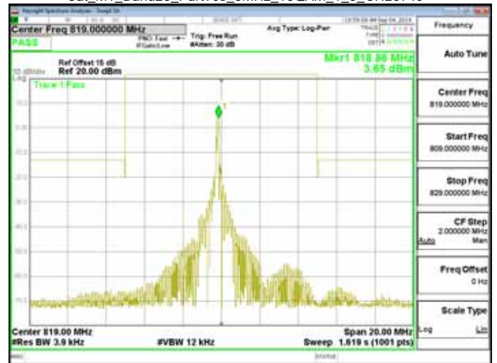
Cat_M1_Band26_Part90s_3MHz_16QAM_1_5_CH26775
