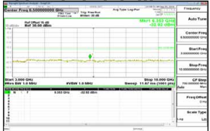
Cat_M1_3GHz-10GHz_Band26_Part90s_5MHz_QPSK_1_0_LowCH26715-816.5
