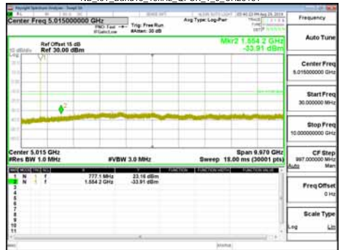
NB_IoT_Band13_15kHz_QPSK_1_0_CH23230
