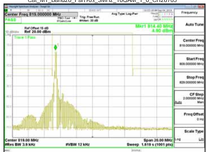
Cat_M1_Band26_Part90s_3MHz_16QAM_1_0_CH26705
