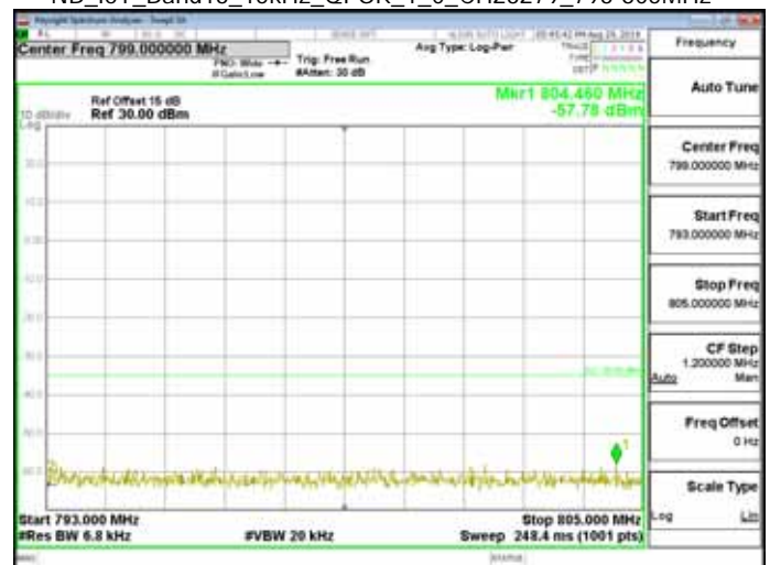
NB_IoT_Band13_15kHz_QPSK_1_0_CH23279_793-805MHz
