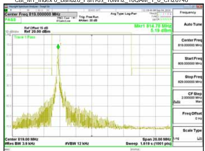
Cat_M1_Index 0_Band26_Part90s_10MHz_16QAM_1_0_CH26740
