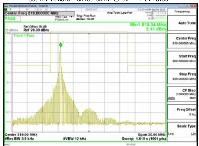
Cat_M1_Band26_Part90s_3MHz_QPSK_1_5_CH26705
