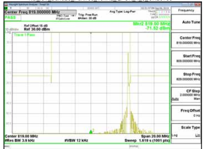
NB_IoT_Band26_Part90s_15kHz_QPSK_1_11_CH26788
