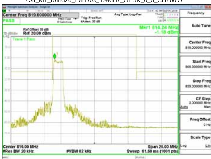
Cat_M1_Band26_Part90s_1.4MHz_QPSK_6_0_CH26697
