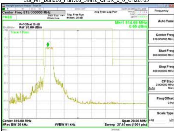
Cat_M1_Band26_Part90s_3MHz_QPSK_6_0_CH26705
