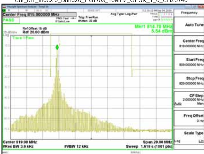
Cat_M1_Index 0_Band26_Part90s_10MHz_QPSK_1_0_CH26740
