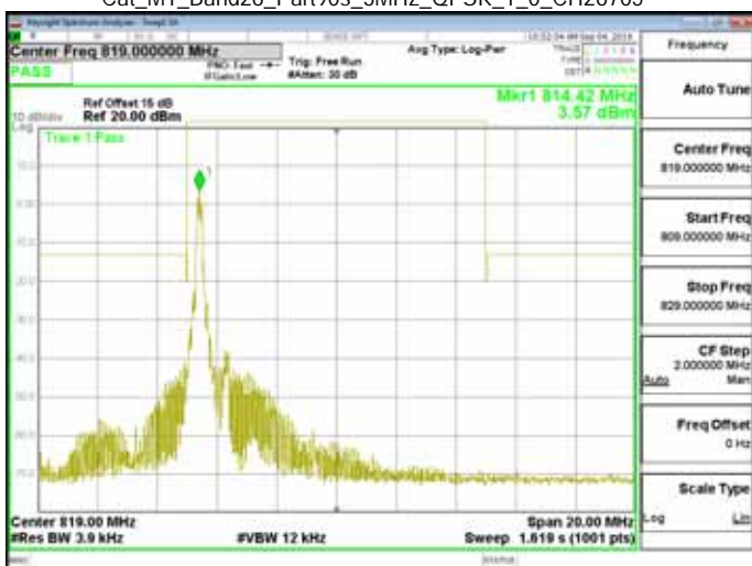
Cat_M1_Band26_Part90s_3MHz_QPSK_1_0_CH26705
