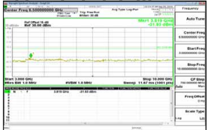
Cat_M1_3GHz-10GHz_Band26_Part90s_3MHz_QPSK_1_0_LowCH26705-815.5
