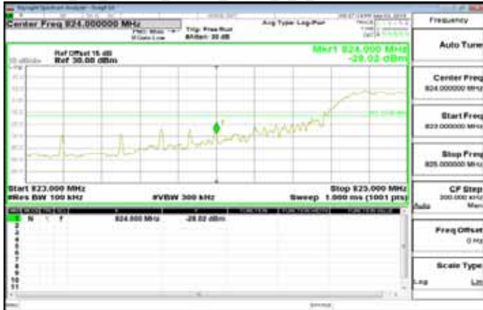
Cat_M1_Band26_10MHz_QPSK_6_0_LowCH26840-829
