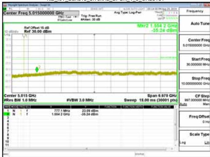
NB_IoT_Band13_3.75kHz_BPSK_1_0_CH23230
