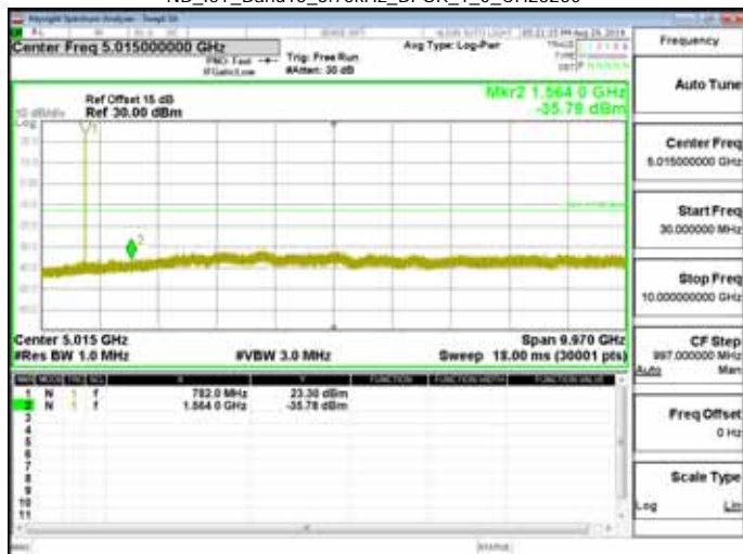
NB_IoT_Band13_3.75kHz_BPSK_1_0_CH23279
