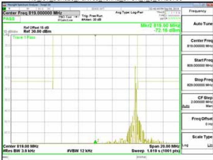
NB_IoT_Band26_Part90s_15kHz_QPSK_1_0_CH26692
