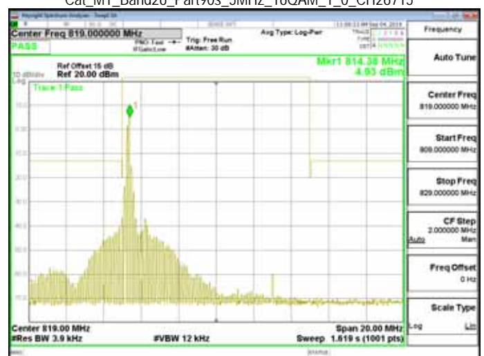
Cat_M1_Band26_Part90s_5MHz_16QAM_1_0_CH26715
