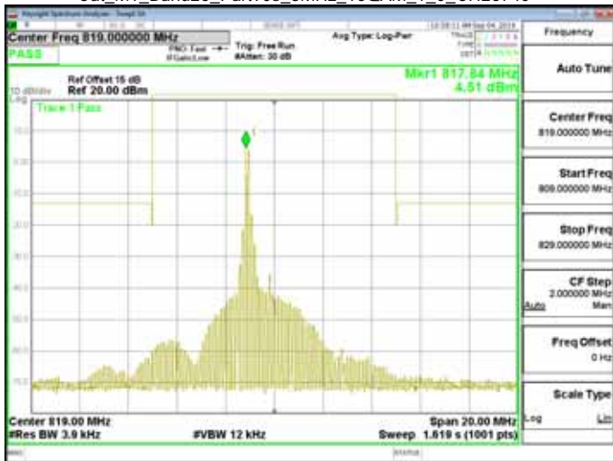
Cat_M1_Band26_Part90s_3MHz_16QAM_1_0_CH26775
