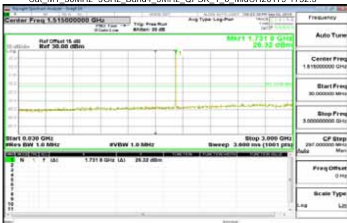
Cat_M1_30MHz-3GHz_Band4_5MHz_QPSK_1_0_MidCH20175-1732.5
