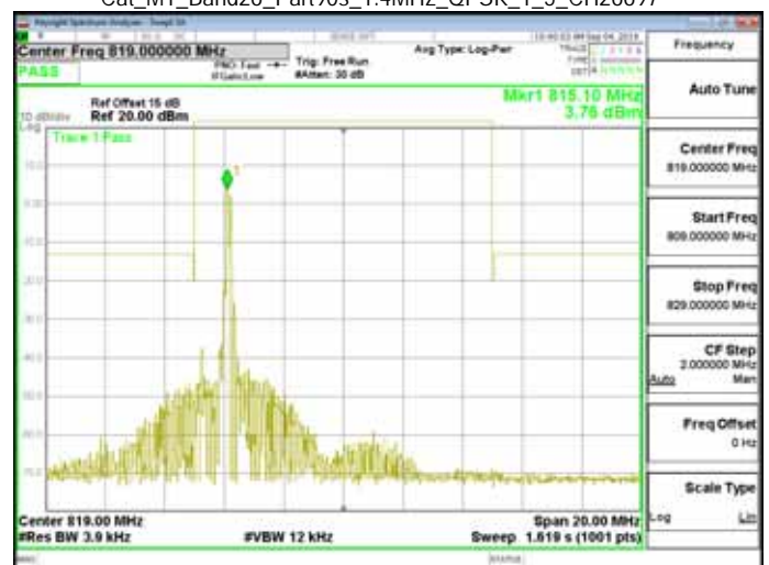
Cat_M1_Band26_Part90s_1.4MHz_QPSK_1_5_CH26697
