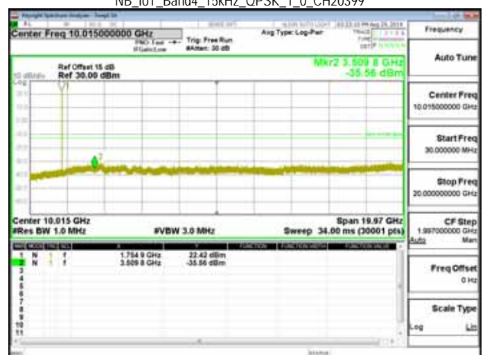
NB_IoT_Band4_15kHz_QPSK_1_0_CH20399
