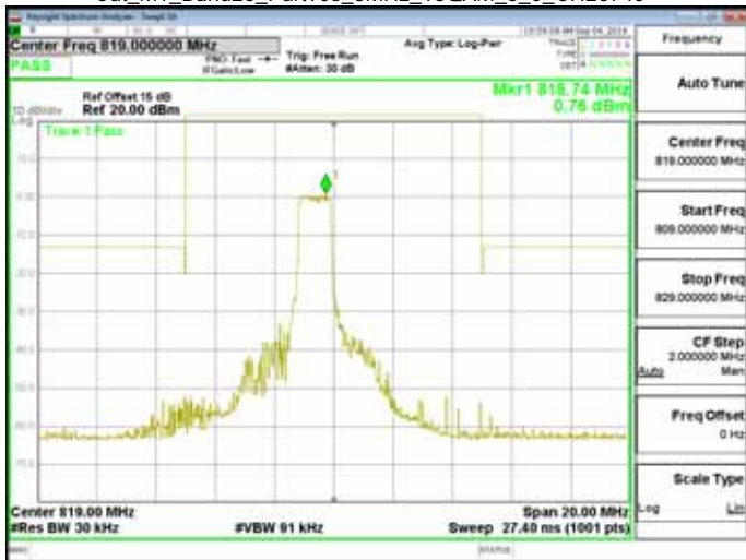
Cat_M1_Band26_Part90s_3MHz_16QAM_6_0_CH26775
