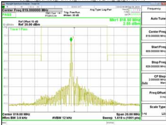
Cat_M1_Band26_Part90s_1.4MHz_16QAM_1_0_CH26783
