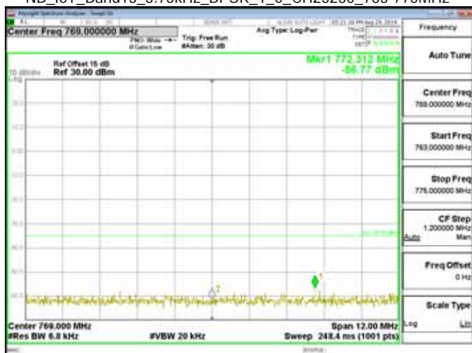
NB_IoT_Band13_3.75kHz_BPSK_1_0_CH23230_763-775MHz
