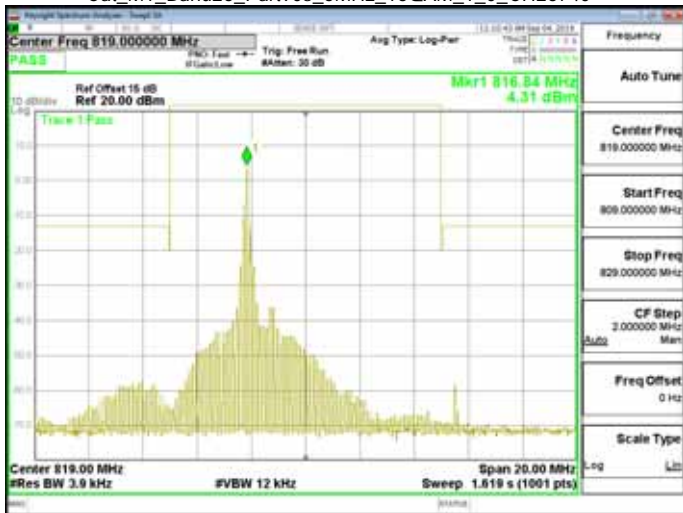
Cat_M1_Band26_Part90s_5MHz_16QAM_1_0_CH26765
