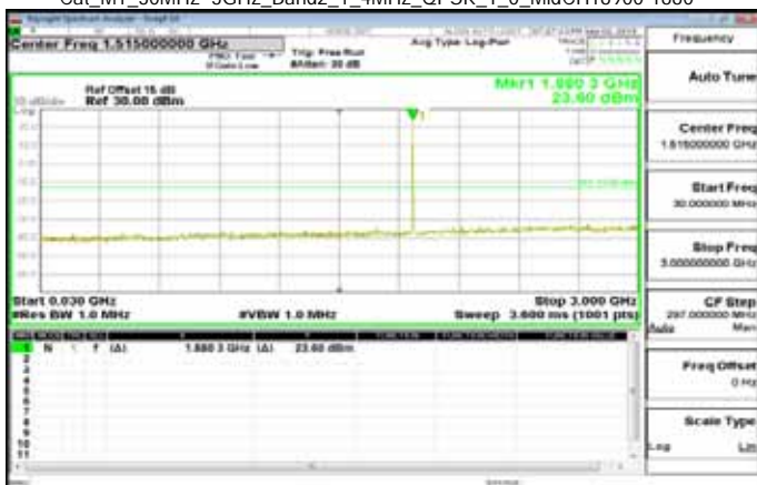
Cat_M1_30MHz-3GHz_Band2_1_4MHz_QPSK_1_0_MidCH18900-1880
