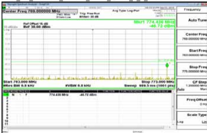
Cat_M1_Inband-1_Band13_5MHz_QPSK_1_0_MidCH23230-782
