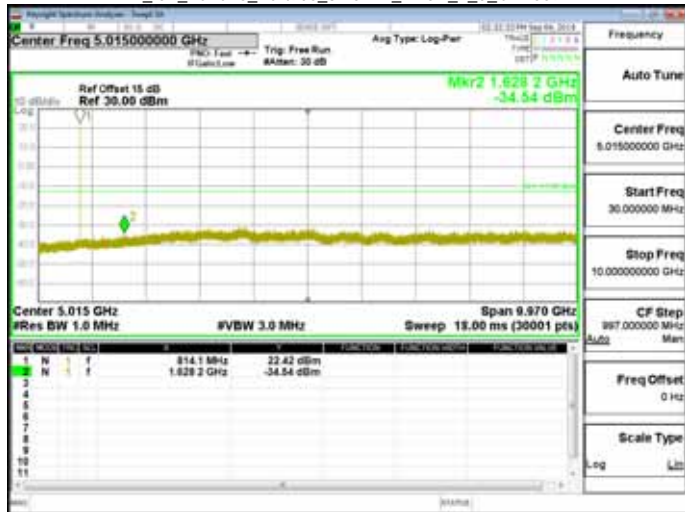
NB_IoT_Band26_Part90s_3.75kHz_BPSK_1_0_CH26740
