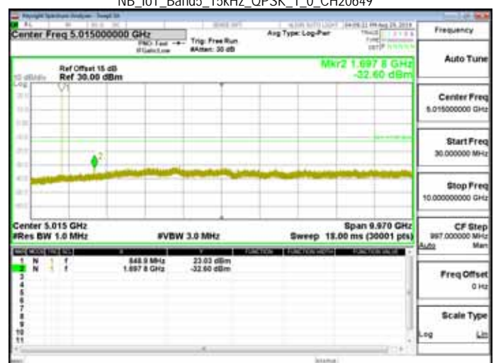
NB_IoT_Band5_15kHz_QPSK_1_0_CH20649
