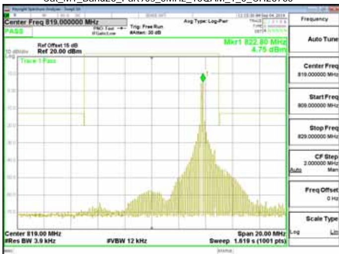
Cat_M1_Band26_Part90s_5MHz_16QAM_1_5_CH26715
