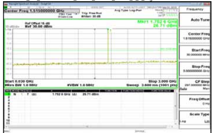
Cat_M1_30MHz-3GHz_Band4_10MHz_QPSK_1_0_HighCH20350-1750
