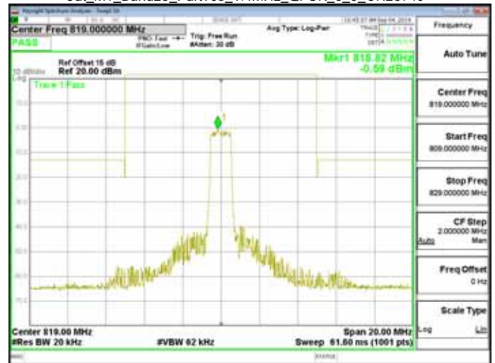
Cat_M1_Band26_Part90s_1.4MHz_QPSK_6_0_CH26783
