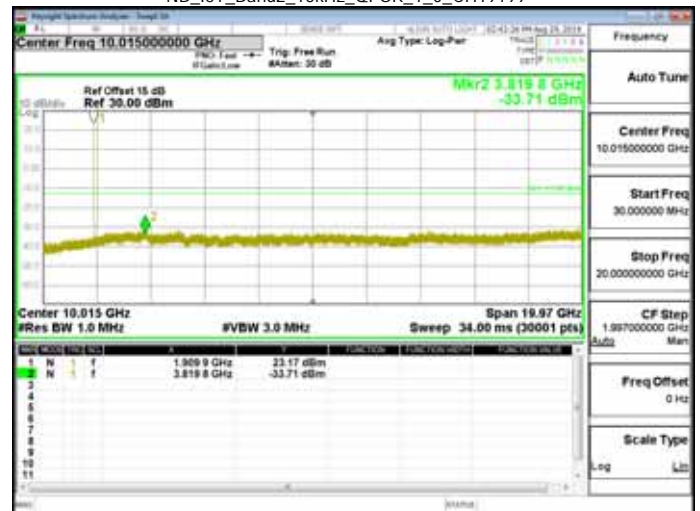
NB_IoT_Band2_15kHz_QPSK_1_0_CH19199
