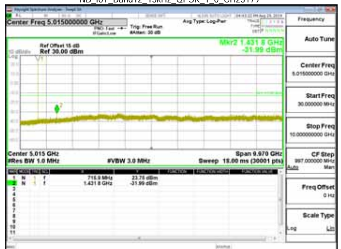
NB_IoT_Band12_15kHz_QPSK_1_0_CH23179
