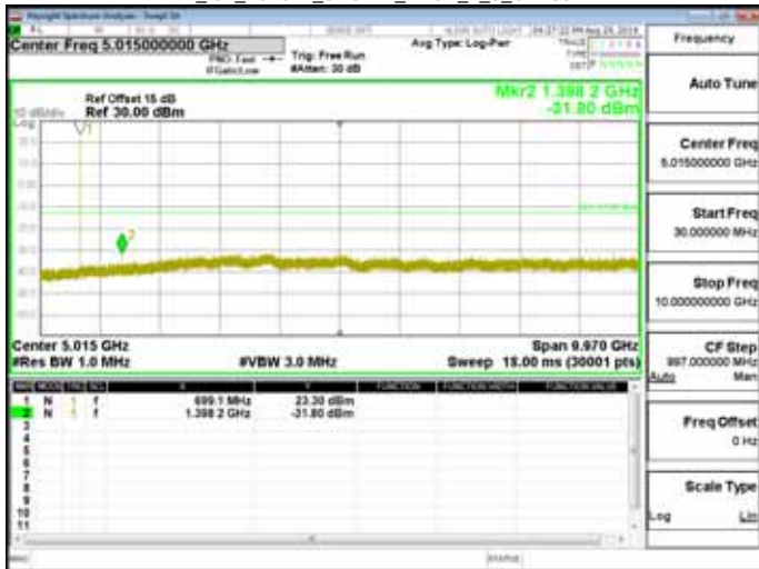
NB_IoT_Band12_3.75kHz_BPSK_1_0_CH23095
