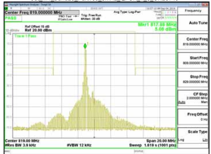
Cat_M1_Band26_Part90s_3MHz_QPSK_1_0_CH26775
