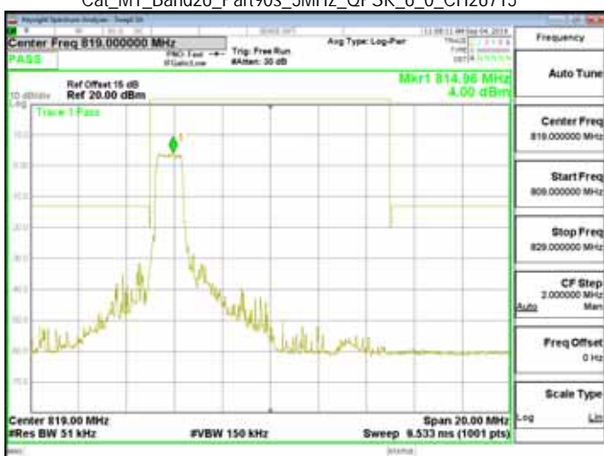
Cat_M1_Band26_Part90s_5MHz_QPSK_6_0_CH26715
