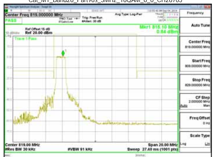
Cat_M1_Band26_Part90s_3MHz_16QAM_6_0_CH26705
