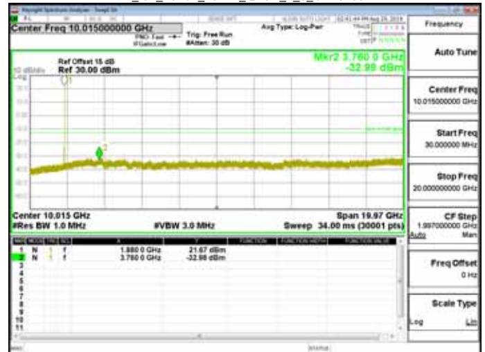
NB_IoT_Band2_15kHz_QPSK_1_0_CH19199
