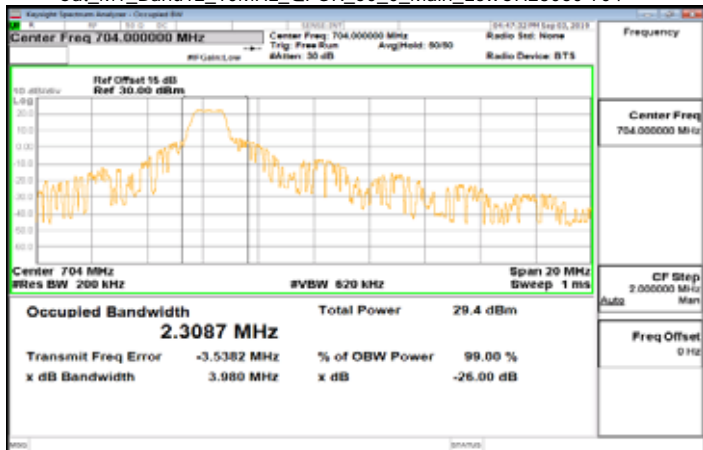
Cat_M1_Band12_10MHz_QPSK_50_0_Main_LowCH23060-704
