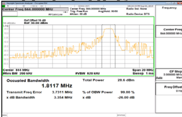
Cat_M1_Band26_10MHz_QPSK_50_0_Main_HighCH26990-844
