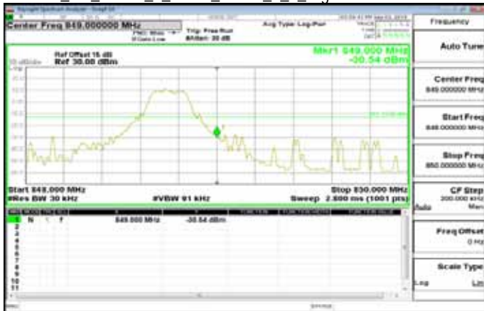
Cat_M1_Band5_1_4MHz_QPSK_1_5_HighCH20643-848.3
