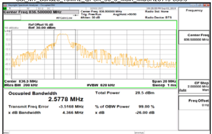
Cat_M1_Band26_10MHz_QPSK_50_0_Main_MidCH26915-836.5
