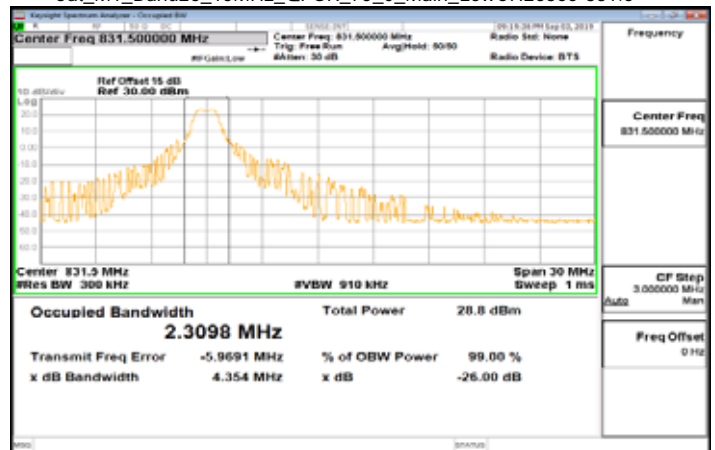
Cat_M1_Band26_15MHz_QPSK_75_0_Main_LowCH26865-831.5
