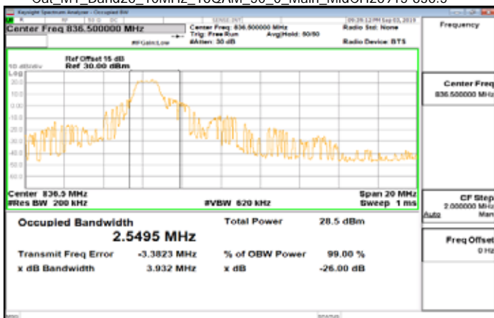
Cat_M1_Band26_10MHz_16QAM_50_0_Main_MidCH26915-836.5
