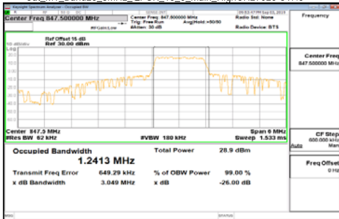
Cat_M1_Band26_3MHz_QPSK_15_0_Main_HighCH27025-847.5
