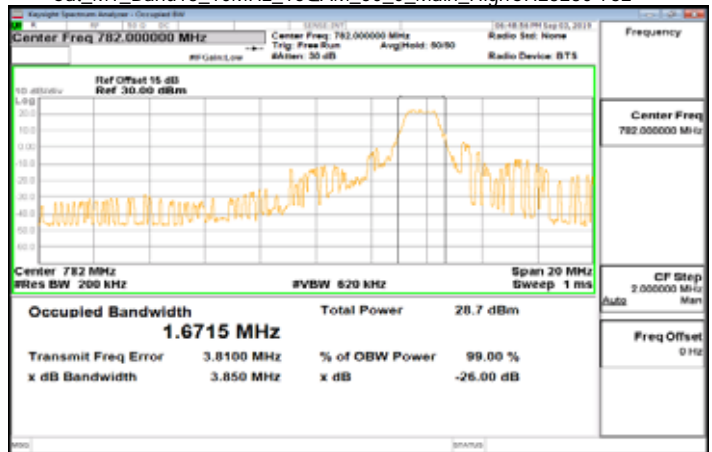
Cat_M1_Band13_10MHz_16QAM_50_0_Main_HighCH23230-782
