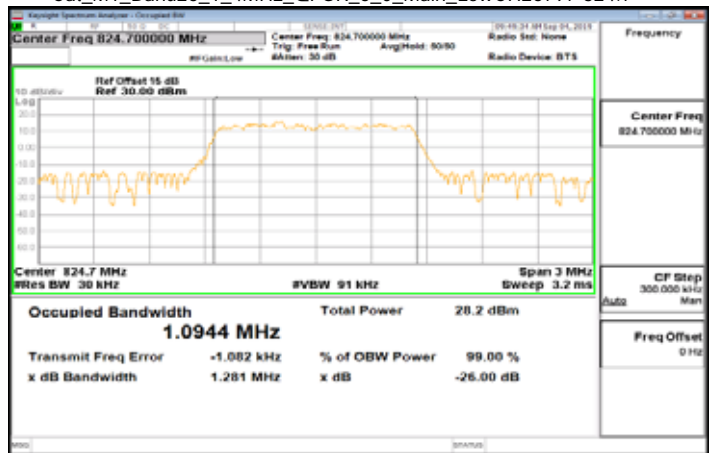
Cat_M1_Band26_1_4MHz_QPSK_6_0_Main_LowCH26797-824.7
