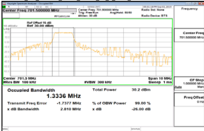
Cat_M1_Band12_5MHz_QPSK_25_0_Main_LowCH23035-701.5
