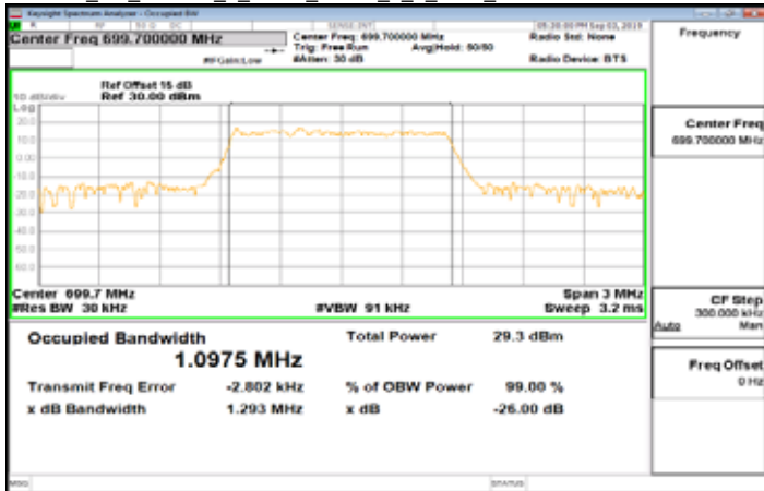
Cat_M1_Band12_1_4MHz_QPSK_6_0_Main_LowCH23017-699.7
