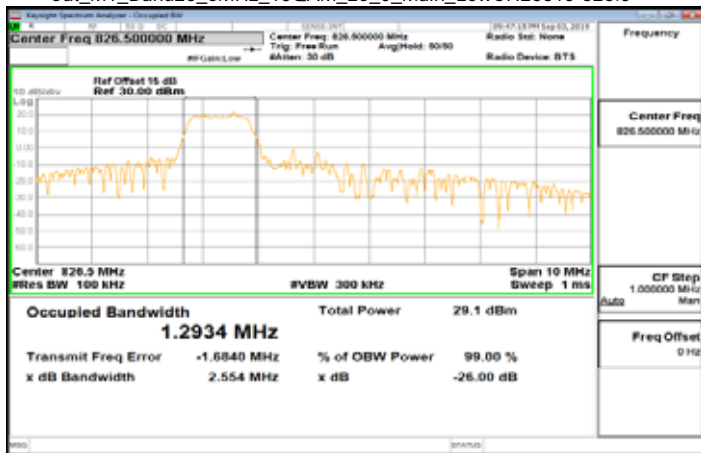
Cat_M1_Band26_5MHz_16QAM_25_0_Main_LowCH26815-826.5
