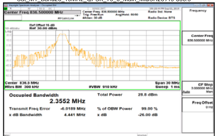
Cat_M1_Band26_15MHz_QPSK_75_0_Main_MidCH26915-836.5
