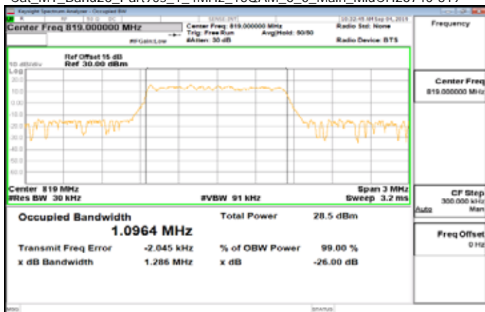
Cat_M1_Band26_Part90s_1_4MHz_16QAM_6_0_Main_MidCH26740-819.0
