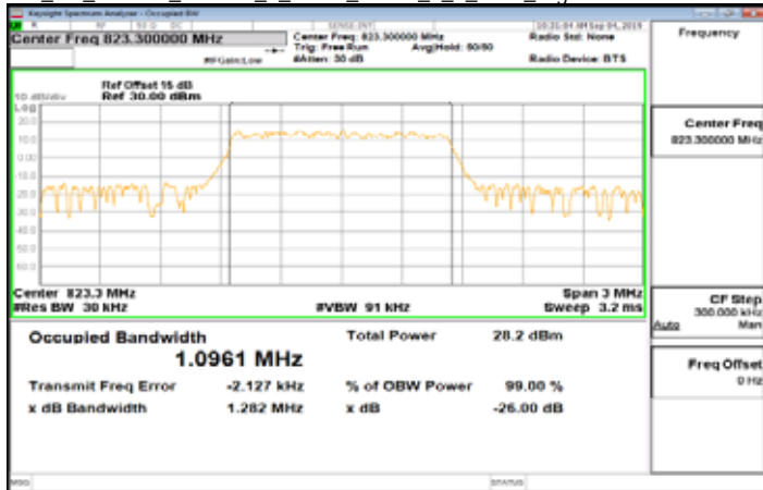
Cat_M1_Band26_Part90s_1_4MHz_QPSK_6_0_Main_HighCH26783-823.3
