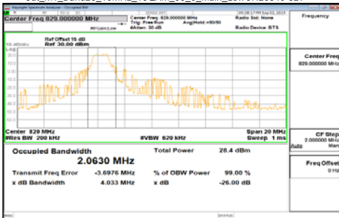
Cat_M1_Band26_10MHz_16QAM_50_0_Main_LowCH26840-829
