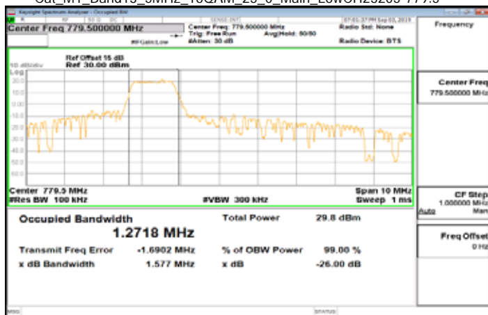
Cat_M1_Band13_5MHz_16QAM_25_0_Main_LowCH23205-779.5
