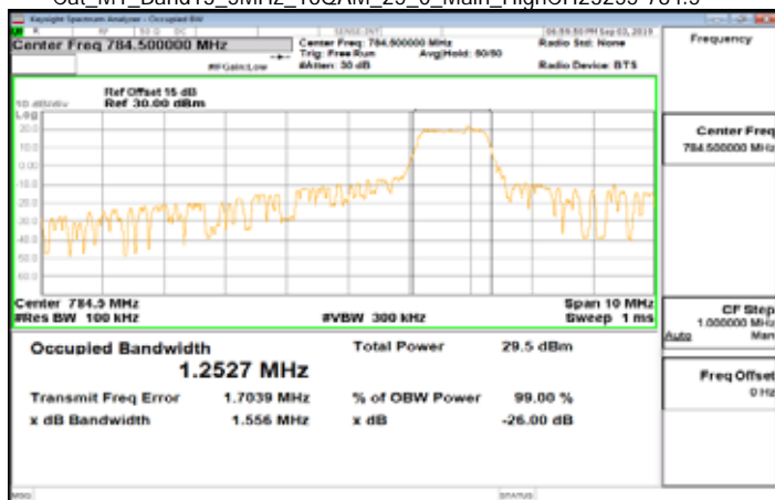
Cat_M1_Band13_5MHz_16QAM_25_0_Main_HighCH23255-784.5
