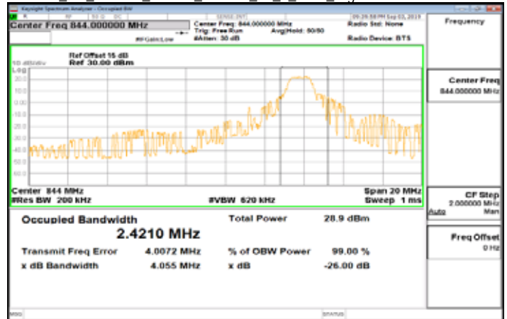
Cat_M1_Band26_10MHz_16QAM_50_0_Main_HighCH26990-844
