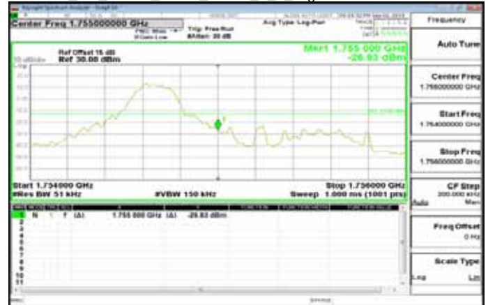
Cat_M1_Band4_5MHz_QPSK_1_5_HighCH20375-1752.5
