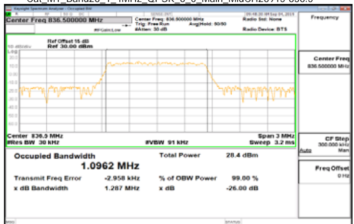
Cat_M1_Band26_1_4MHz_QPSK_6_0_Main_MidCH26915-836.5
