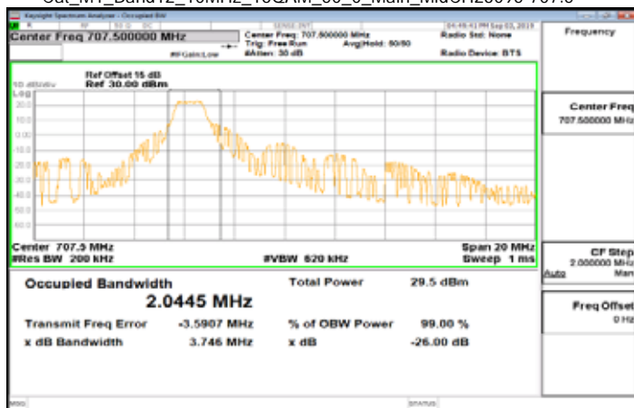
Cat_M1_Band12_10MHz_16QAM_50_0_Main_MidCH23095-707.5
