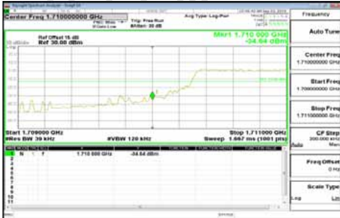
Cat_M1_Band4_3MHz_QPSK_6_0_LowCH19965-1711.5
