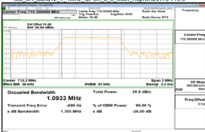
Cat_M1_Band12_1_4MHz_QPSK_6_0_Main_HighCH23173-715.3
