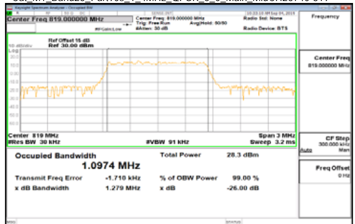
Cat_M1_Band26_Part90s_1_4MHz_QPSK_6_0_Main_MidCH26740-819
