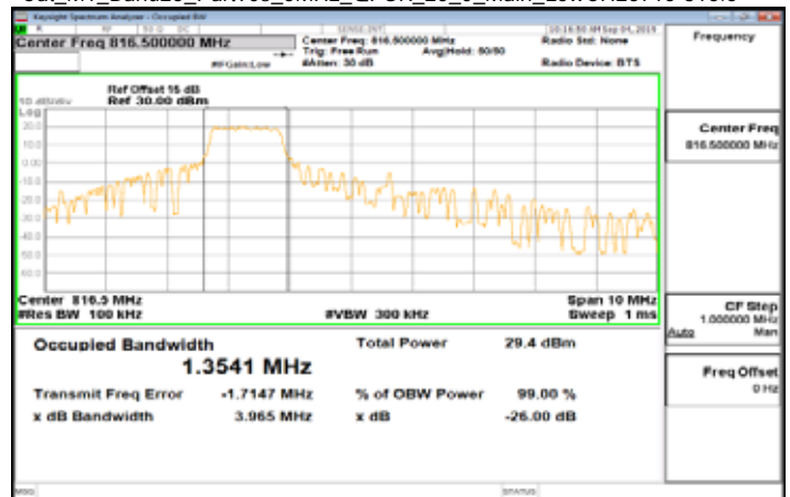
Cat_M1_Band26_Part90s_5MHz_QPSK_25_0_Main_LowCH26715-816.5
