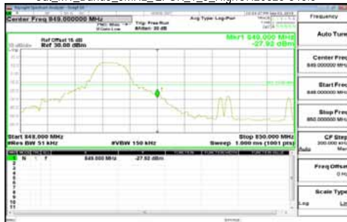
Cat_M1_Band5_5MHz_QPSK_1_5_HighCH20625-846.5
