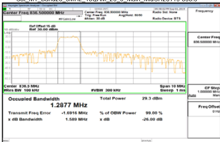
Cat_M1_Band26_5MHz_16QAM_25_0_Main_MidCH26915-836.5
