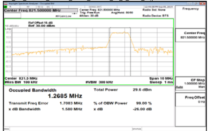
Cat_M1_Band26_Part90s_5MHz_16QAM_25_0_Main_HighCH26765-821.5
