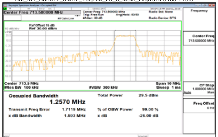
Cat_M1_Band12_5MHz_16QAM_25_0_Main_HighCH23155-713.5
