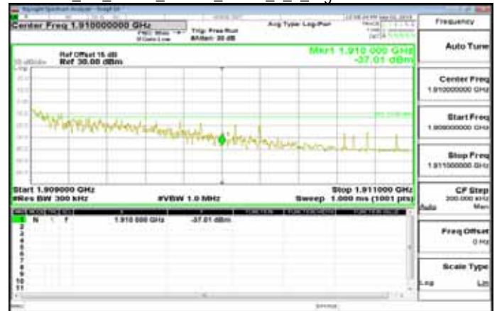
Cat_M1_Band2_20MHz_QPSK_1_5_HighCH19100-1900
