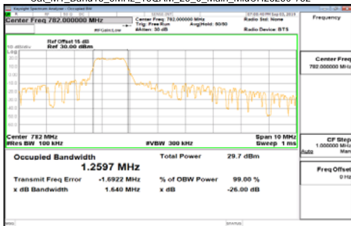
Cat_M1_Band13_5MHz_16QAM_25_0_Main_MidCH23230-782
