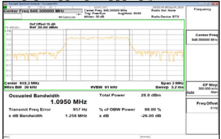
Cat_M1_Band26_1_4MHz_16QAM_6_0_Main_HighCH27033-848.3
