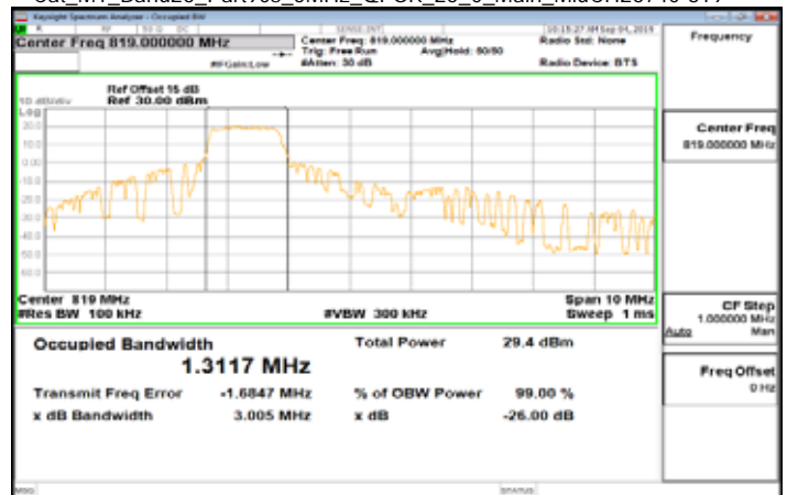
Cat_M1_Band26_Part90s_5MHz_QPSK_25_0_Main_MidCH26740-819
