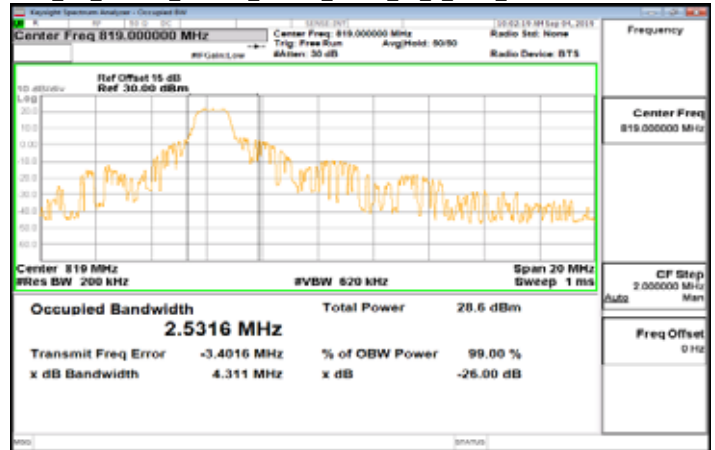
Cat_M1_Band26_Part90s_10MHz_QPSK_50_0_Main_LowCH26740-819
