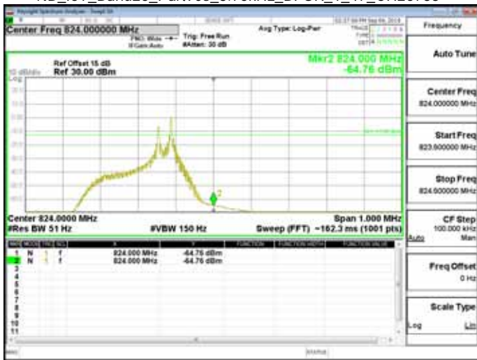
NB_IoT_Band26_Part90s_15kHz_QPSK_1_0_CH26692
