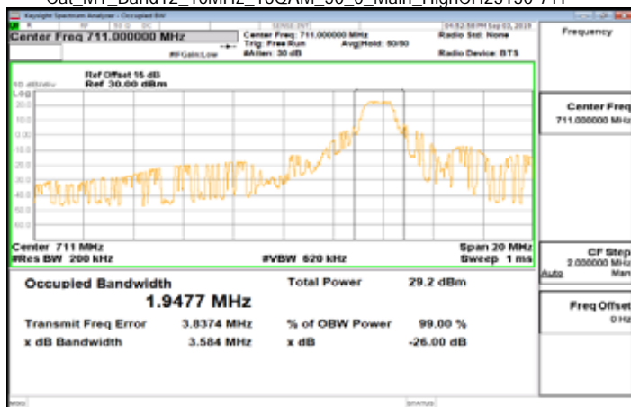
Cat_M1_Band12_10MHz_16QAM_50_0_Main_HighCH23130-711
