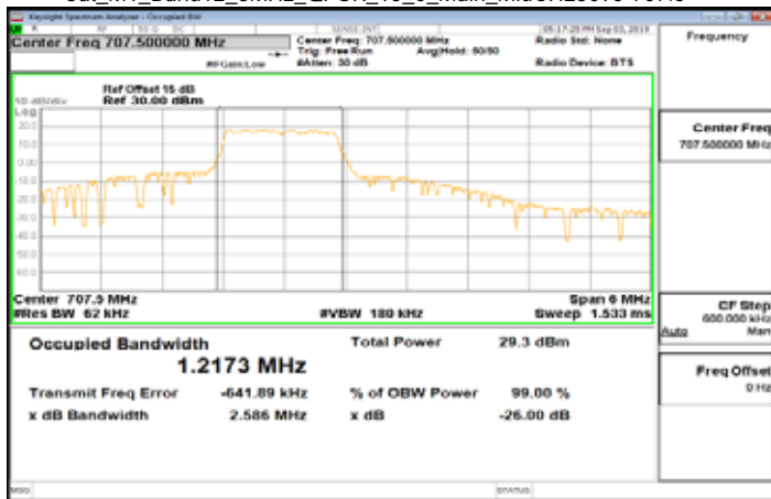
Cat_M1_Band12_3MHz_QPSK_15_0_Main_MidCH23095-707.5
