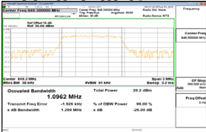
Cat_M1_Band26_1_4MHz_QPSK_6_0_Main_HighCH27033-848.3
