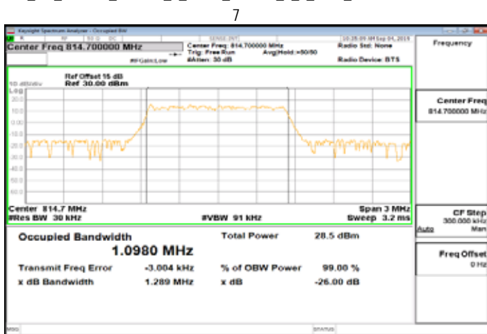
Cat_M1_Band26_Part90s_1_4MHz_16QAM_6_0_Main_LowCH26697-814.7
