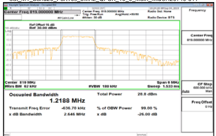
Cat_M1_Band26_Part90s_3MHz_QPSK_15_0_Main_MidCH26740-819.0
