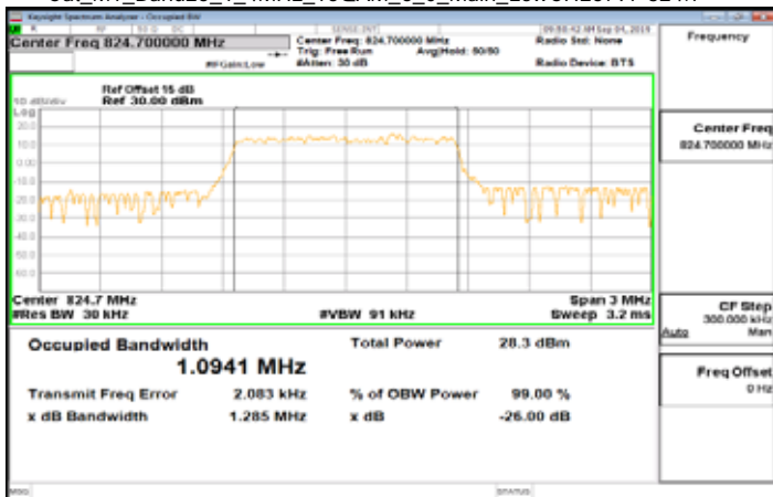
Cat_M1_Band26_1_4MHz_16QAM_6_0_Main_LowCH26797-824.7
