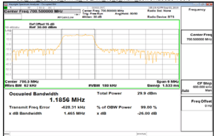
Cat_M1_Band12_3MHz_16QAM_15_0_Main_LowCH23025-700.5
