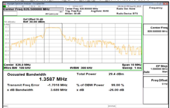
Cat_M1_Band26_5MHz_QPSK_25_0_Main_LowCH26815-826.5
