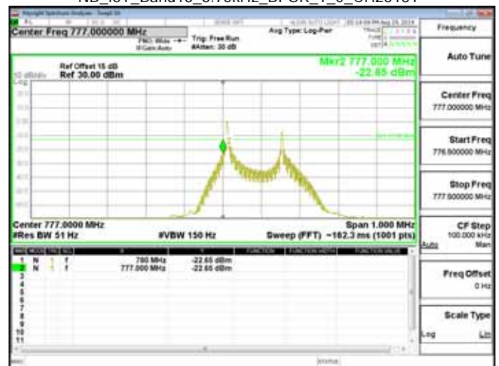
NB_IoT_Band13_3.75kHz_BPSK_1_0_CH23181
