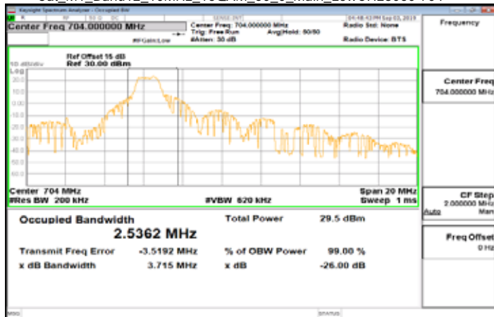
Cat_M1_Band12_10MHz_16QAM_50_0_Main_LowCH23060-704
