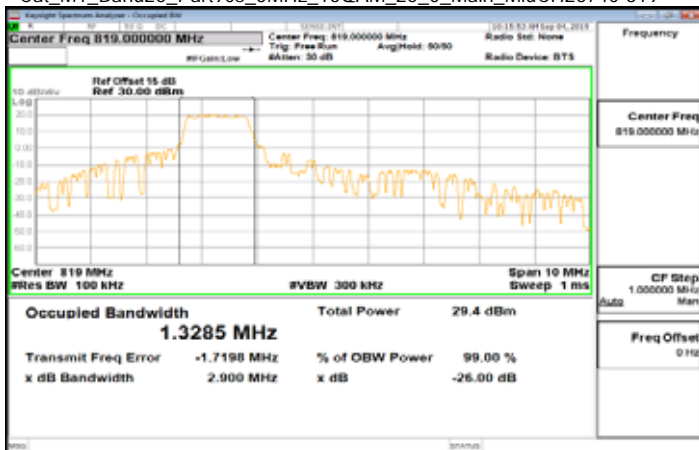
Cat_M1_Band26_Part90s_5MHz_16QAM_25_0_Main_MidCH26740-819
