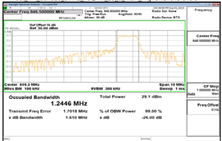
Cat_M1_Band26_5MHz_16QAM_25_0_Main_HighCH27015-846.5
