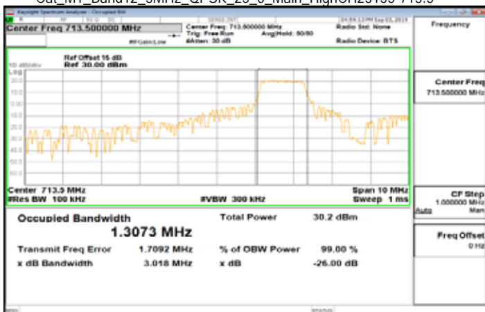
Cat_M1_Band12_5MHz_QPSK_25_0_Main_HighCH23155-713.5
