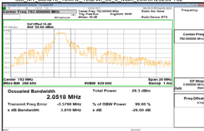
Cat_M1_Band13_10MHz_16QAM_50_0_Main_LowCH23230-782
