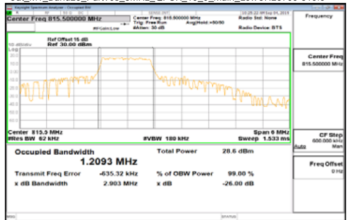
Cat_M1_Band26_Part90s_3MHz_QPSK_15_0_Main_LowCH26705-815.5
