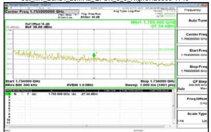
Cat_M1_Band4_20MHz_QPSK_6_0_HighCH20300-1745
