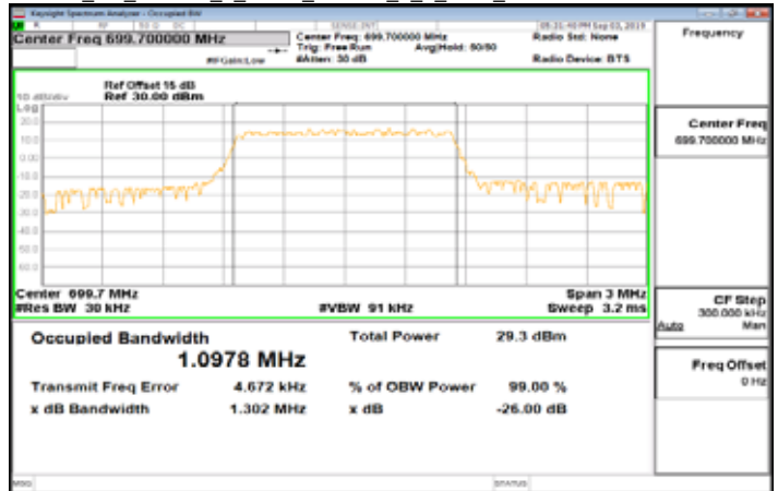
Cat_M1_Band12_1_4MHz_16QAM_6_0_Main_LowCH23017-699.7
