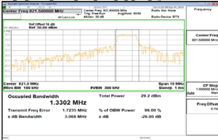
Cat_M1_Band26_Part90s_5MHz_QPSK_25_0_Main_HighCH26765-821.5
