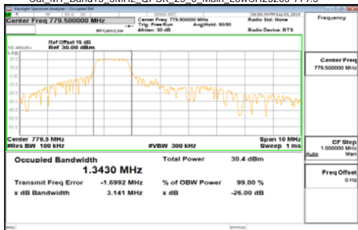
Cat_M1_Band13_5MHz_QPSK_25_0_Main_LowCH23205-779.5
