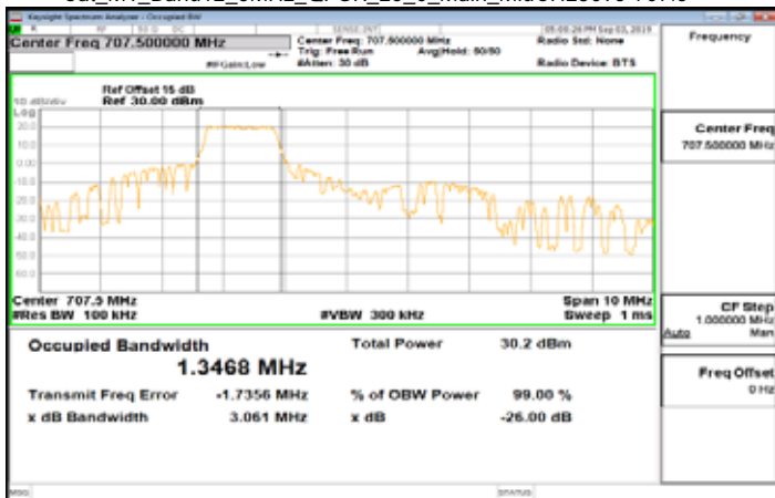
Cat_M1_Band12_5MHz_QPSK_25_0_Main_MidCH23095-707.5
