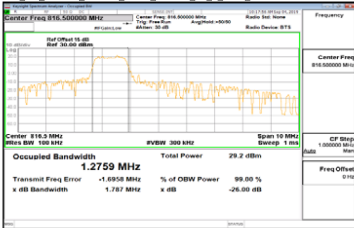
Cat_M1_Band26_Part90s_5MHz_16QAM_25_0_Main_LowCH26715-816.5
