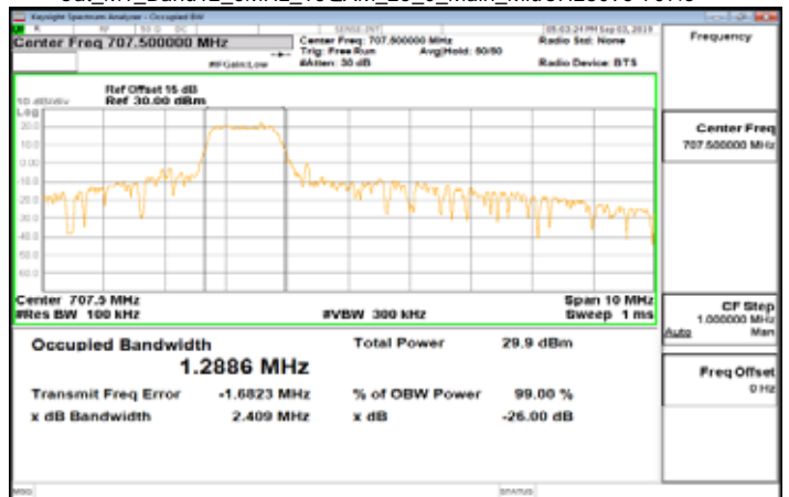
Cat_M1_Band12_5MHz_16QAM_25_0_Main_MidCH23095-707.5
