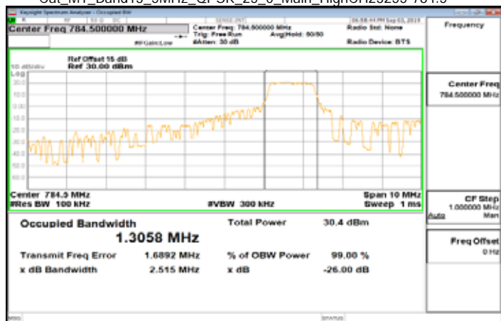
Cat_M1_Band13_5MHz_QPSK_25_0_Main_HighCH23255-784.5
