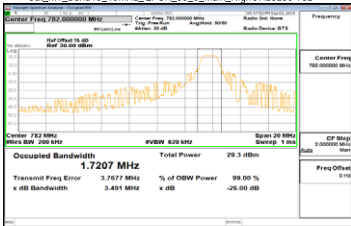
Cat_M1_Band13_10MHz_QPSK_50_0_Main_HighCH23230-782
