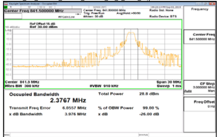
Cat_M1_Band26_15MHz_16QAM_75_0_Main_HighCH26965-841.5
