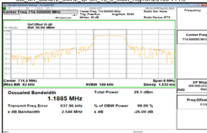
Cat_M1_Band12_3MHz_QPSK_15_0_Main_HighCH23165-714.5
