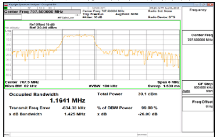
Cat_M1_Band12_3MHz_16QAM_15_0_Main_MidCH23095-707.5
