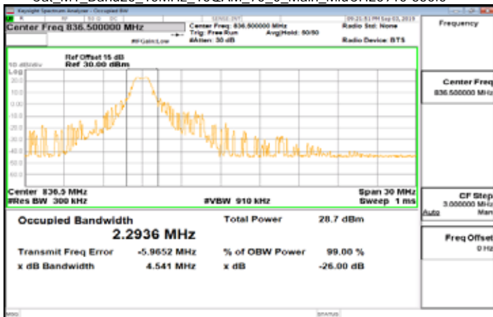
Cat_M1_Band26_15MHz_16QAM_75_0_Main_MidCH26915-836.5
