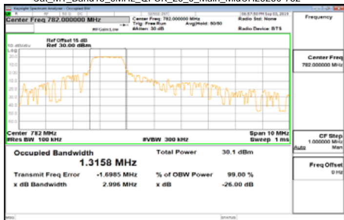
Cat_M1_Band13_5MHz_QPSK_25_0_Main_MidCH23230-782
