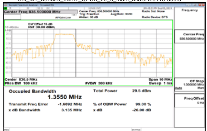
Cat_M1_Band26_5MHz_QPSK_25_0_Main_MidCH26915-836.5
