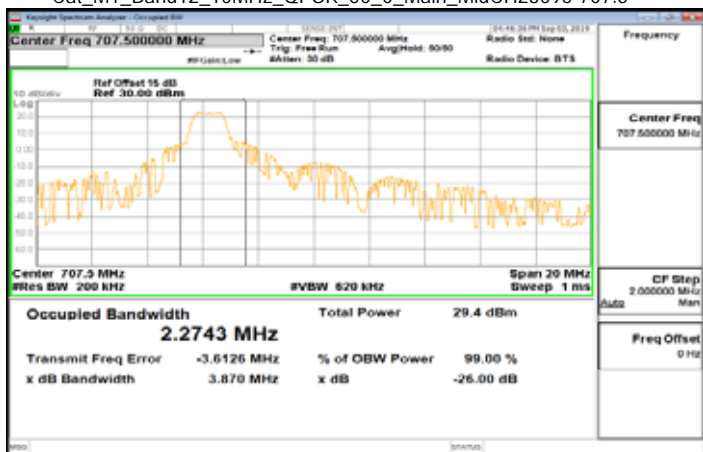
Cat_M1_Band12_10MHz_QPSK_50_0_Main_MidCH23095-707.5
