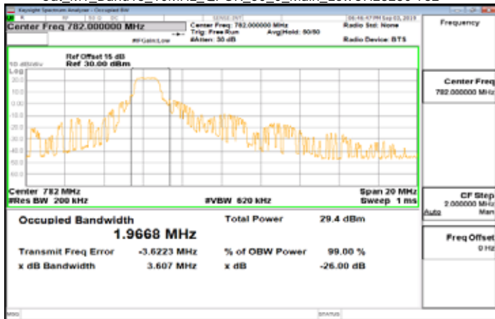
Cat_M1_Band13_10MHz_QPSK_50_0_Main_LowCH23230-782
