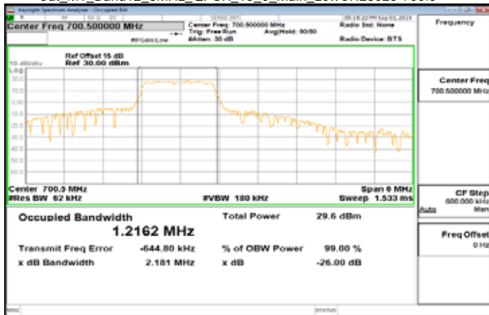
Cat_M1_Band12_3MHz_QPSK_15_0_Main_LowCH23025-700.5
