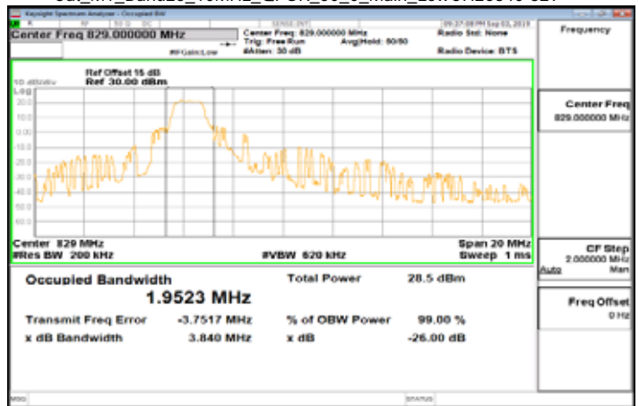
Cat_M1_Band26_10MHz_QPSK_50_0_Main_LowCH26840-829
