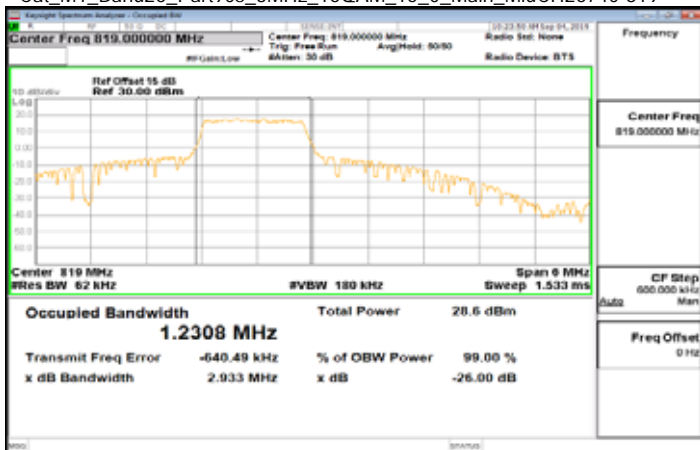
Cat_M1_Band26_Part90s_3MHz_16QAM_15_0_Main_MidCH26740-819
