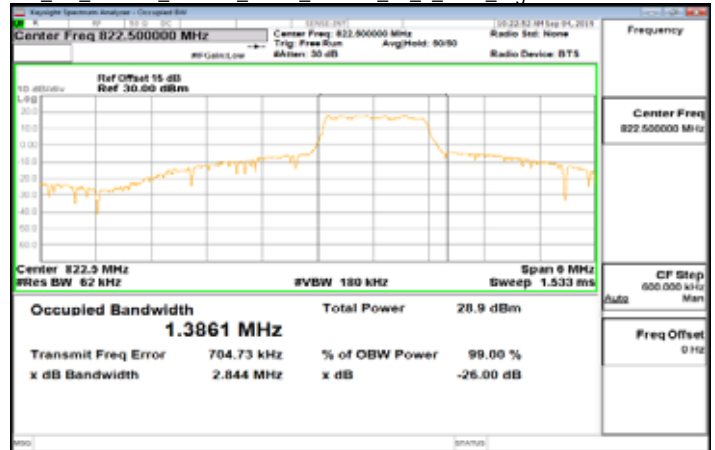
Cat_M1_Band26_Part90s_3MHz_16QAM_15_0_Main_HighCH26775-822.5
