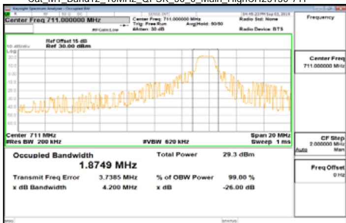
Cat_M1_Band12_10MHz_QPSK_50_0_Main_HighCH23130-711
