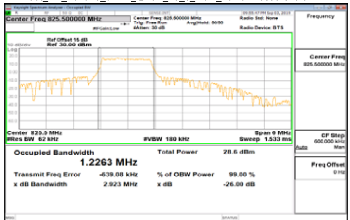
Cat_M1_Band26_3MHz_QPSK_15_0_Main_LowCH26805-825.5
