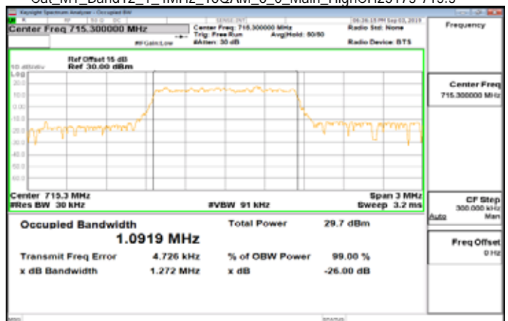
Cat_M1_Band12_1_4MHz_16QAM_6_0_Main_HighCH23173-715.3
