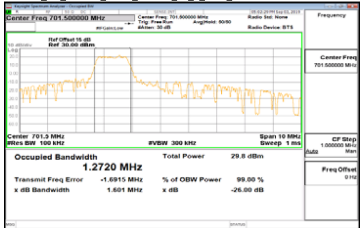
Cat_M1_Band12_5MHz_16QAM_25_0_Main_LowCH23035-701.5
