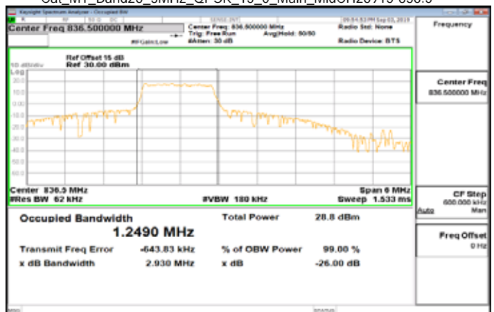
Cat_M1_Band26_3MHz_QPSK_15_0_Main_MidCH26915-836.5
