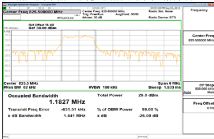
Cat_M1_Band26_3MHz_16QAM_15_0_Main_LowCH26805-825.5
