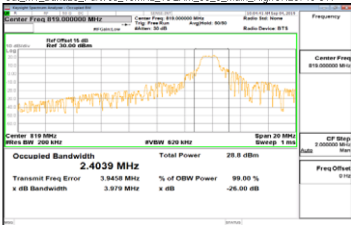
Cat_M1_Band26_Part90s_10MHz_16QAM_50_0_Main_HighCH26740-819
