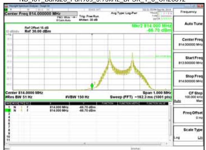
NB_IoT_Band26_Part90s_3.75kHz_BPSK_1_0_CH26692
