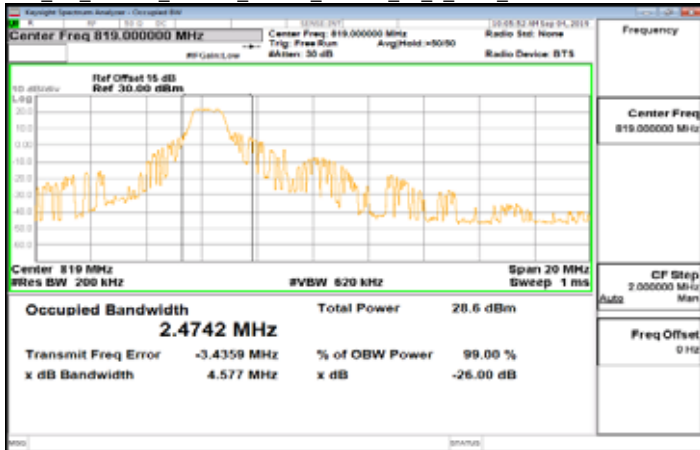
Cat_M1_Band26_Part90s_10MHz_16QAM_50_0_Main_LowCH26740-819
