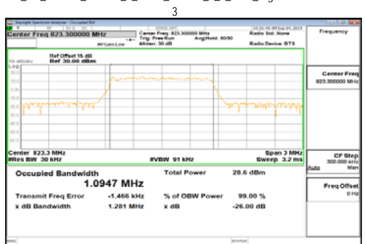
Cat_M1_Band26_Part90s_1_4MHz_16QAM_6_0_Main_HighCH26783-823.3
