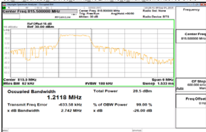
Cat_M1_Band26_Part90s_3MHz_16QAM_15_0_Main_LowCH26705-815.5
