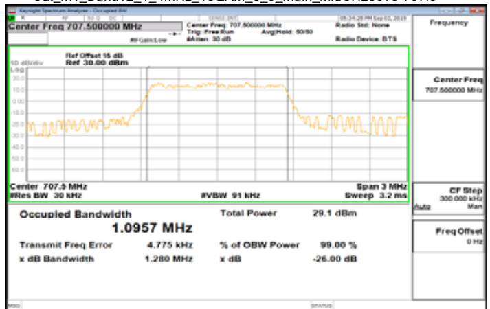
Cat_M1_Band12_1_4MHz_16QAM_6_0_Main_MidCH23095-707.5
