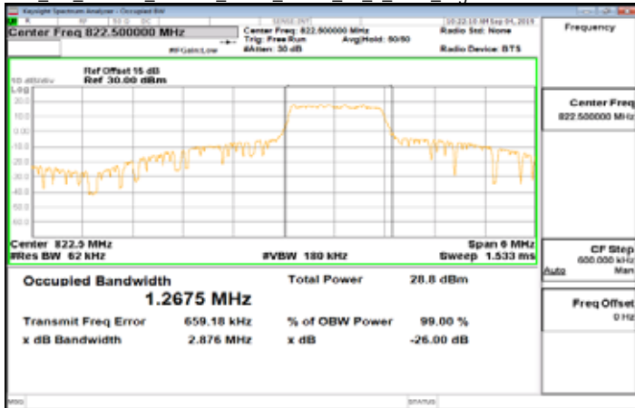
Cat_M1_Band26_Part90s_3MHz_QPSK_15_0_Main_HighCH26775-822.5
