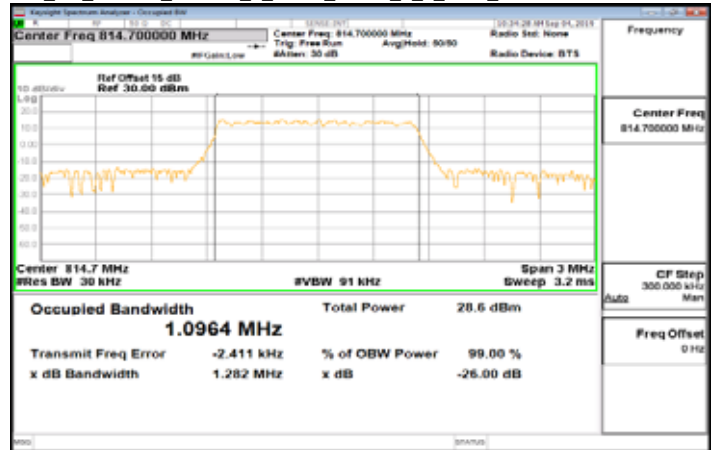
Cat_M1_Band26_Part90s_1_4MHz_QPSK_6_0_Main_LowCH26697-814.7
