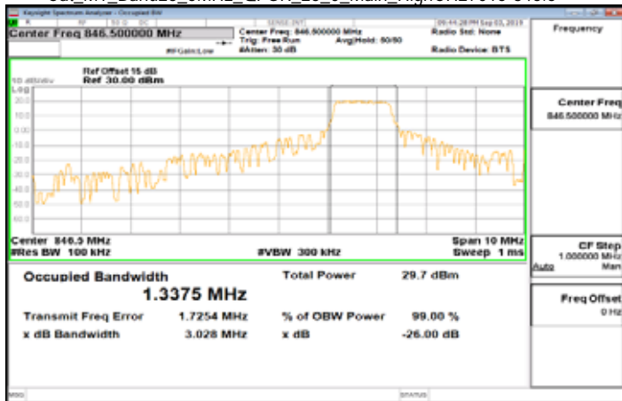
Cat_M1_Band26_5MHz_QPSK_25_0_Main_HighCH27015-846.5
