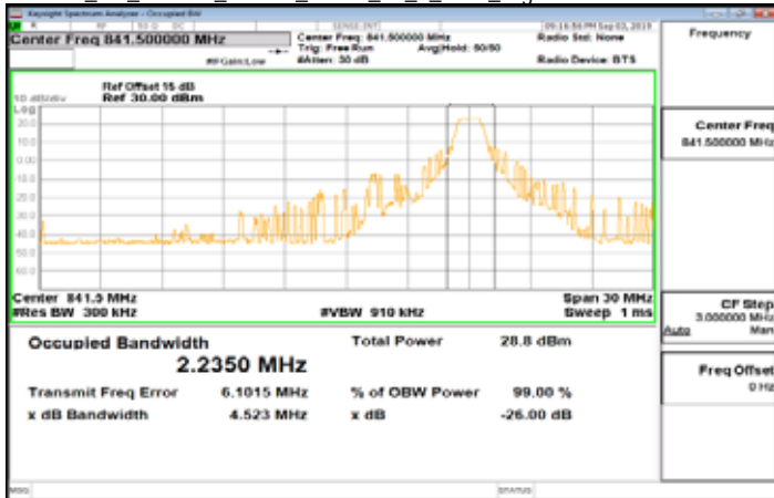
Cat_M1_Band26_15MHz_QPSK_75_0_Main_HighCH26965-841.5
