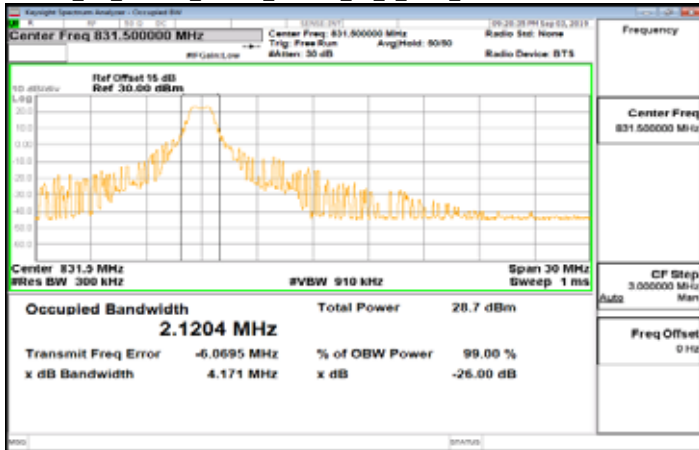
Cat_M1_Band26_15MHz_16QAM_75_0_Main_LowCH26865-831.5
