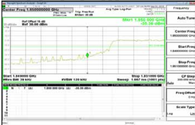
Cat_M1_Band2_3MHz_QPSK_6_0_LowCH18615-1851.5
