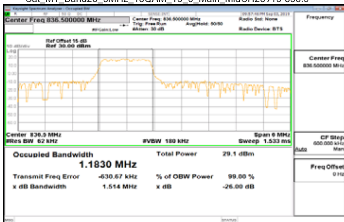
Cat_M1_Band26_3MHz_16QAM_15_0_Main_MidCH26915-836.5
