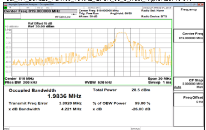
Cat_M1_Band26_Part90s_10MHz_QPSK_50_0_Main_HighCH26740-819
