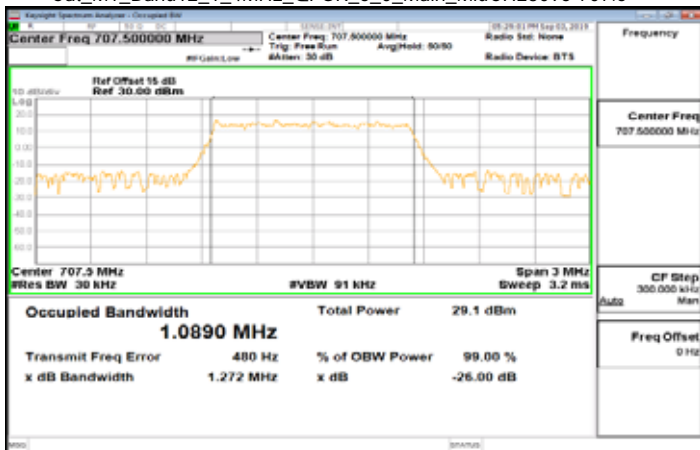
Cat_M1_Band12_1_4MHz_QPSK_6_0_Main_MidCH23095-707.5
