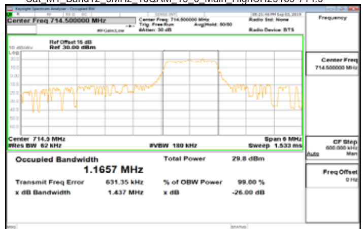
Cat_M1_Band12_3MHz_16QAM_15_0_Main_HighCH23165-714.5
