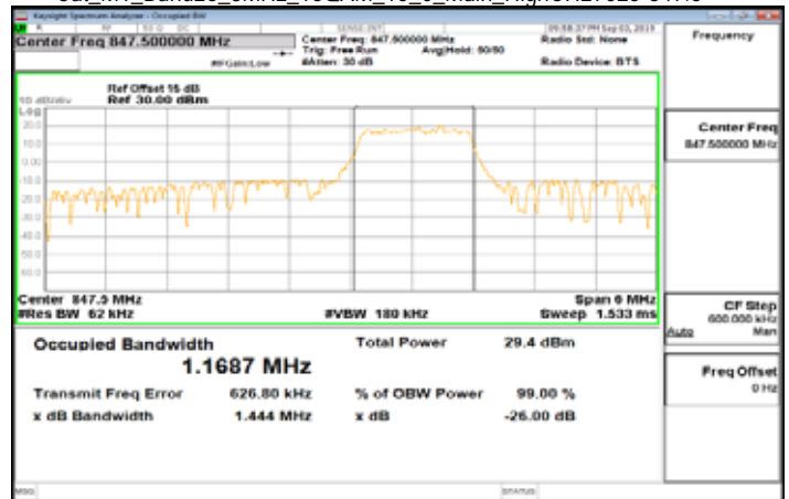
Cat_M1_Band26_3MHz_16QAM_15_0_Main_HighCH27025-847.5
