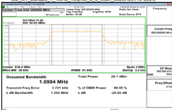
Cat_M1_Band26_1_4MHz_16QAM_6_0_Main_MidCH26915-836.5
