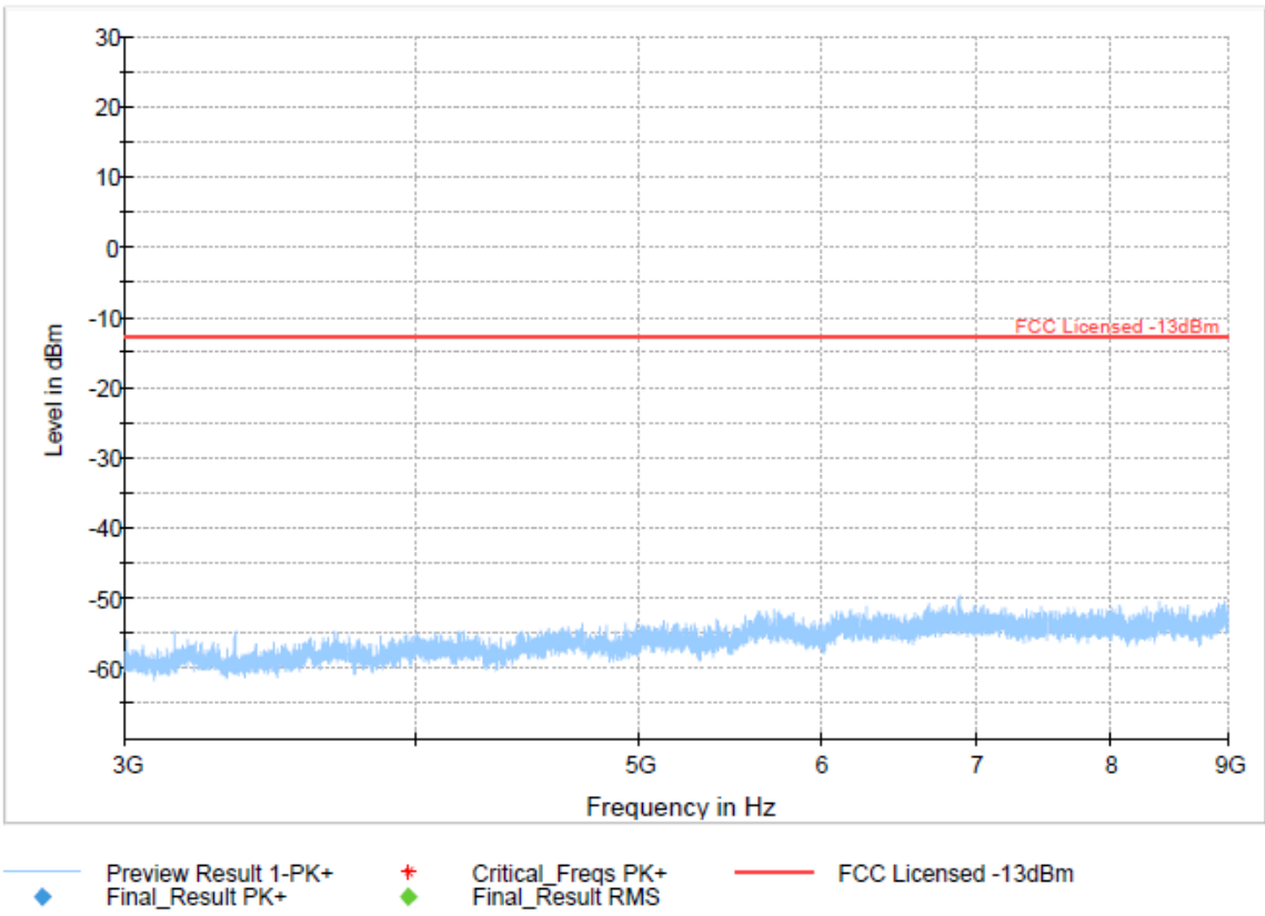
Plot # 6 Radiated Emissions: 3 GHz – 9 GHz
