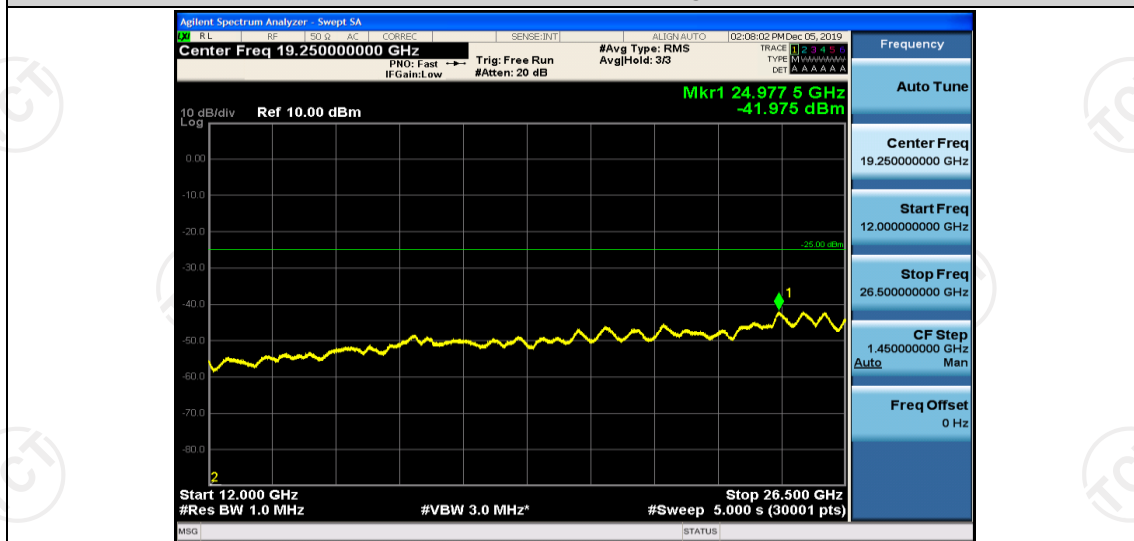
Band41-20MHz-16QAM-41065-1RB#0-Range6:12000~26500MHz
