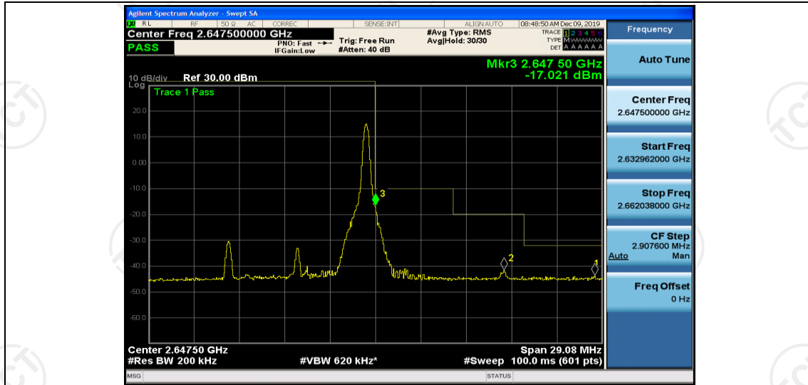
Band41-10MHz-16QAM-41115-50RB#0
