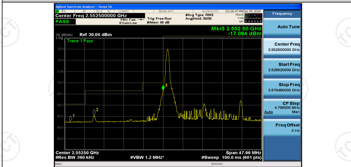
Band41-20MHz-16QAM-40315-1RB#99
