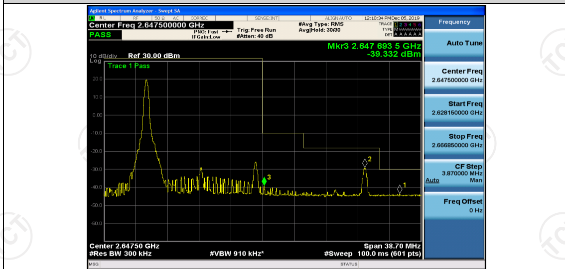
Band41-15MHz-16QAM-41090-1RB#74
