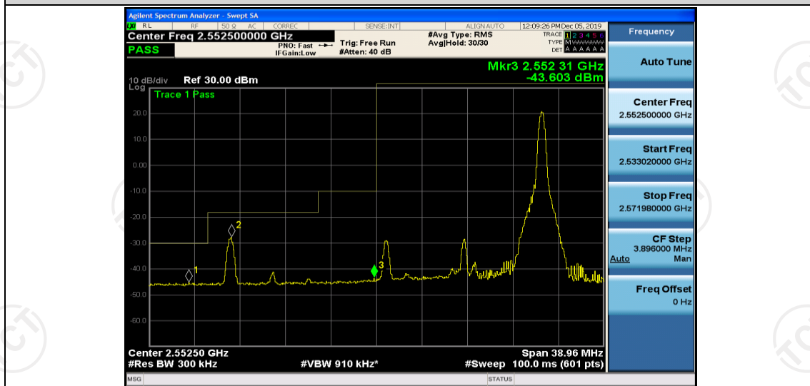
Band41-15MHz-QPSK-40290-1RB#0
