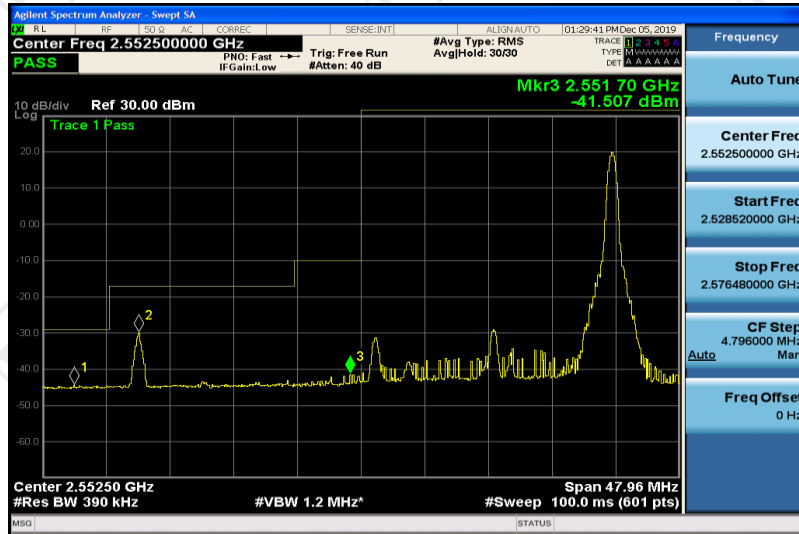
Band41-20MHz-16QAM-40315-100RB#0
