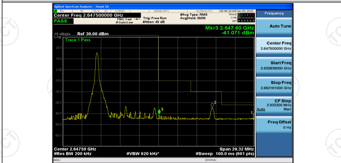
Band41-10MHz-QPSK-41115-1RB#49
