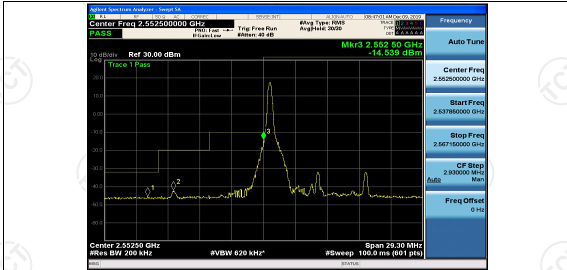
Band41-10MHz-QPSK-40265-50RB#0
