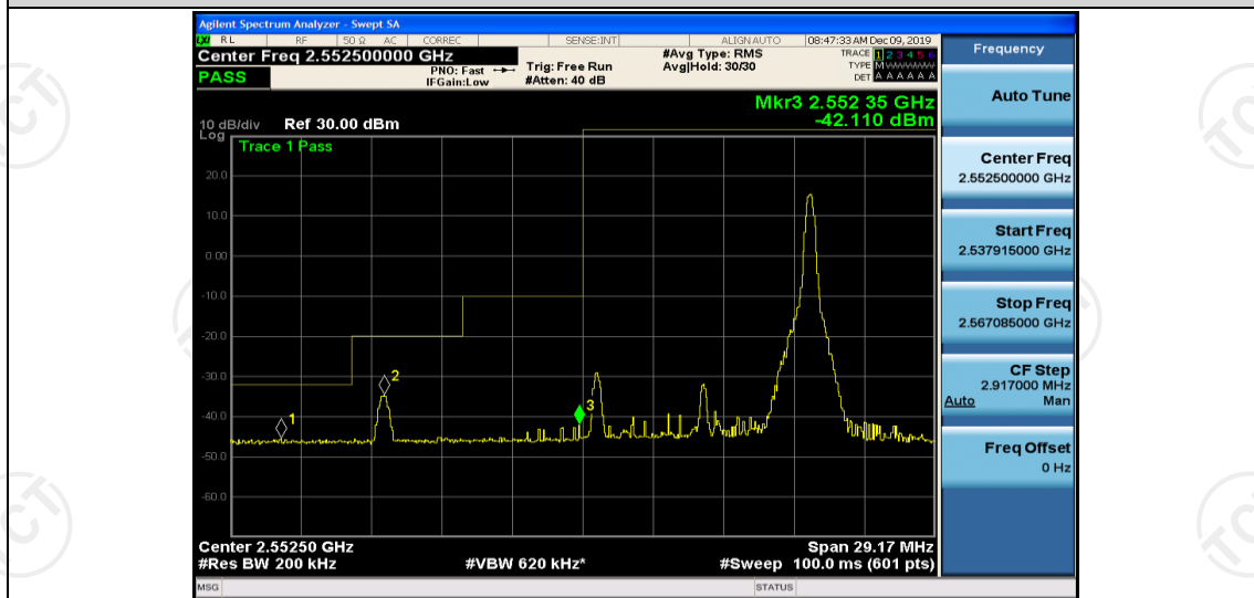
Band41-10MHz-16QAM-40265-1RB#0
