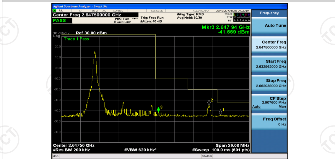
Band41-10MHz-16QAM-41115-1RB#49
