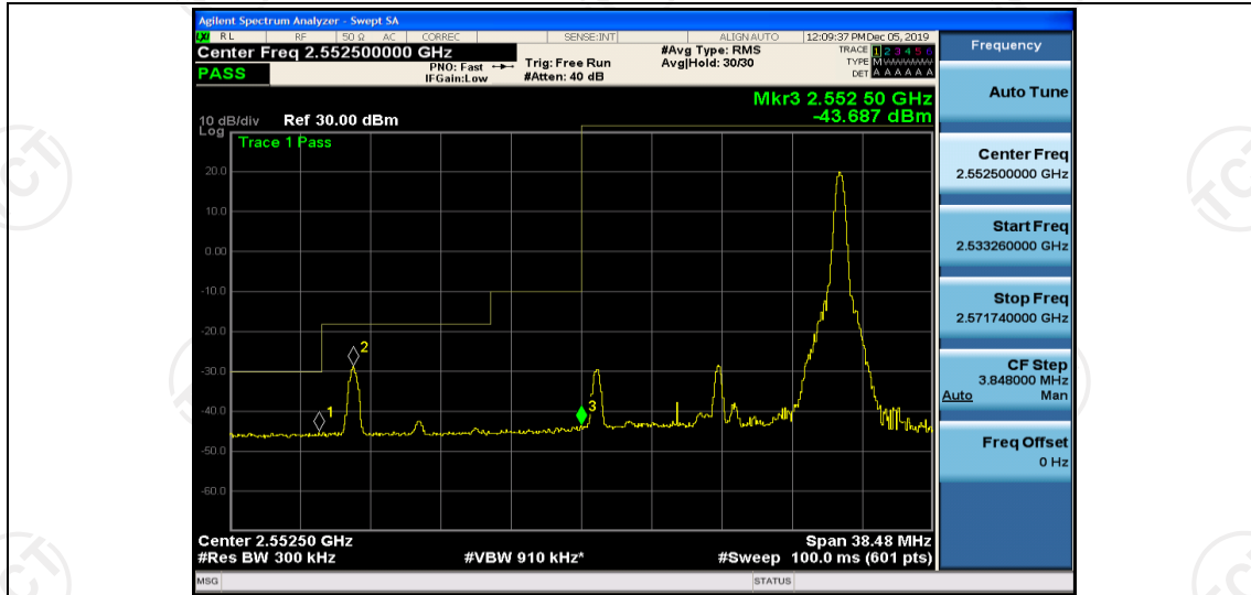
Band41-15MHz-16QAM-40290-75RB#0
