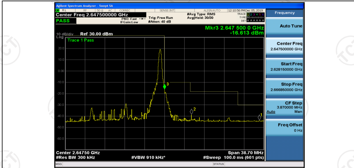
Band41-15MHz-16QAM-41090-75RB#0
