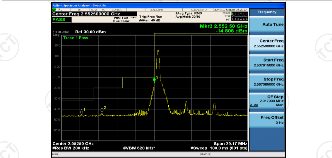
Band41-10MHz-16QAM-40265-50RB#0
