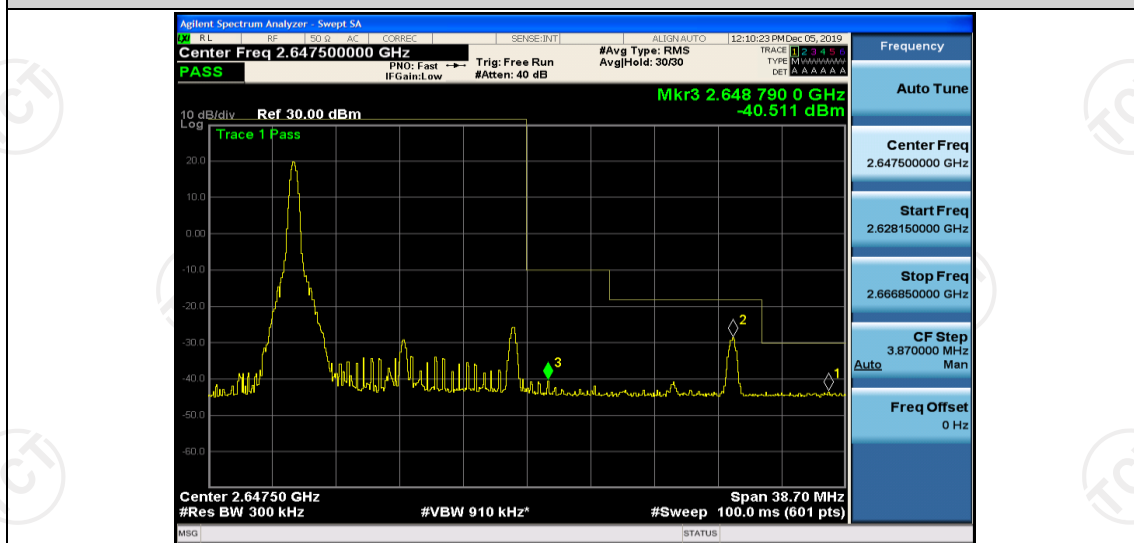
Band41-15MHz-QPSK-41090-1RB#74
