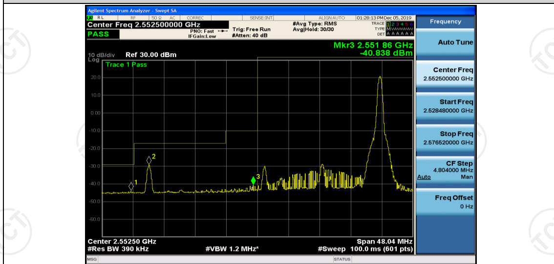
Band41-20MHz-QPSK-40315-1RB#0
