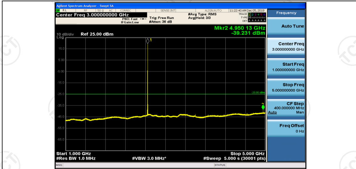
Band41-5MHz-16QAM-41140-1RB#0-Range5:5000~12000MHz
