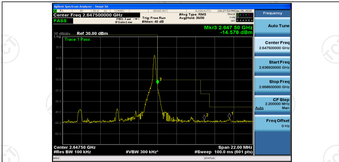
Band41-5MHz-QPSK-41140-25RB#0
