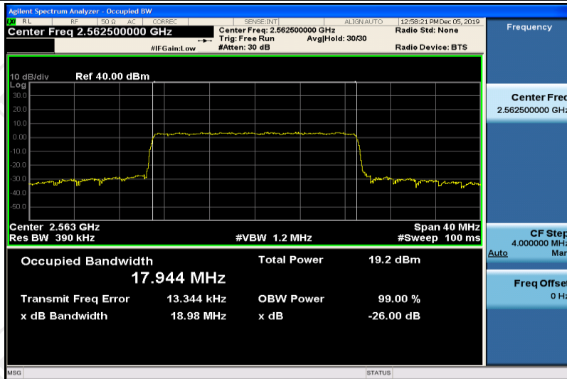
Band41-20MHz-16QAM-40620-100RB#0-17.942
