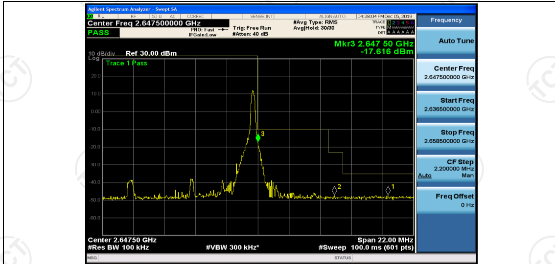
Band41-5MHz-16QAM-41140-25RB#0
