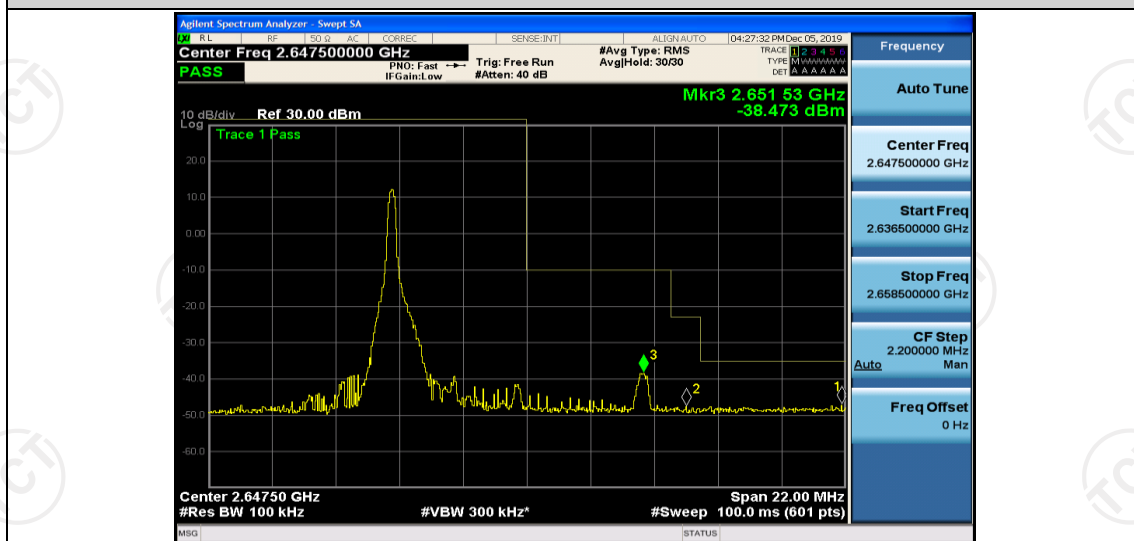
Band41-5MHz-QPSK-41140-1RB#24
