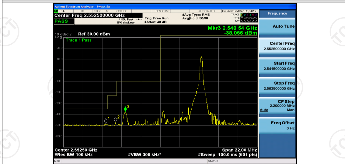
Band41-5MHz-16QAM-40240-1RB#0
