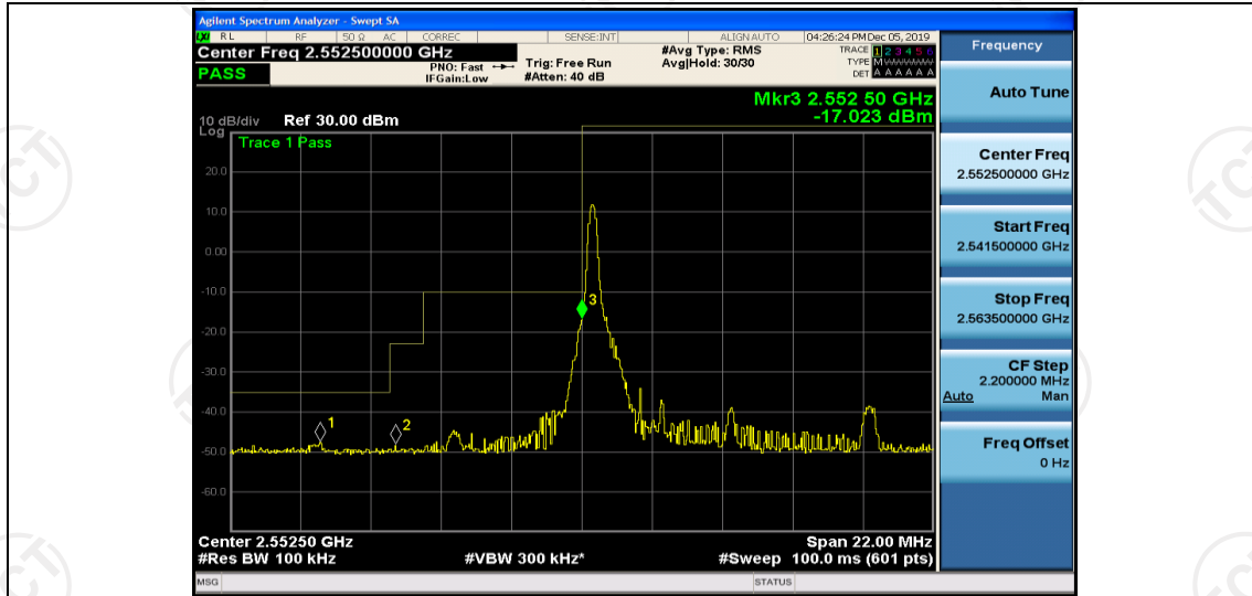
Band41-5MHz-16QAM-40240-25RB#0
