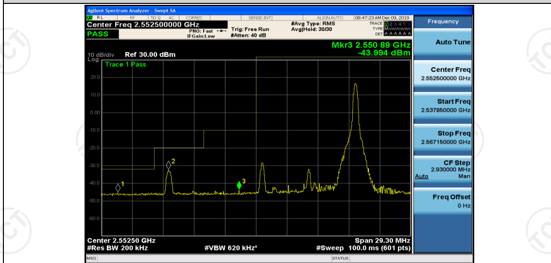
Band41-10MHz-QPSK-40265-1RB#0
