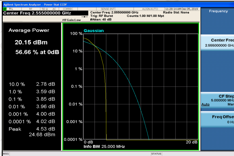
Band41-5MHz-QPSK-40240-25RB#0
