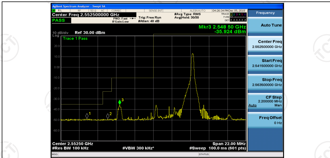
Band41-5MHz-QPSK-40240-25RB#0
