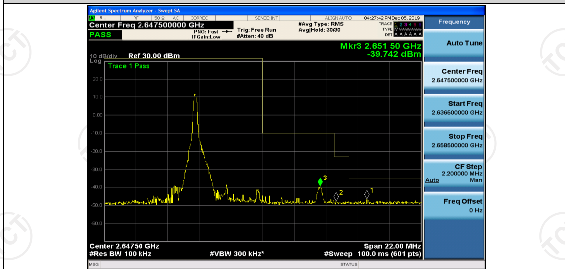
Band41-5MHz-16QAM-41140-1RB#24
