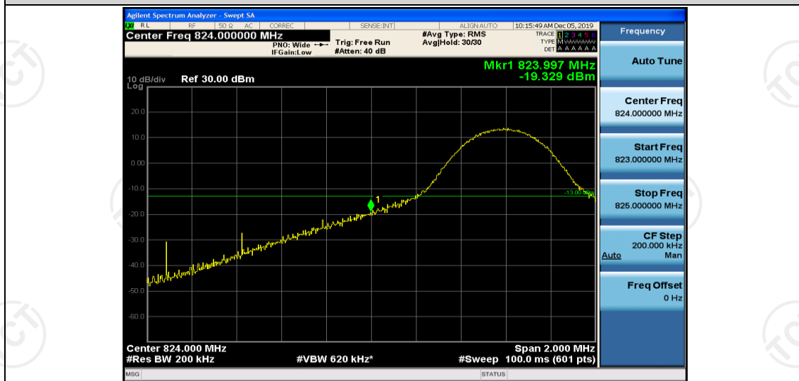
Band26-10MHz-16QAM-26840-1RB#49
