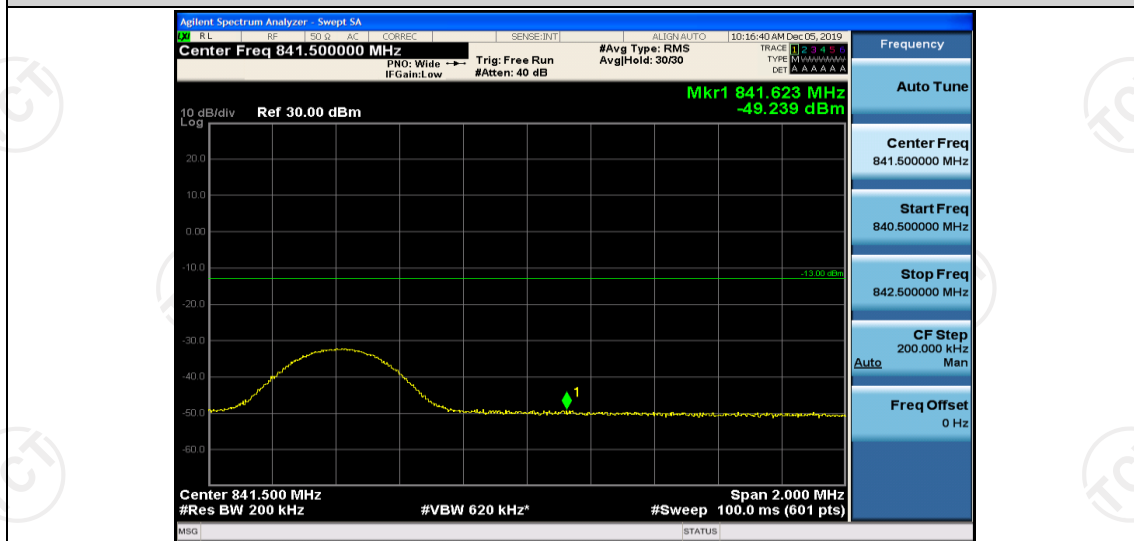
Band26-10MHz-QPSK-26915-1RB#49
