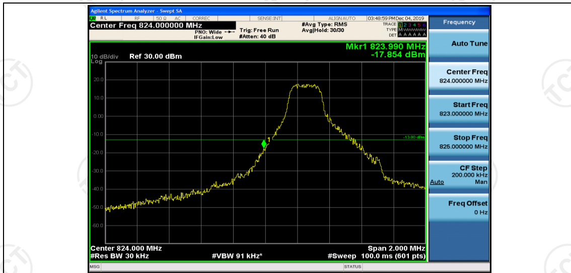
Band26-1.4MHz-QPSK-26797-6RB#0
