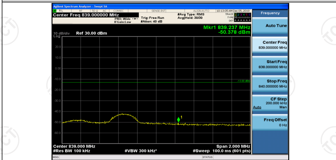
Band26-5MHz-QPSK-26915-1RB#24
