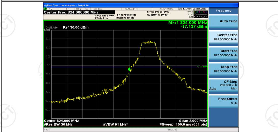
Band26-1.4MHz-16QAM-26797-1RB#5
