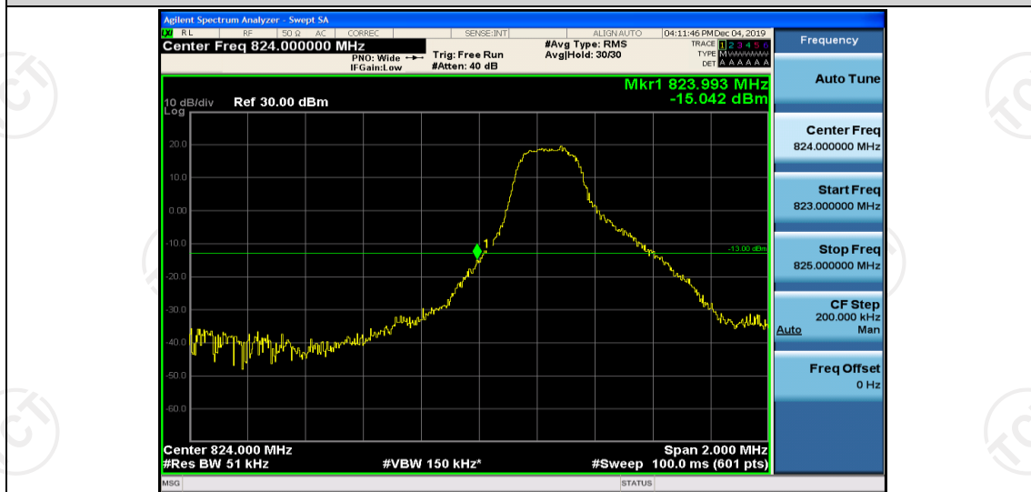
Band26-3MHz-QPSK-26805-1RB#14
