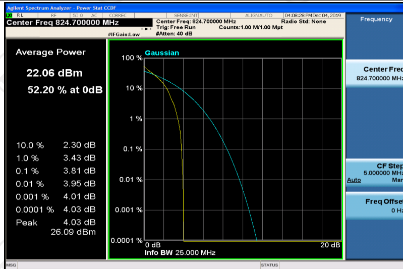
Band26-1.4MHz-QPSK-26797-6RB#0
