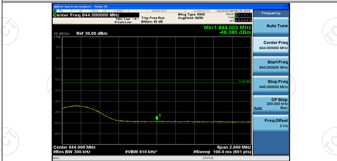
Band26-15MHz-16QAM-26915-1RB#74
