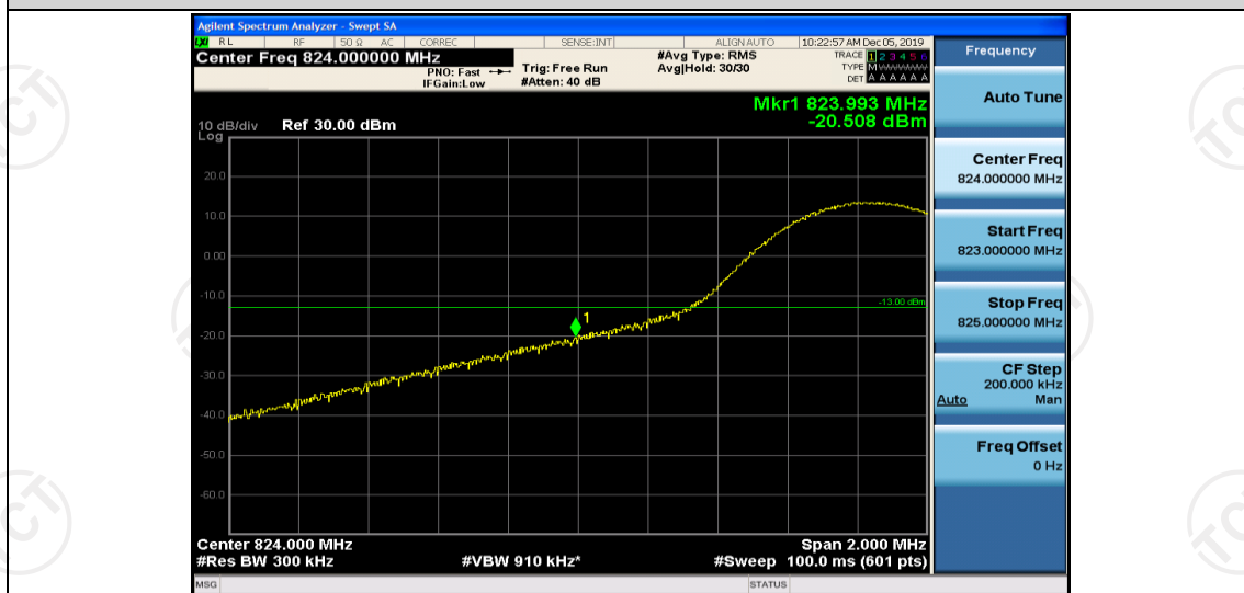
Band26-15MHz-16QAM-26865-1RB#74
