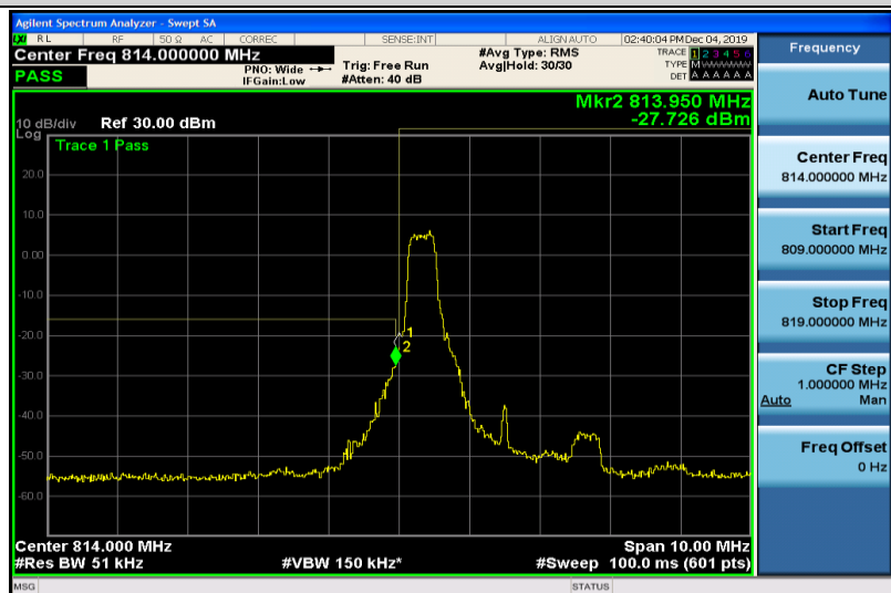
Band26-3MHz-16QAM-26705-15RB#0
