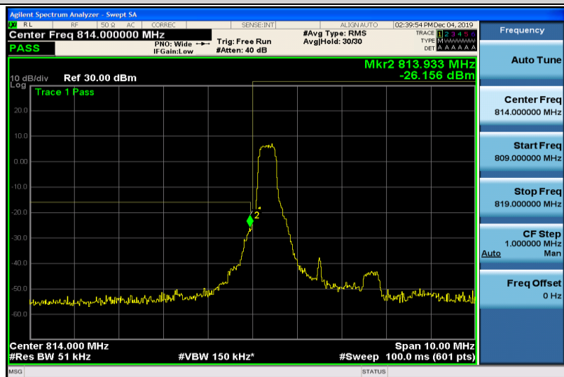
Band26-3MHz-QPSK-26705-15RB#0
