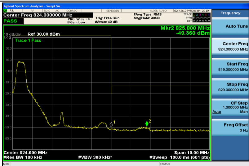
Band26-5MHz-QPSK-26765-1RB#25
