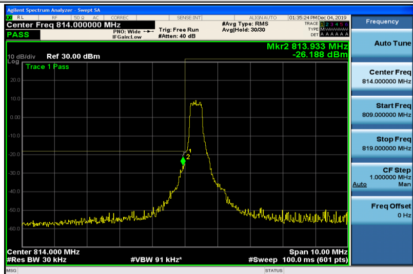
Band26-1.4MHz-16QAM-26697-1RB#5
