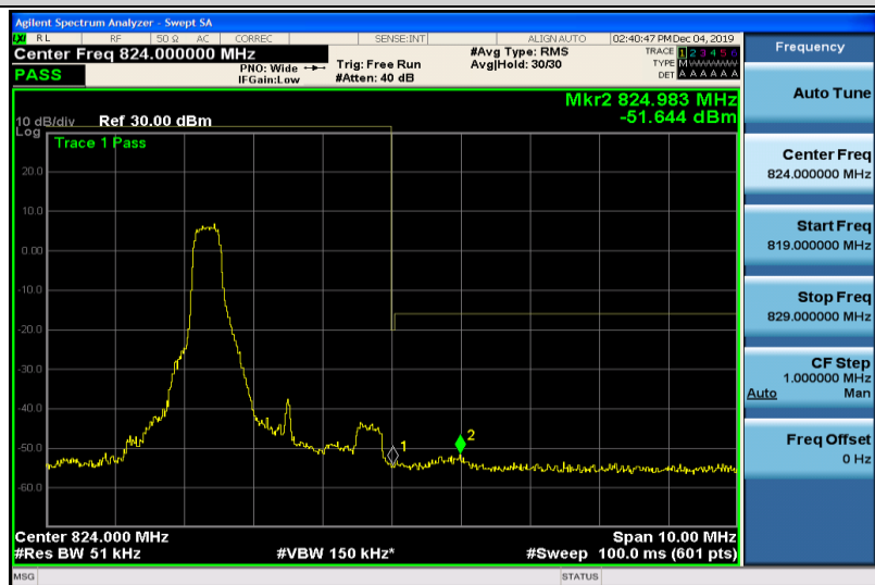
Band26-3MHz-QPSK-26775-15RB#0
