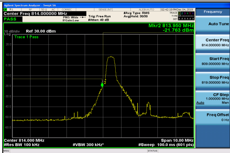
Band26-5MHz-QPSK-26715-25RB#0
