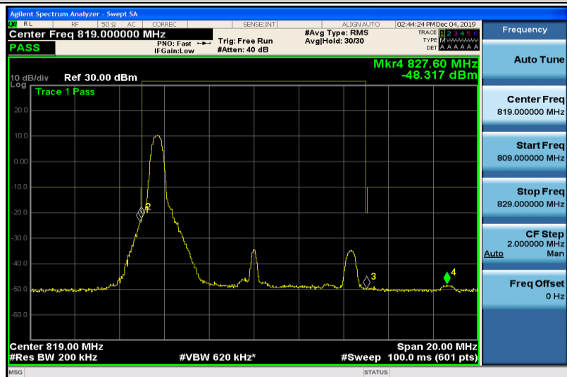
Band26-10MHz-QPSK-26740-1RB#50
