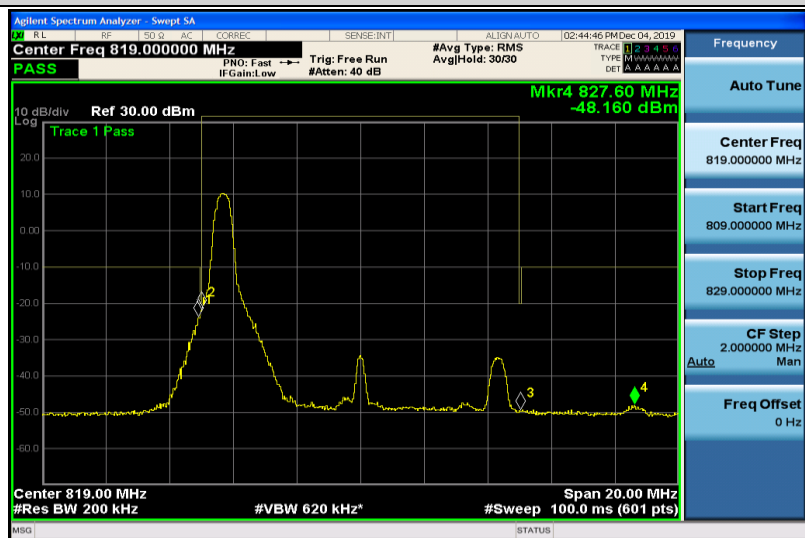
Band26-10MHz-QPSK-26740-50RB#0
