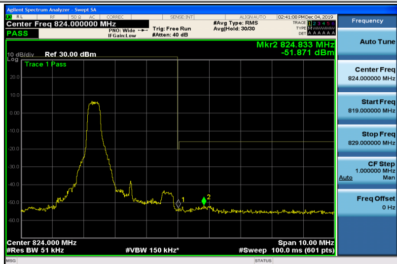
Band26-3MHz-QPSK-26775-1RB#0
