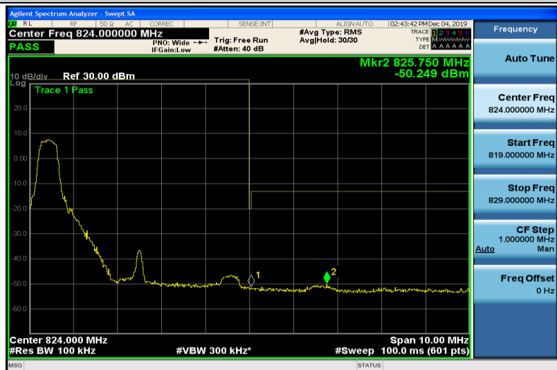
Band26-5MHz-16QAM-26765-1RB#0
