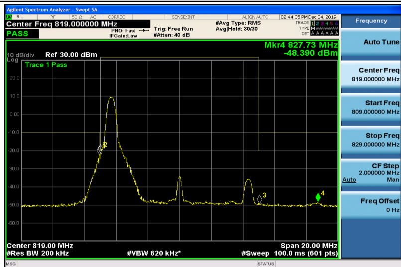
Band26-10MHz-16QAM-26740-1RB#50
