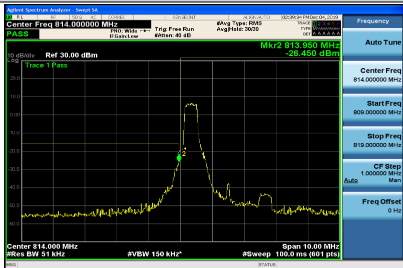
Band26-3MHz-QPSK-26705-1RB#15
