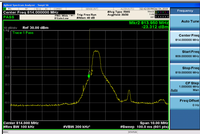
Band26-5MHz-16QAM-26715-25RB#0
