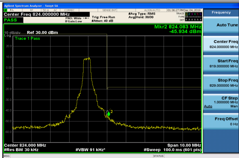
Band26-1.4MHz-QPSK-26783-1RB#5
