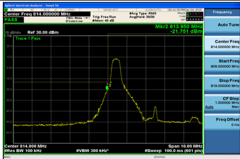
Band26-5MHz-QPSK-26715-1RB#25
