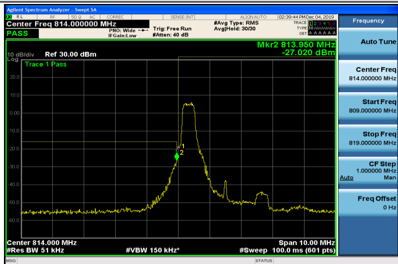
Band26-3MHz-16QAM-26705-1RB#15
