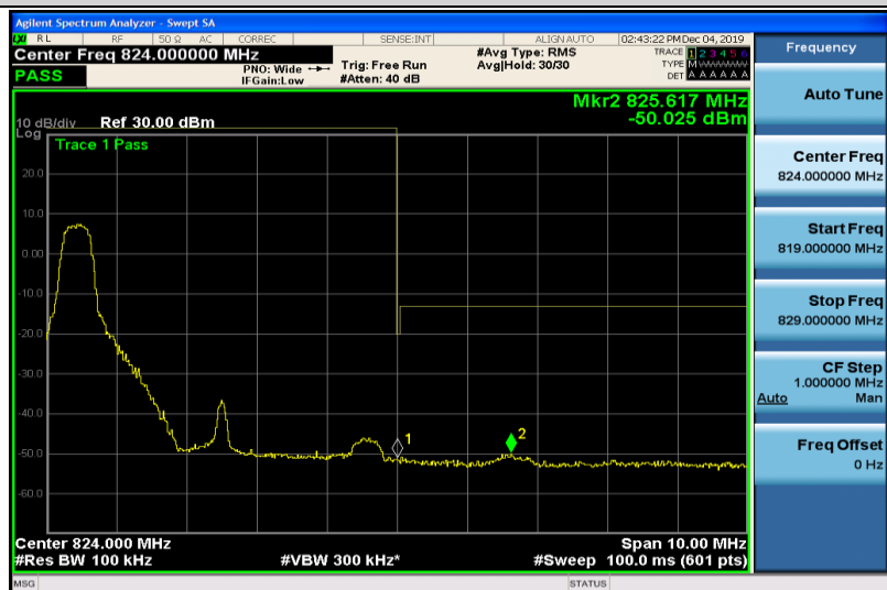
Band26-5MHz-16QAM-26765-25RB#0
