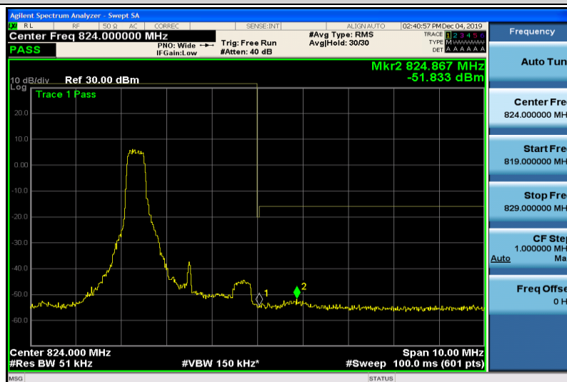
Band26-3MHz-16QAM-26775-1RB#15
