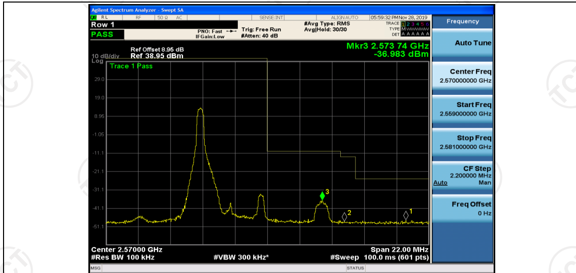
(Channel Bandwidth: 5 MHz)_HCH_QPSK_1RB#24
