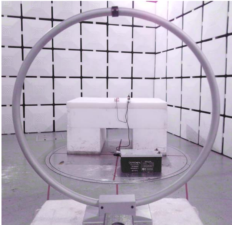
Photo of Setup for Radiated Emission (Below 1 GHz)
