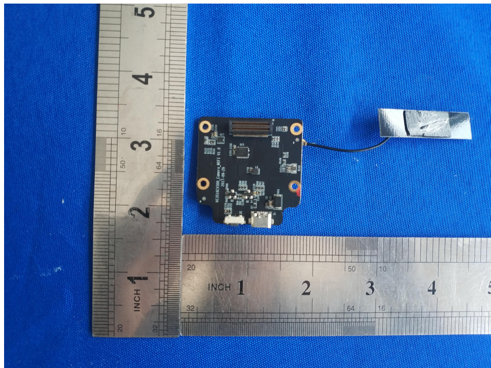
PCB antenna
