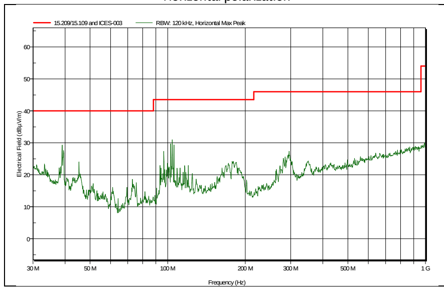
Horizontal polarization
