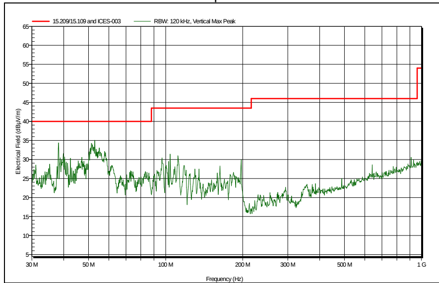
Vertical polarization
