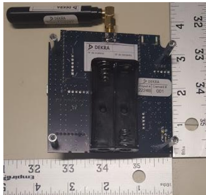
Figure B2: Rear view DUT
