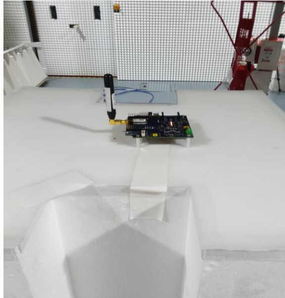
Figure B3. Radiated Setup
