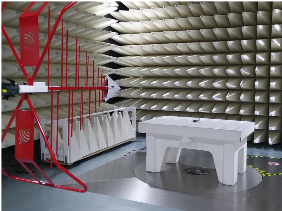
Figure B4. Radiated Emission Setup
