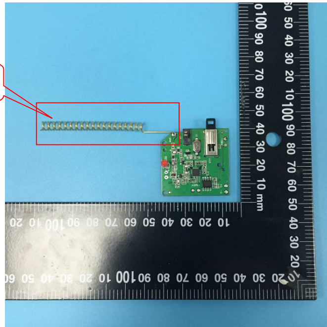
FRS Antenna
