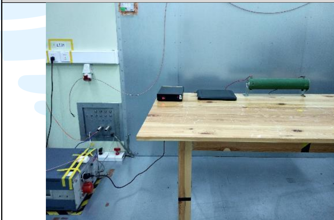
Conducted Emission Test Setu
