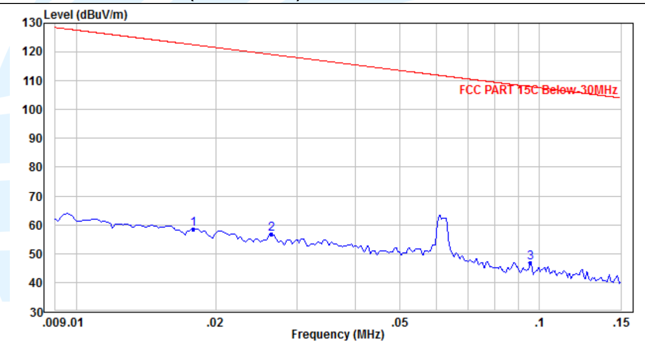
Radiated Emission Test Data (9 KHz ~ 150 KHz):
