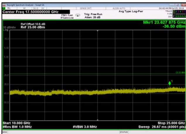
Conducted Emission: 8DPSK,2441,3DH5 ,10000MHz~25000MHz
