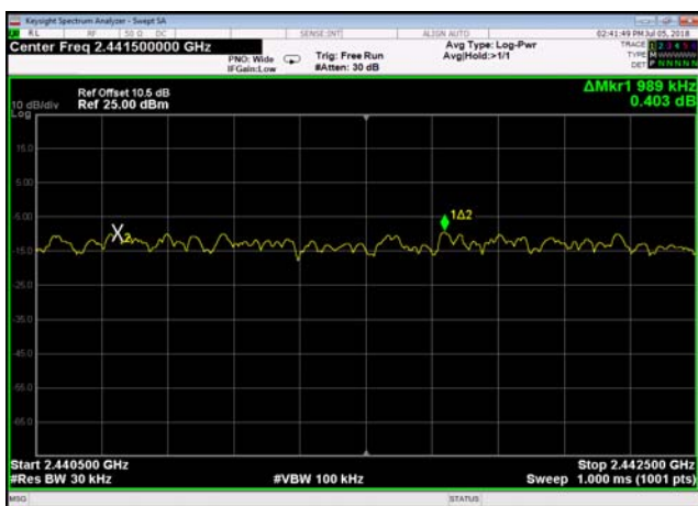
Carrier Frequency Separation: pi/4DQPSK ,Hopping2DH52440.5~2442.5
