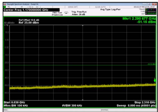
Conducted Emission: 8DPSK,2480,3DH5 ,30MHz~2310MHz
