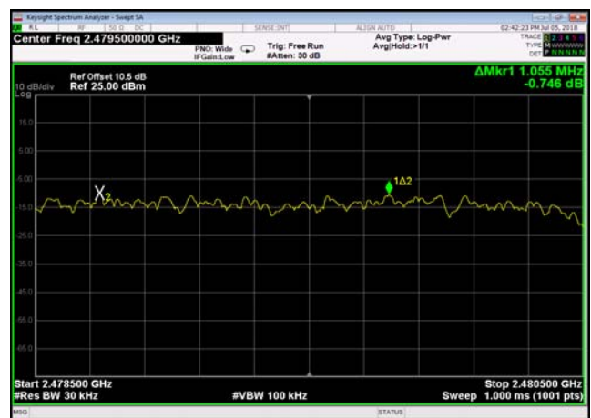
Carrier Frequency Separation: pi/4DQPSK ,Hopping2DH52478.5~2480.5
