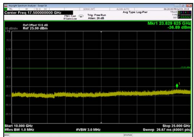
Conducted Emission: 8DPSK,2480,3DH5 ,10000MHz~25000MHz
