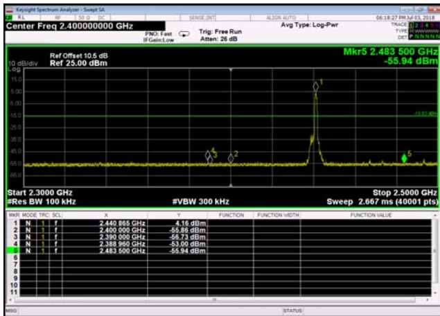
Conducted Emission: 8DPSK,2441,3DH5 ,Reference Level
