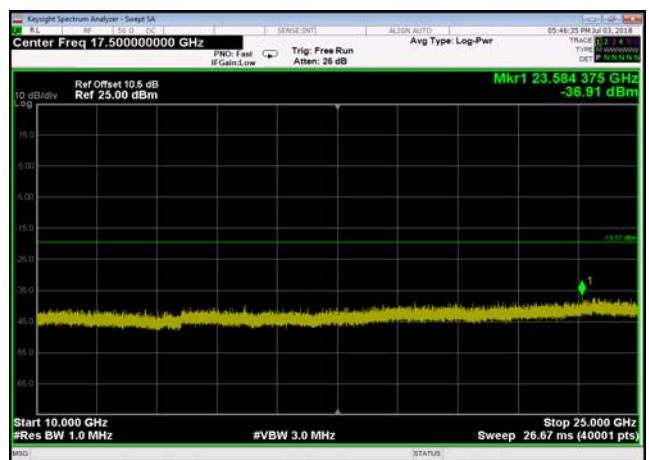
Conducted Emission: 8DPSK,2402,3DH5 ,10000MHz~25000MHz
