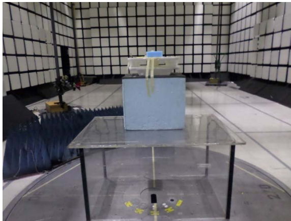
Figure 5: Radiated Emissions Limits, 1GHz-10GHz - Setup Rear View
