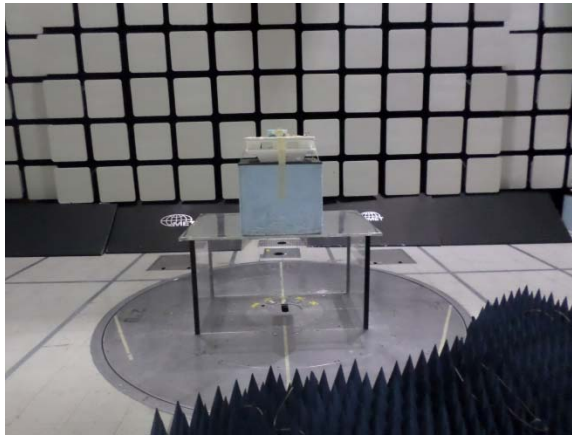
Figure 4: Radiated Emissions Limits, 1GHz-10GHz - Setup Front View
