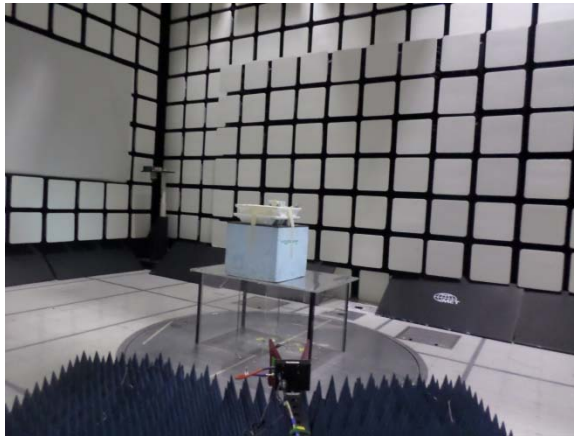
Figure 6: Radiated Emissions Limits, 1GHz-10GHz - Setup Antenna View
