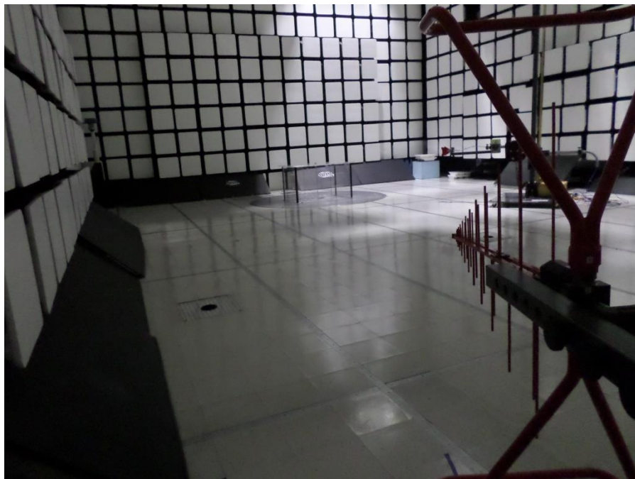
Photograph 4. Radiated Spurious Emissions, <1 GHz, Antenna
