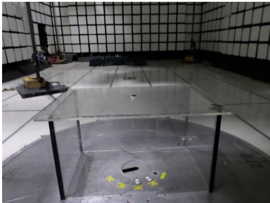
Photograph 6. Radiated Spurious Emissions, <1 GHz, Rear
