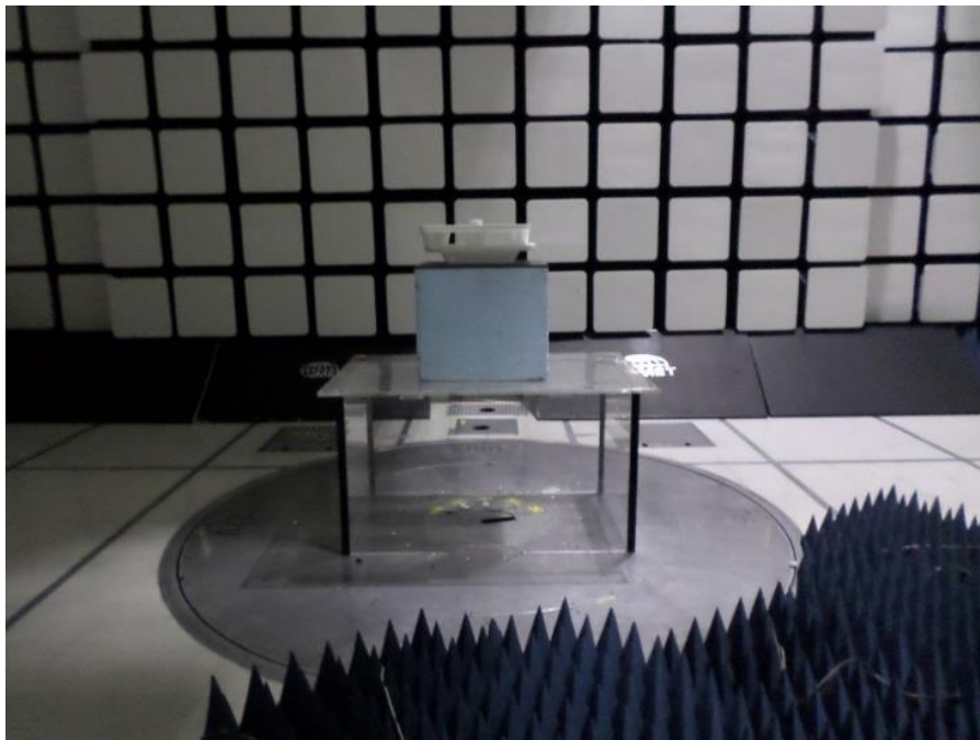
Photograph 2. Radiated Spurious Emissions, >1 GHz, Front
