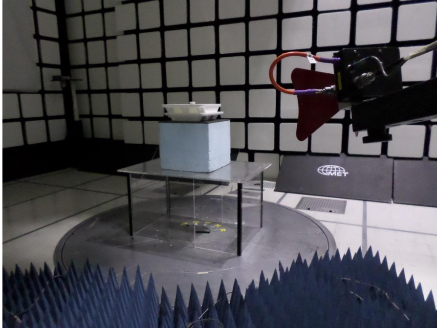
Photograph 1. Radiated Spurious Emissions, >1 GHz, Antenna
