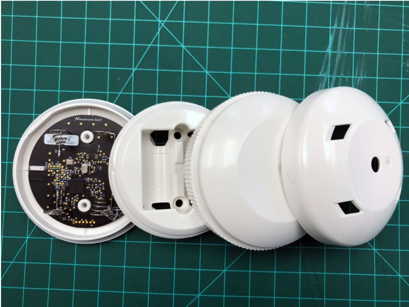
Gen3 Node - All Parts
