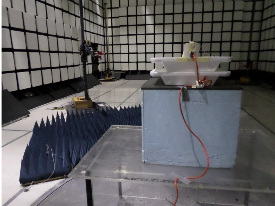
Photograph 5. Radiated Spurious Emissions, >1 GHz, Rear
