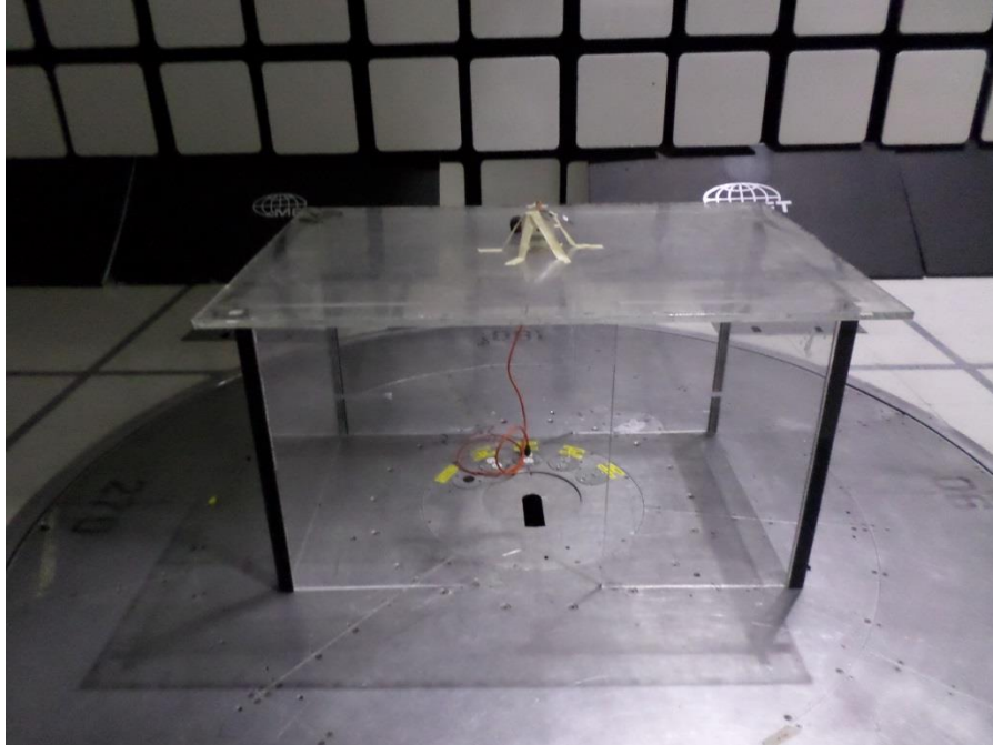
Photograph 7. Radiated Spurious Emissions, <1 GHz, Front
