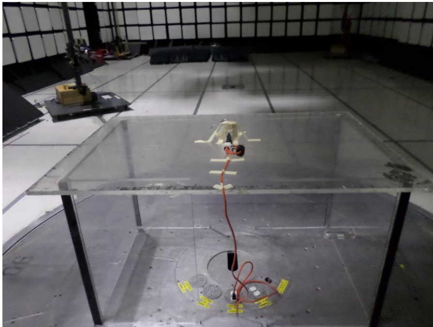
Photograph 8. Radiated Spurious Emissions, <1 GHz, Rear
