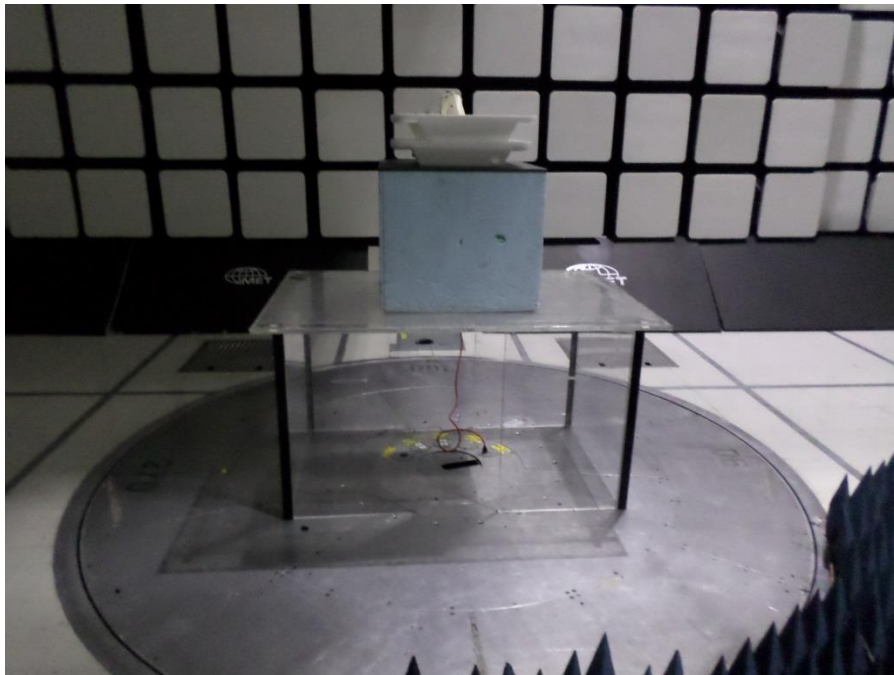
Photograph 4. Radiated Spurious Emissions, >1 GHz, Front
