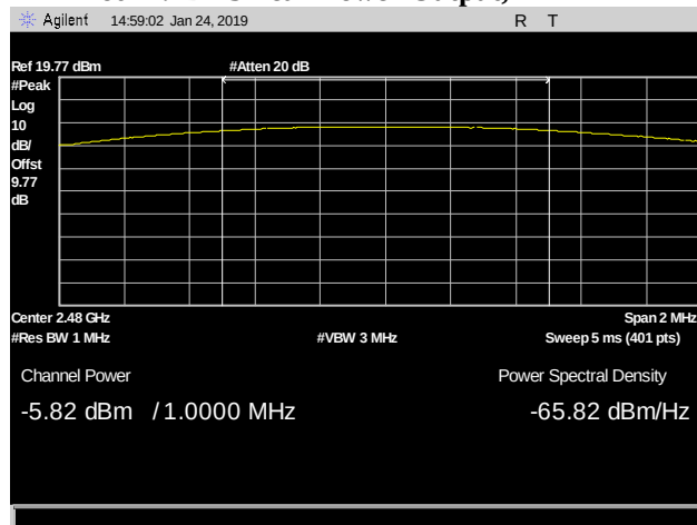
Plot 28. DH3 Peak Power Output, 2480 MHz
