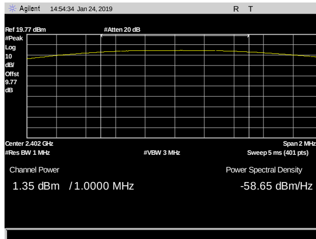
Plot 26. DH3 Peak Power Output, 2402 MHz
