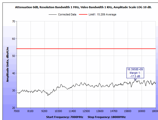
Plot 58. Radiated Spurious Emissions, 2480 MHz, 7 – 18 GHz, H, Average
