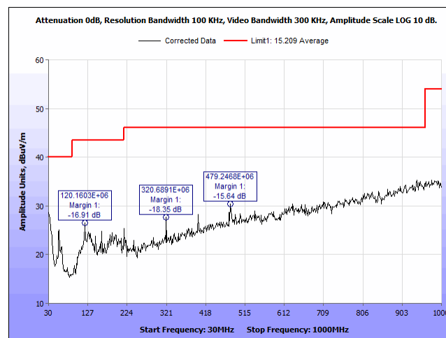
Plot 52. Radiated Spurious Emissions, 2480 MHz, 30 MHz – 1 GHz, H
